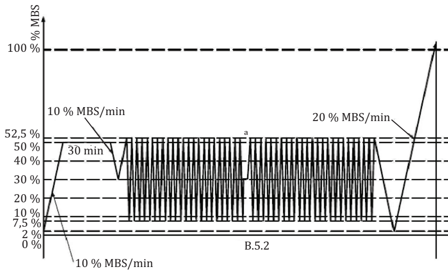
Figure F.6 — Linear density test sequence, B.4
