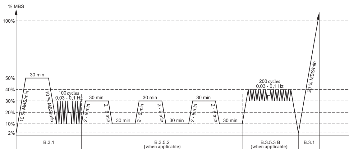
Figure F.4 — Quasi-static stiffness, dynamic stiffness and breaking test sequence, B.3 , sample b
