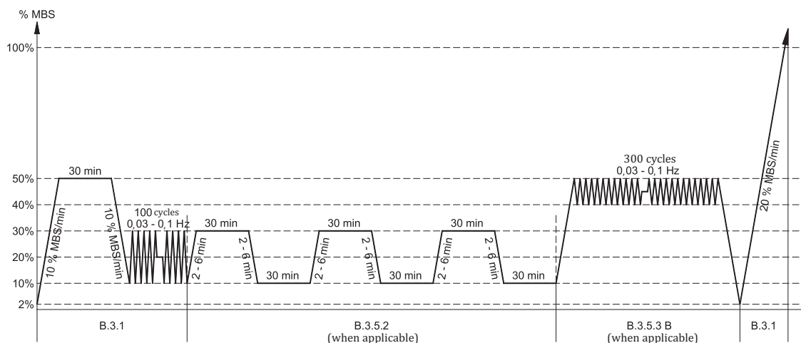
Figure F.5 — Quasi-static stiffness, dynamic stiffness and breaking test sequence, B.3 , sample c
