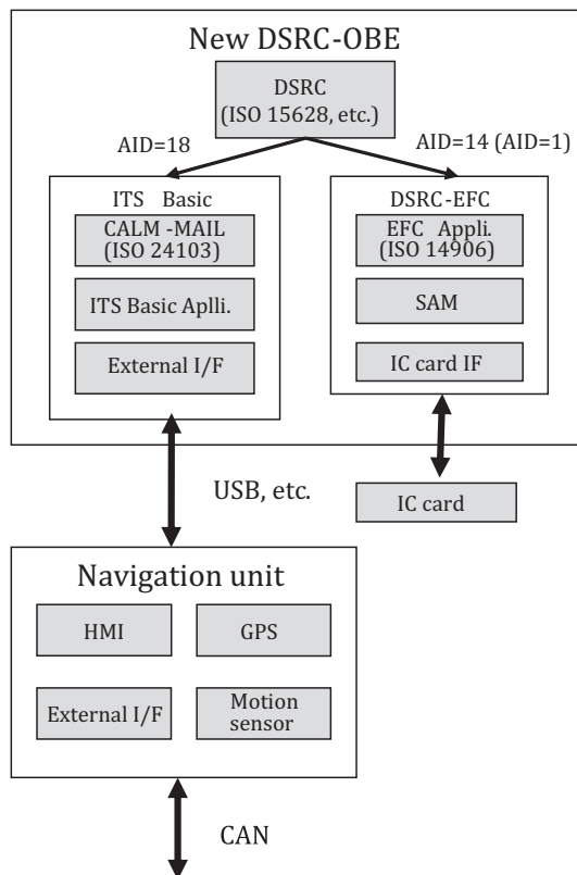
Figure E.2 — Internal diagram of new DSRC-OBE
