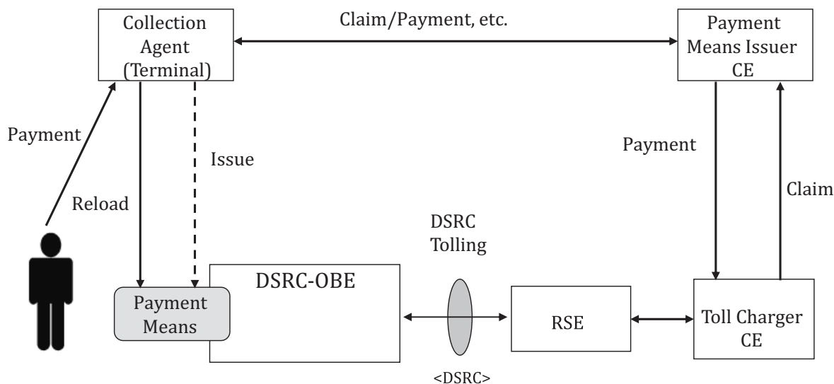
Figure 6 — Basic DSRC tolling
