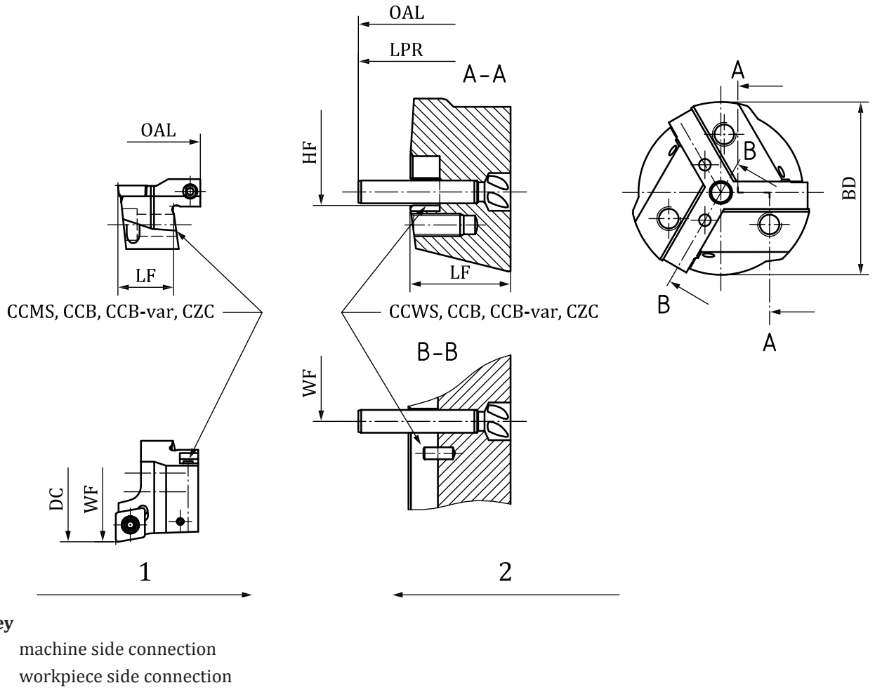
Figure E.11 — Variant 01 of CCB Coromant CoroBore
