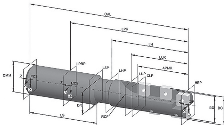
Figure 71 — Assembled multi-rows, centre cutting end mill
