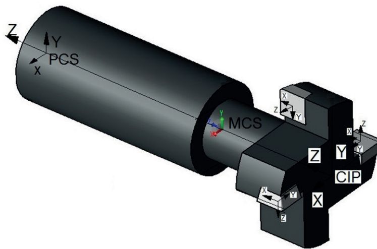
Figure 103 — Example of a data exchange model of a T-slotting end mill
