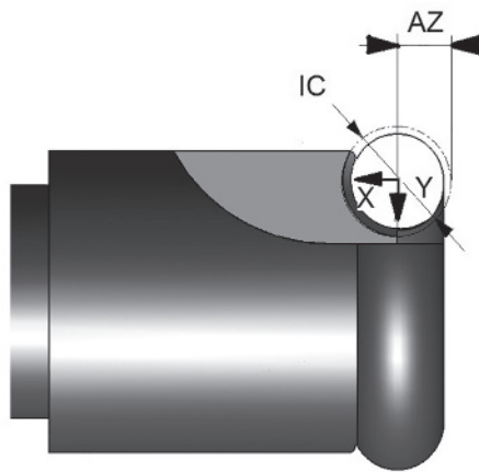
Figure 41 — Pocket seat
