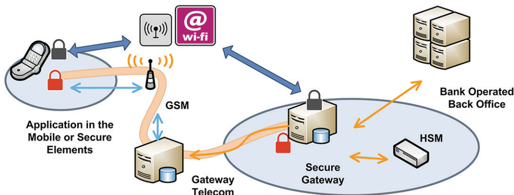
Figure D.1 — Typical architecture for the provision of remote MFSs
