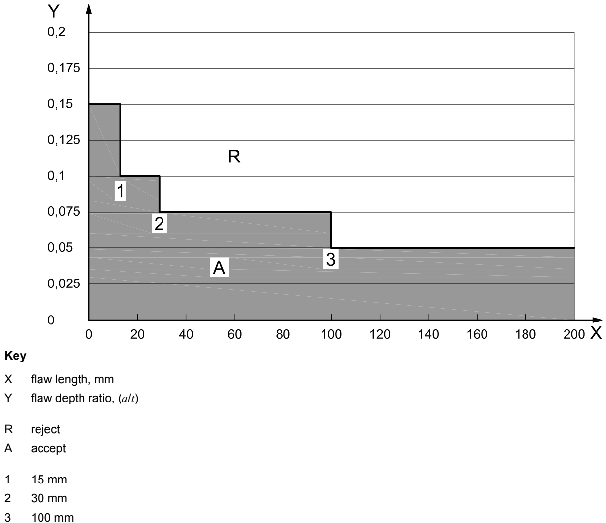
Figure 25 — Accept/reject master curve for all aluminium-alloy cylinders
