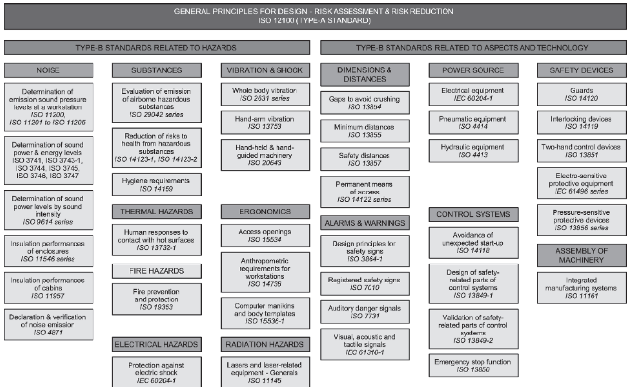
Figure 5 — Overview on type-B standards grouped by hazard category and aspects and technology (not all inclusive)
