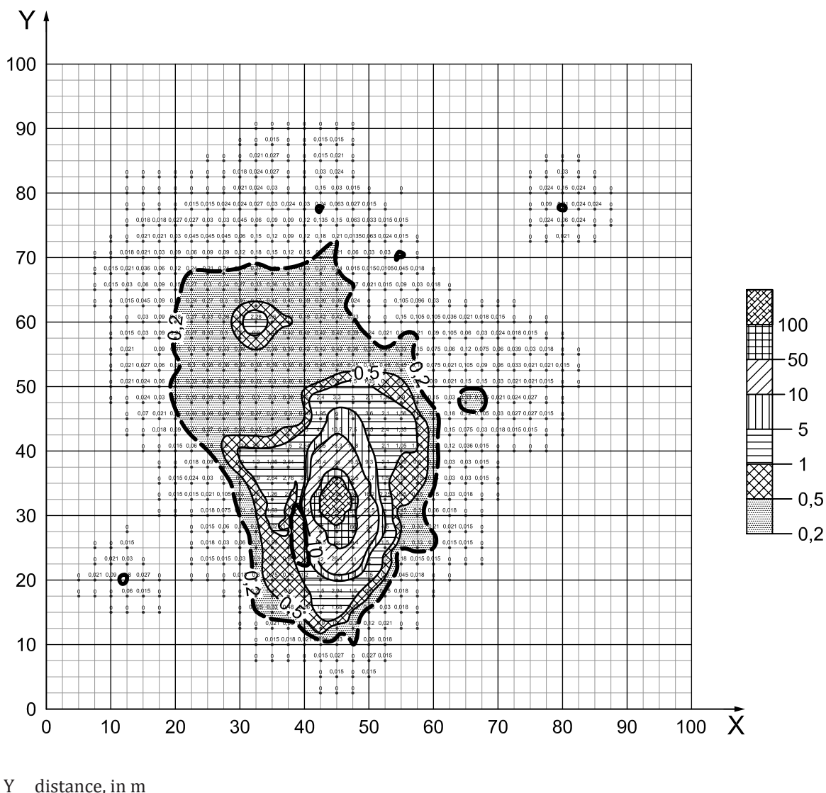
Figure C.5 — Cr(VI) distributions mapped through test-kit screening work in the clayey soil ground having a Cr(VI) recovery of 30 %
