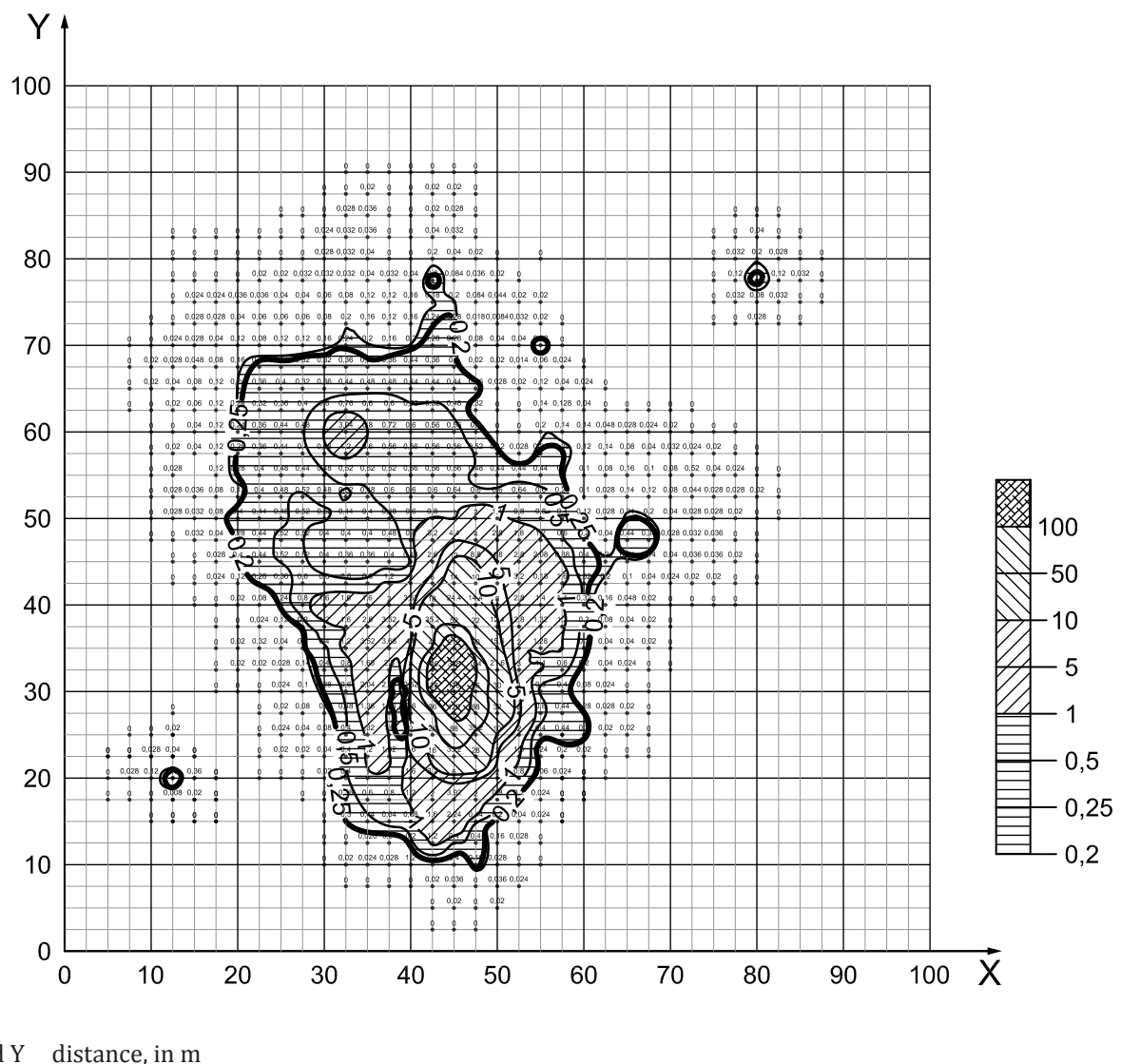
Figure C.4 — Cr(VI) distributions mapped through test-kit screening work in the common-type soil ground having a Cr(VI) recovery of 40 \%
