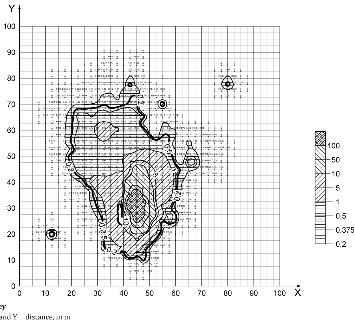
Figure C.3 — Cr(VI) distributions mapped through test-kit screening work in the sandy soil ground having a Cr(VI) recovery of 60 %
