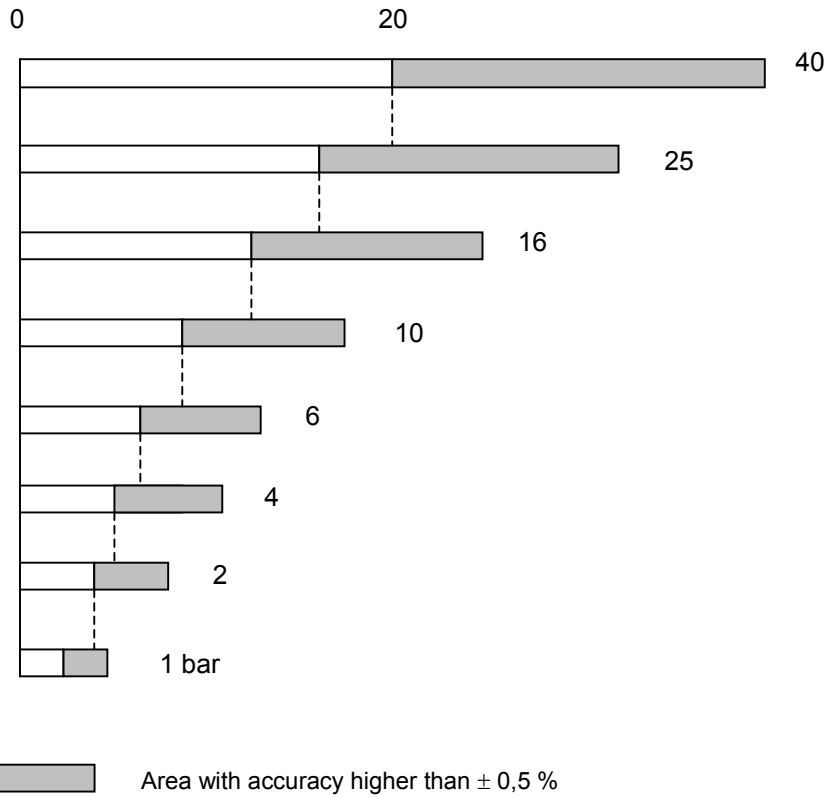
Figure 4 — Example of a range of pressure gauges for a test facility
