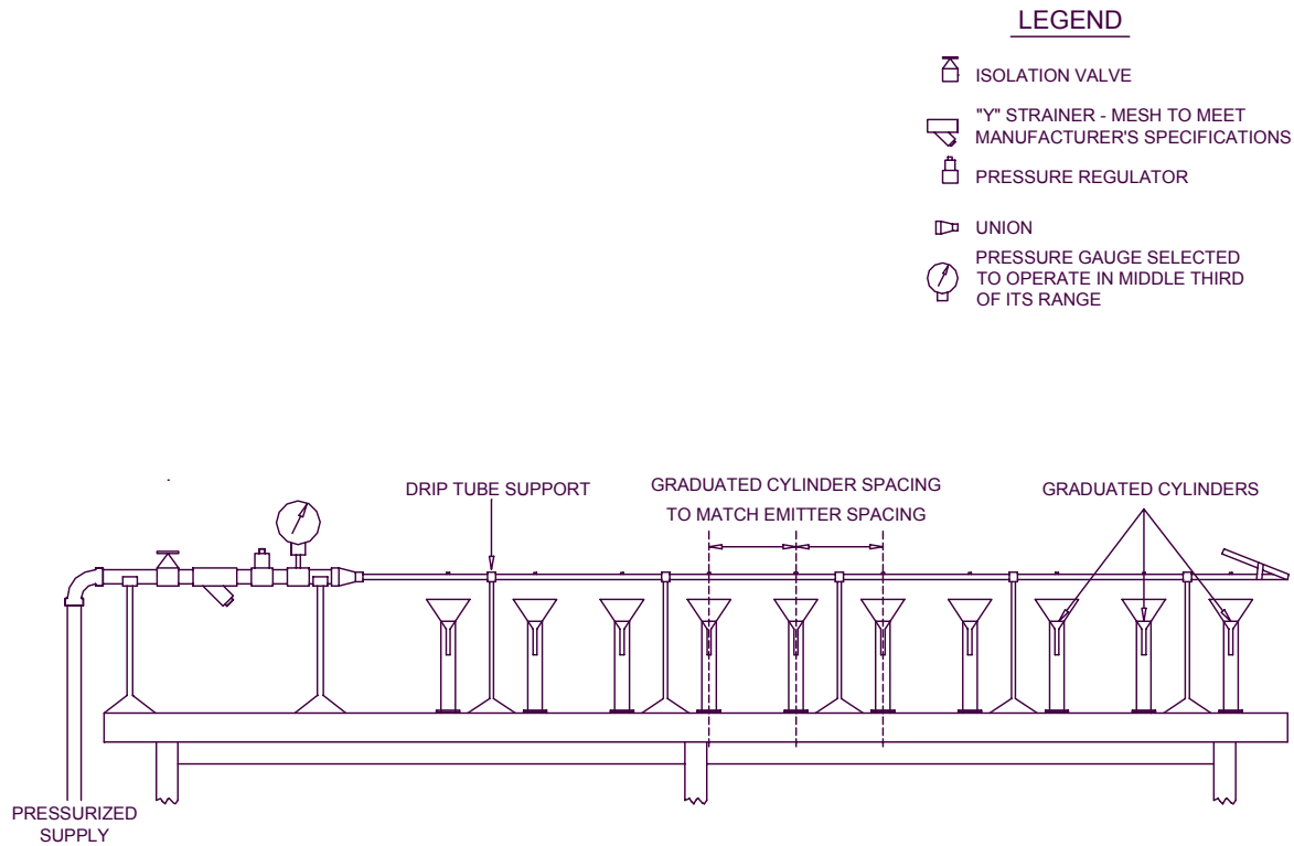
Figure 3 — Typical test bench configurations for testing emitters
