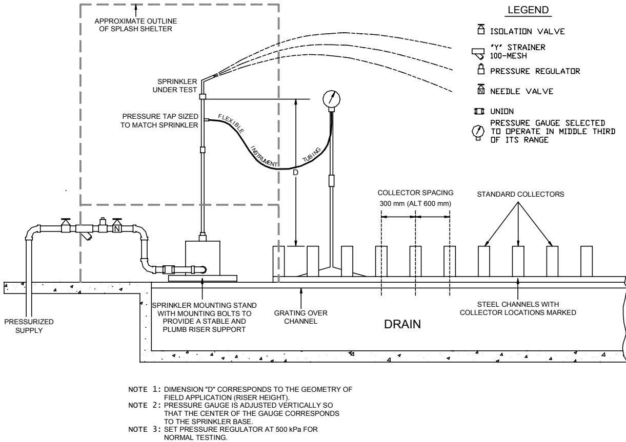
Figure 2 — Typical test bench configurations for testing sprinklers
