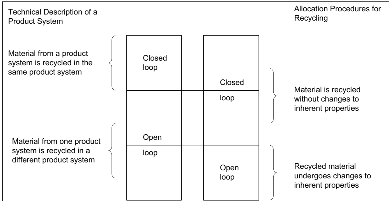
ISO 14044:2006 — Figure 2 — Distinction between a technical description of a product system and allocation procedures for recycling
