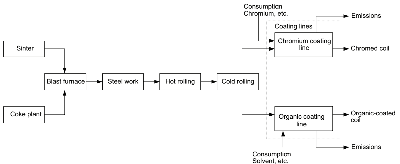
Figure 7 — System where allocation may be avoided through a more precise data collection and dividing into two different subsystems
