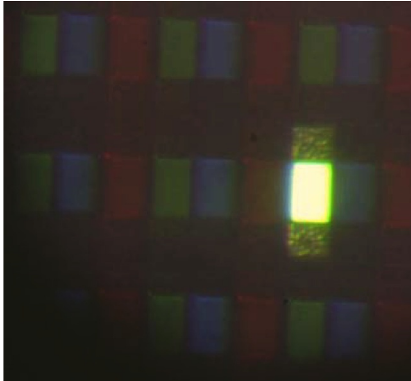
Figure 16 — Subpixel defect in a transfective LCD in dark
