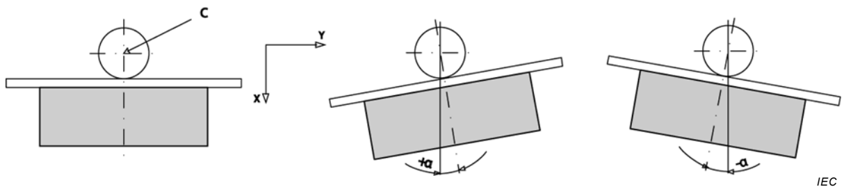
Figure 3 – Angular misalignment – side view
