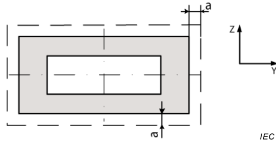
Figure 2 – Orthogonal misalignment – front view
