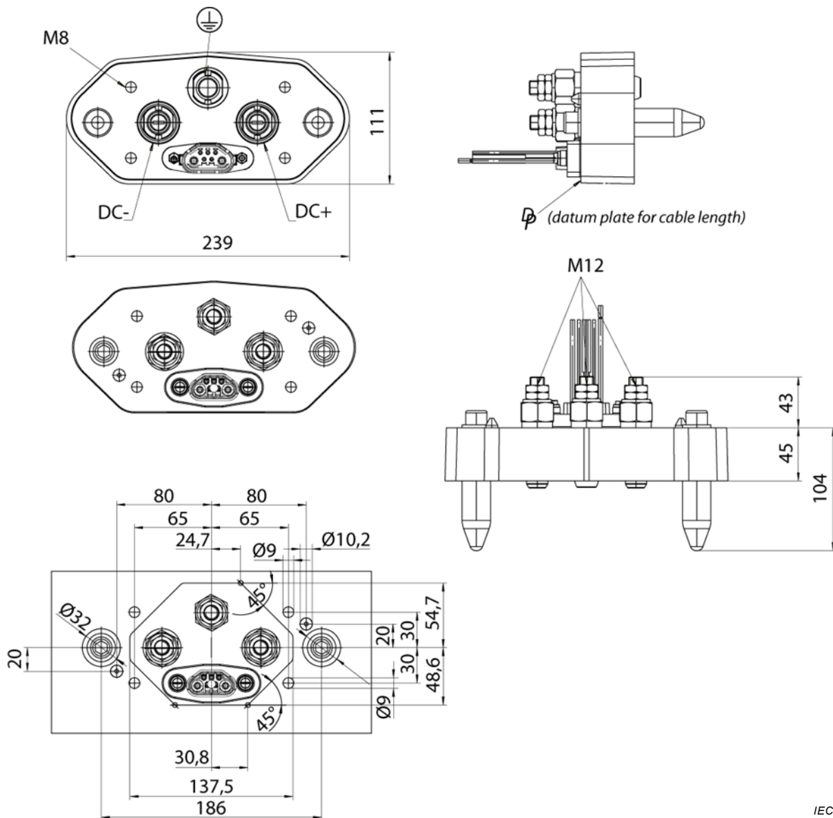
Figure C.8 – Accessory example 3 Type B
