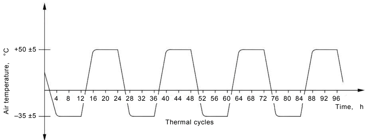
Figure 1 – Thermal cycle test
