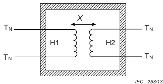
Figures D.2 c) and d) – Protection between a HAZARDOUS LIVE primary circuit and circuits which have ACCESSIBLE external TERMINALS
