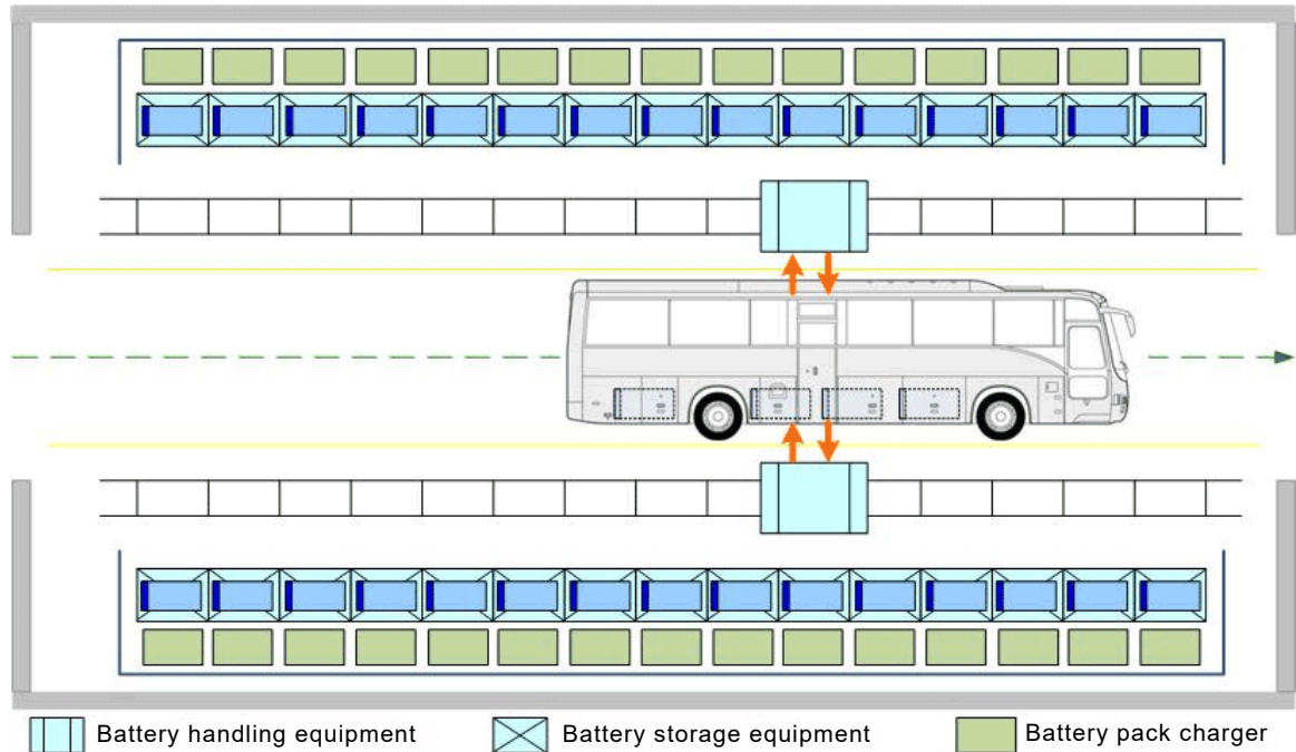
Figure B.1 – Automatic side-swapping station layout
