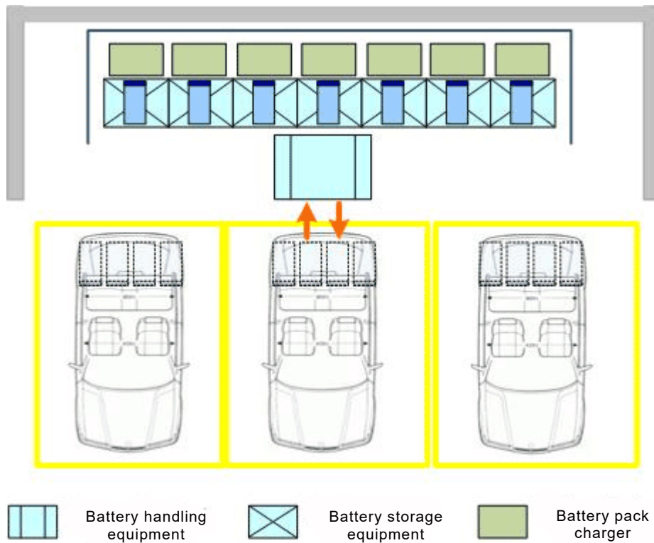
Figure B.3 – Semi-automatic rear-swapping station layout
