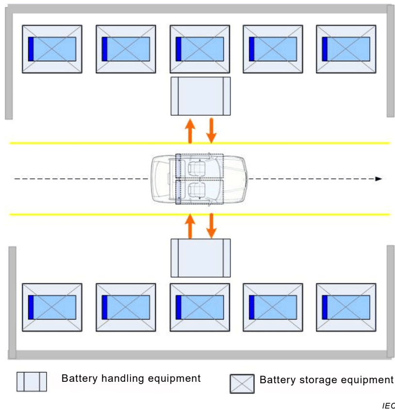
Figure B.5 – Automatic side-swapping station layout
