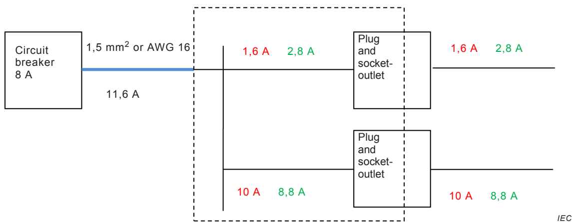
Figure 34 – Circuit diagram for testing socket-outlets and plugs according to 18.2
