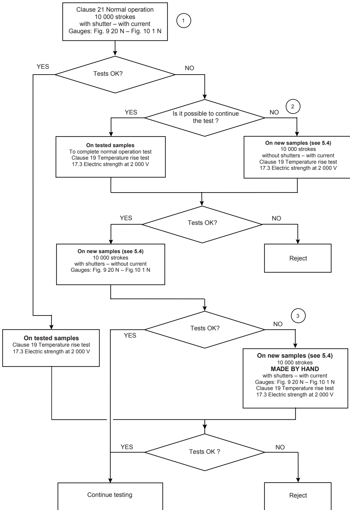
Figure 30 – Test procedures for normal operation (see Clause 21)
