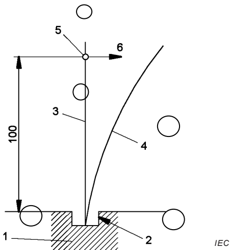
Figure 12a – Principle of the test apparatus for deflection on screwless terminals
