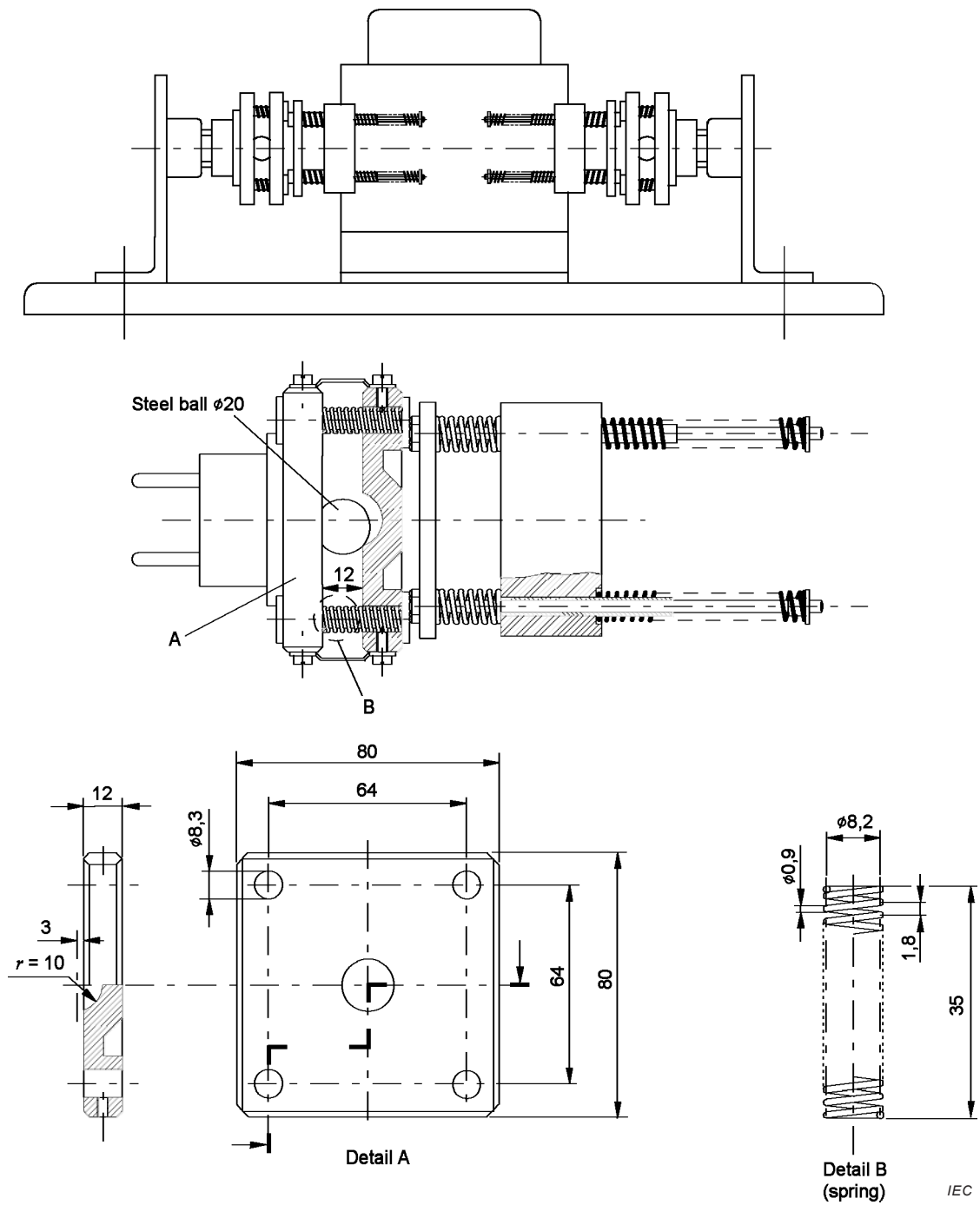
Figure 14 – Example of apparatus for breaking capacity and normal operation test
