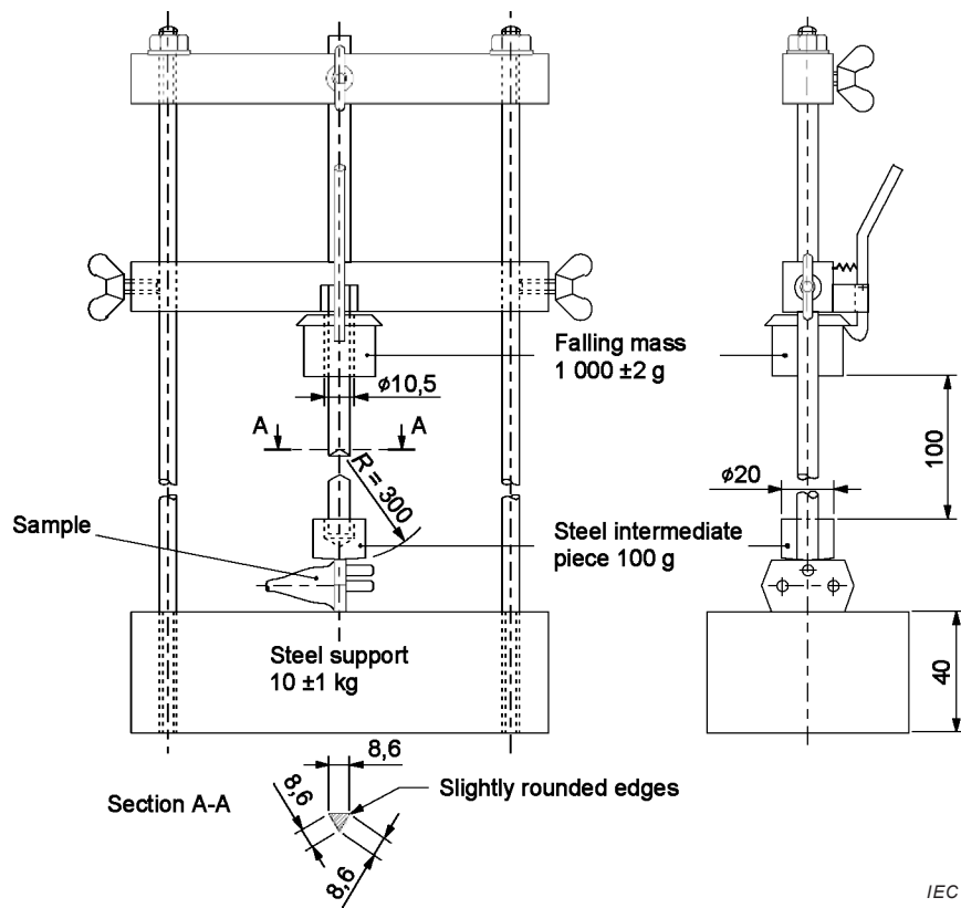
Figure 20 – Apparatus for impact test at low temperature of 24.5
