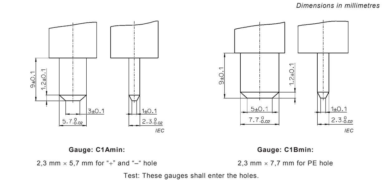
Figure D.4 – Minimum gauges for checking the dimensions of the entry holes: C1
