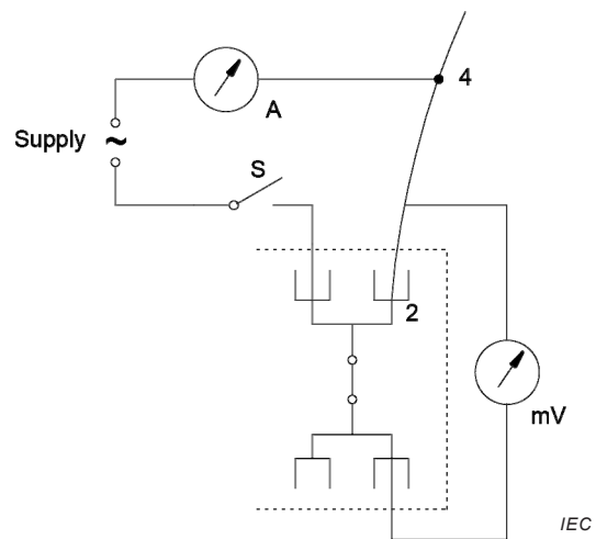
Figure 12b – Example of test arrangement to measure the voltage drop during deflection test on screwless terminals
