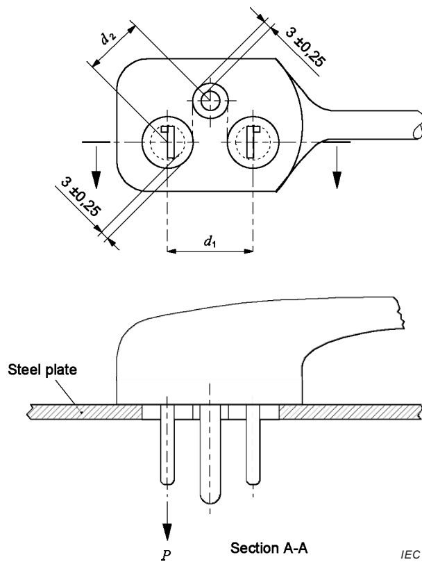
Figure 21 – Example of test arrangement to verify the fixation of pins in the body of the plug
