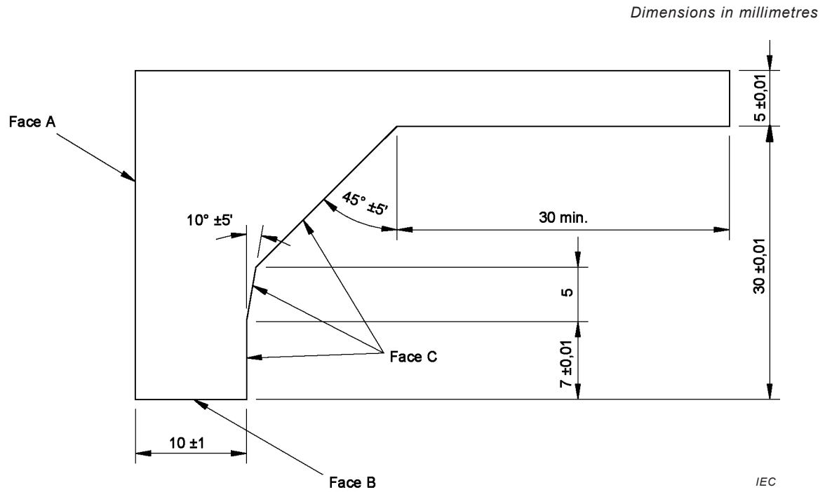
Figure 23 – Gauge (thickness about 2 mm) for the verification of the outline of covers or cover-plates
