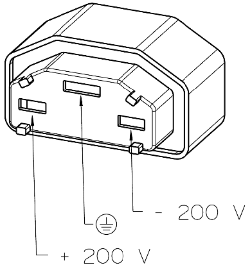
Figure D.3 – Standard sheet 3: positioning of the “+” and “-” pins/socket-contacts
