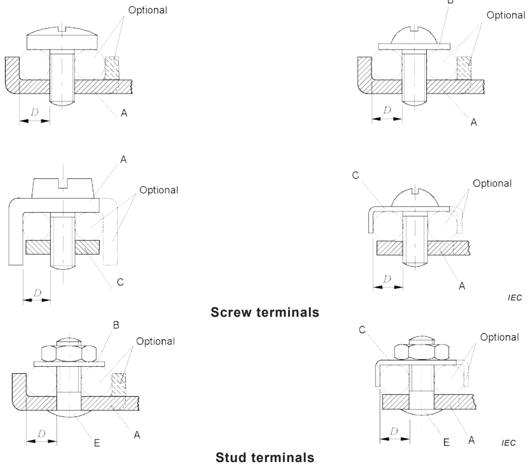
Figure 3a – Screw/stud not requiring washer or clamping plate
