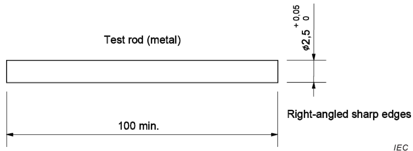
Figure 26 – Gauge for verification of grooves, holes and reverse tapers
