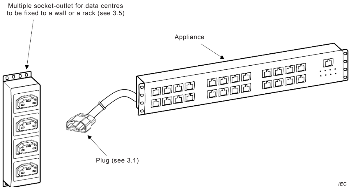
Figure 1b – Diagram showing various accessories and their use
