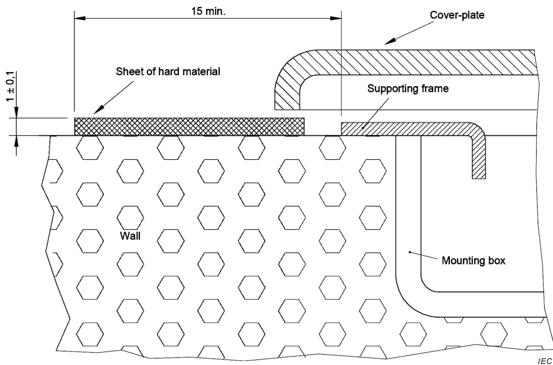
Figure 22 – Arrangement for test on covers or cover-plates
