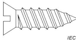
Figure 6 – Example of thread-forming screw
