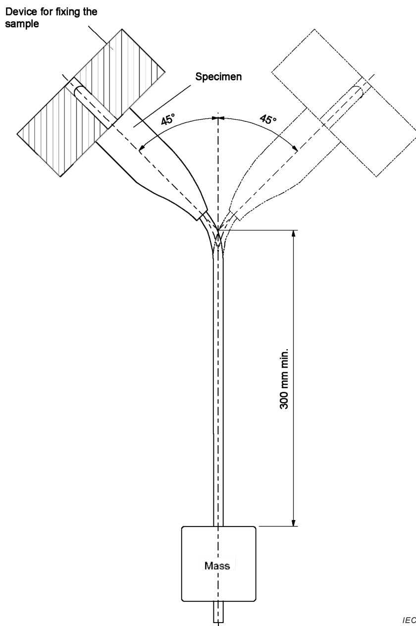
Figure 18 – Apparatus for flexing test
