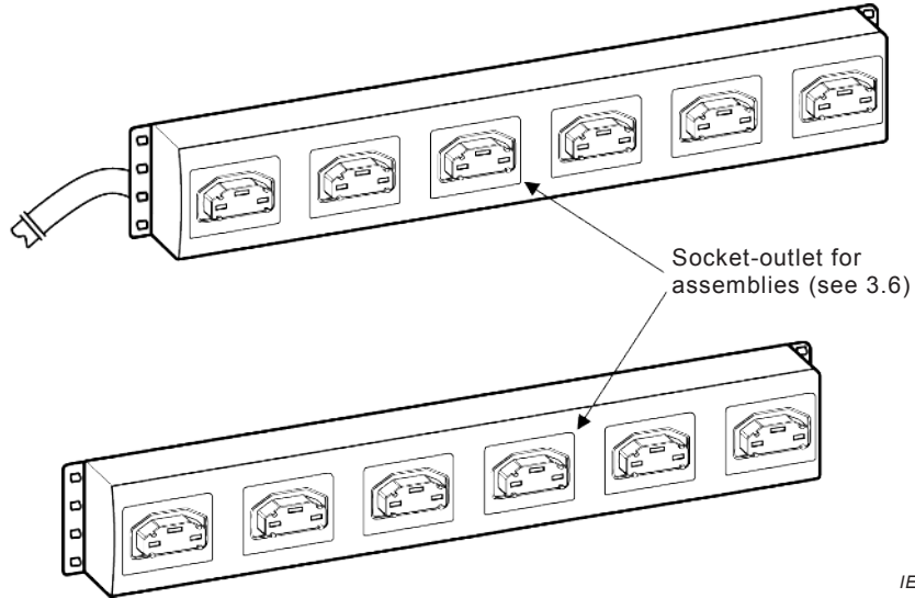
Figure 1d – Multiple socket-outlet for data centres to be fixed to a wall or a rack
