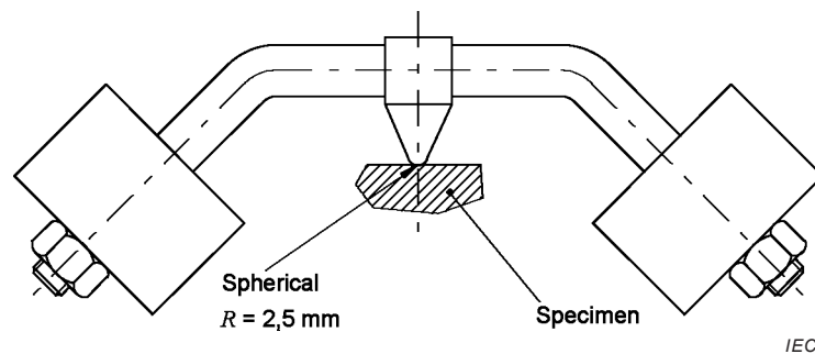
Figure 28 – Ball pressure test apparatus
