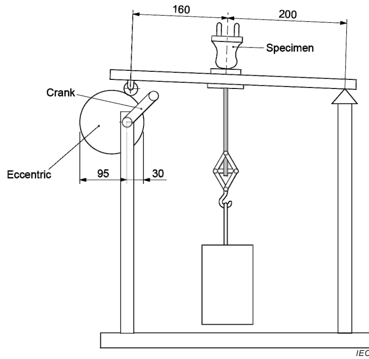
Figure 17 – Apparatus for testing cord retention
