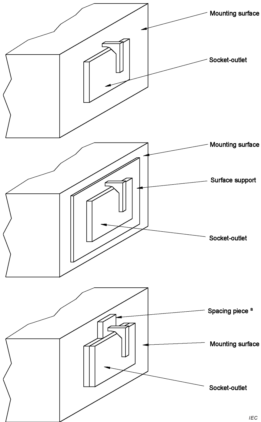
Figure 24 – Examples of application of the gauge of Figure 23 on covers fixed without screws on a mounting surface or supporting surface
