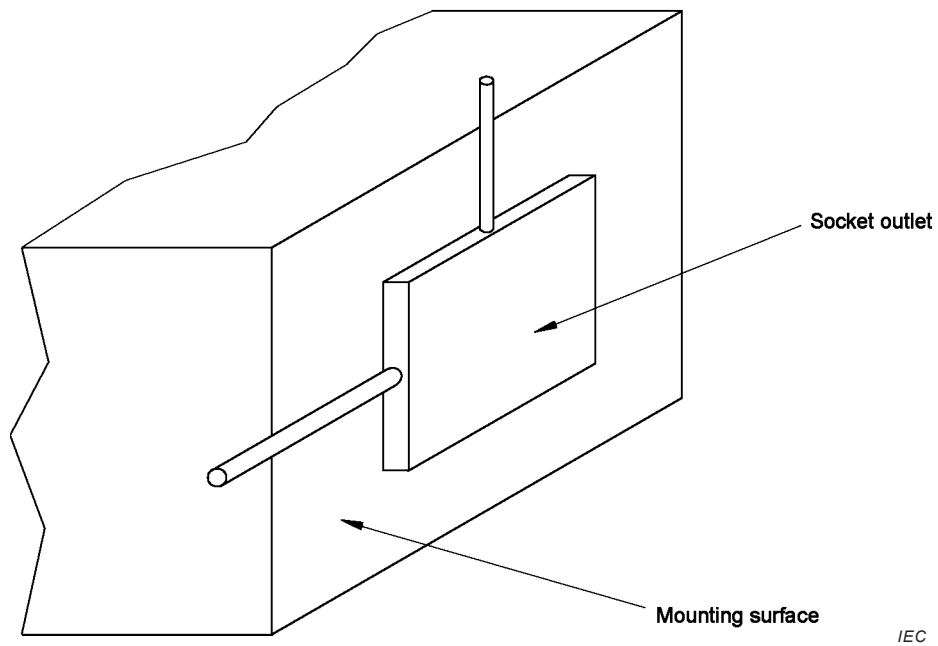
Figure 27 – Sketch showing the direction of application of the gauge of Figure 26
