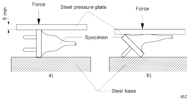
Figure 8 – Arrangement for compression test of 10.2 and 24.6
