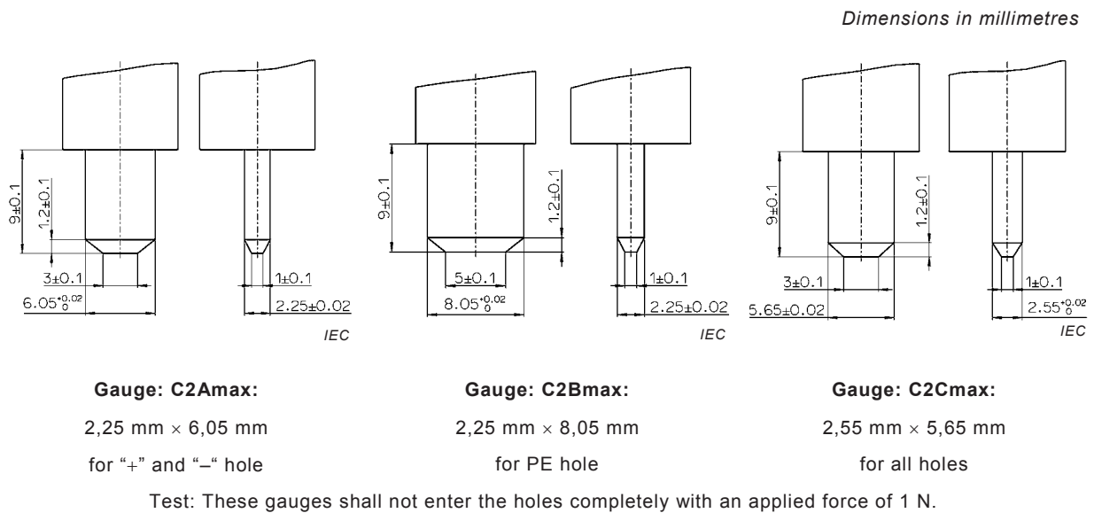
Figure D.5 – Maximum gauges for checking the dimensions of the entry holes: C2
