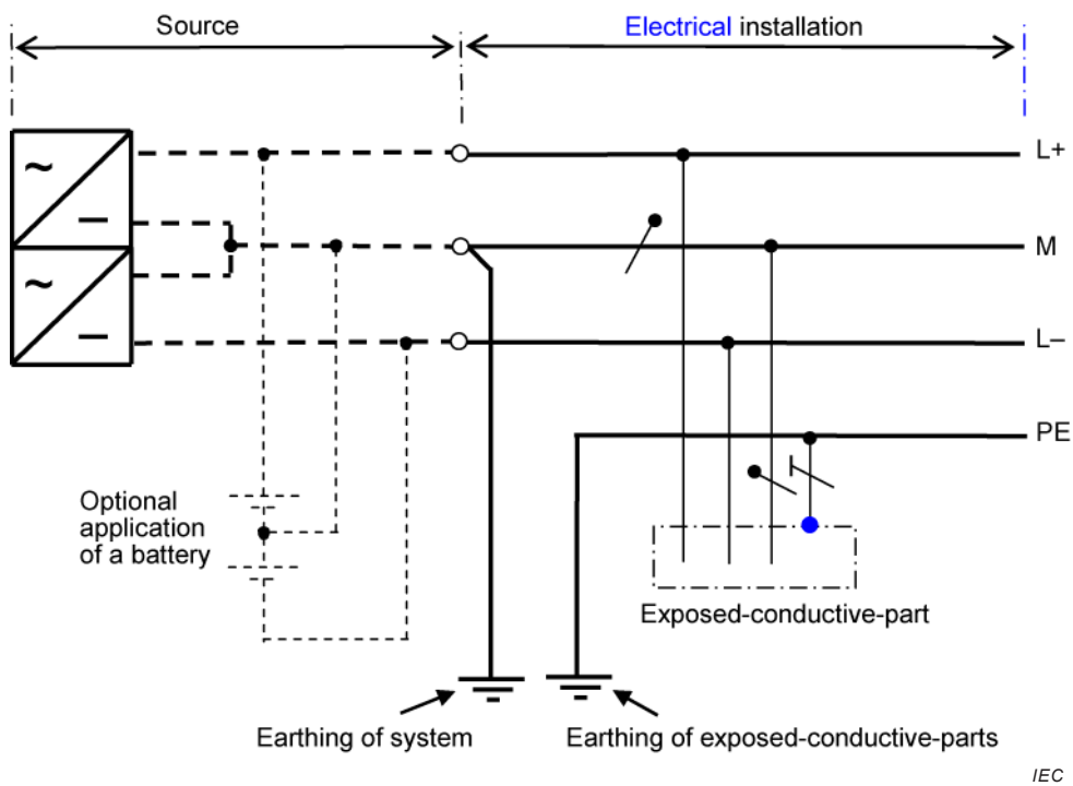
Figure B.16 – TT d.c. system
