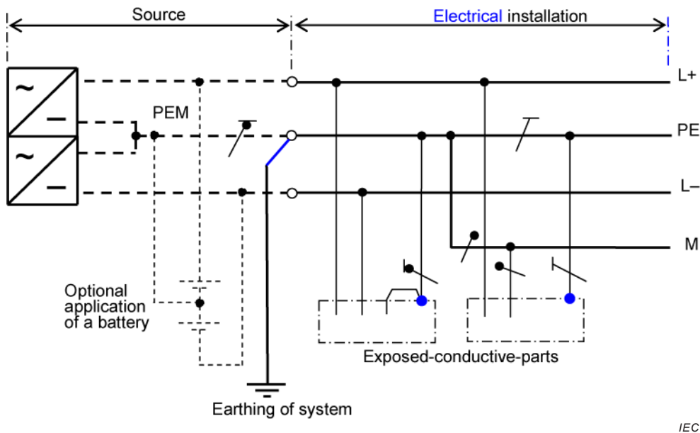
Figure B.15 – TN-C-S d.c. system
