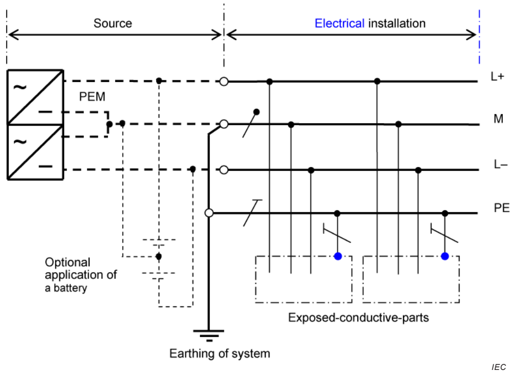
Figure B.13 – TN-S d.c. system
