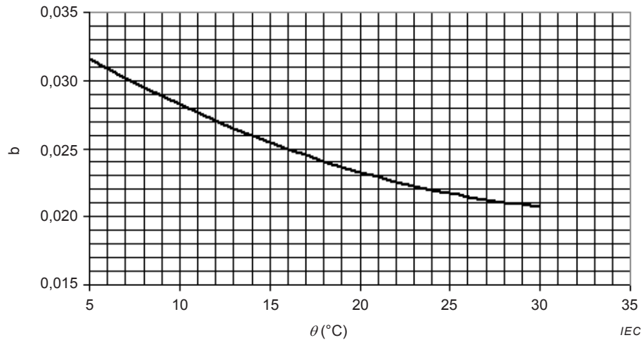
Figure 3 – Value of factor b versus solution temperature \theta
