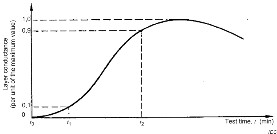
Figure C.1 – Determination of layer conductance and evaluation of its rise time T_c = t_2 - t_1
