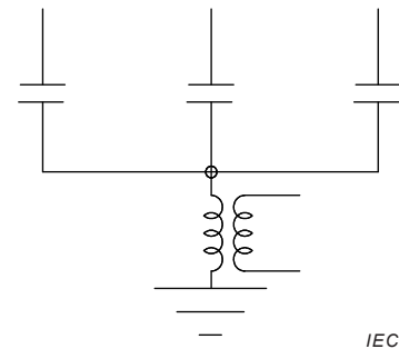
Figure 4 – Star connection with voltage transformer between neutral and ground
