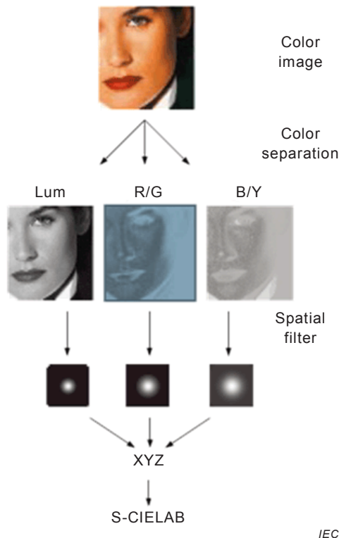
Figure A.1 – Flowchart of S-CIELAB calculation
