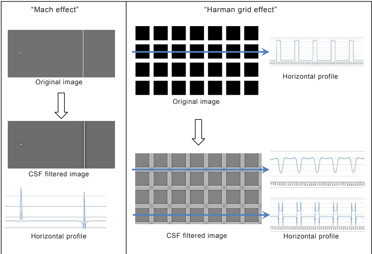
Figure A.3 – Examples of the convolution of a two-dimensional CSF filter for illusion
