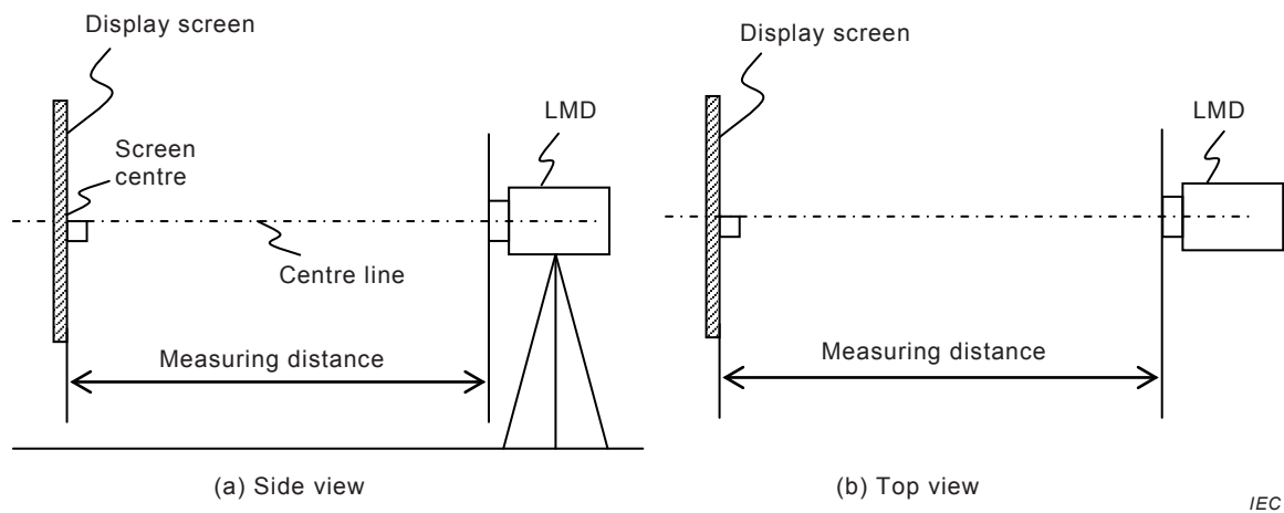
Figure 1 – Measuring layout
