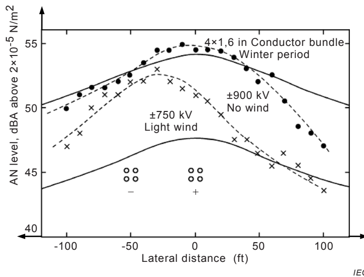
Bipolar HVDC-line equipped with 4 cm × 4,1 cm conductor bundles energized with ±750 kV and ±900 kV [32]
