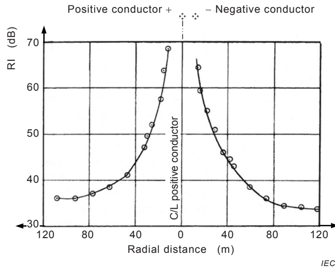
Figure B.2 – Typical RI lateral profile at ±600kV, 4 × 30,5 mm conductor, 11,2 m pole spacing, 15,2 m average height [12]
