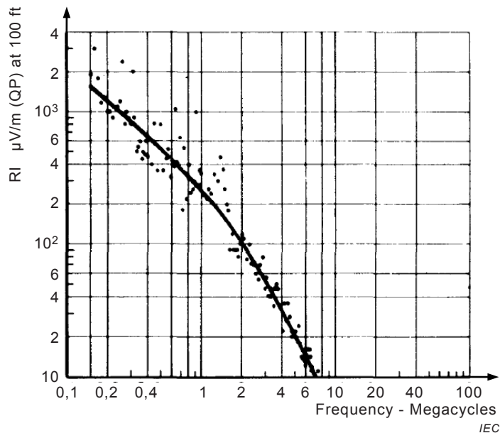
Figure B.10 – RI vs. frequency at ±400 kV [121]
