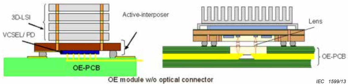
Figure 9 – Classification of optical modules on boards
