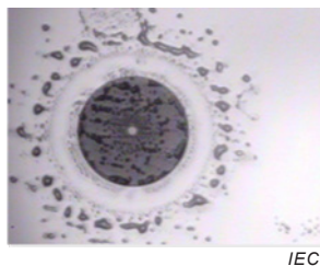
c) Plug A after mating
