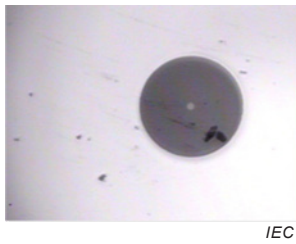
a) Clean plug wiped on a T-shirt
