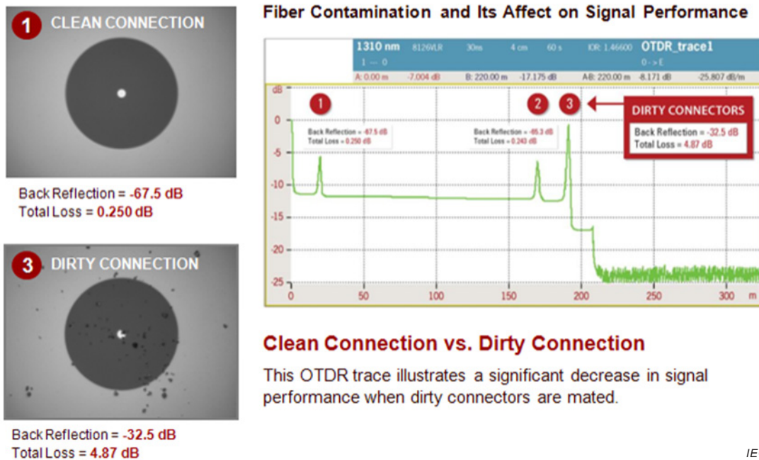
Figure B.4 – Signal degradation due to contamination
