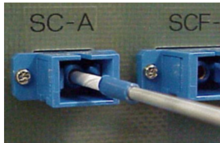
Figure 8 – Cleaning ports using a stick type cleaner
