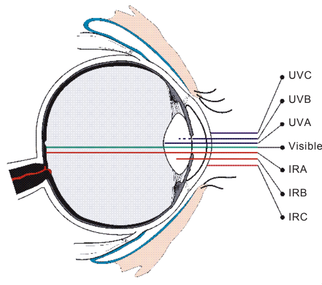
Figure A.2 – Penetration of different wavelengths through the eye
