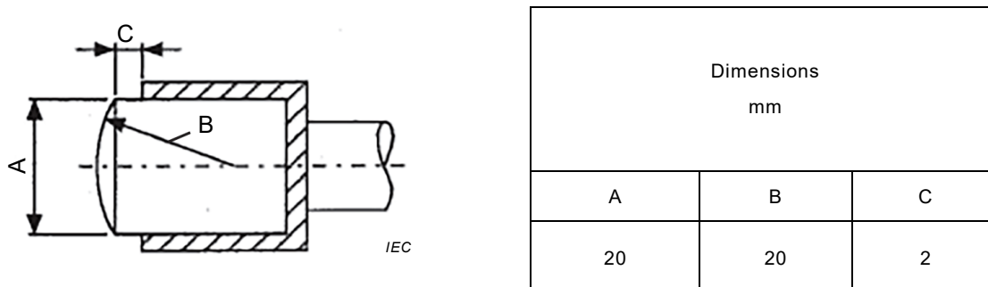
Figure 4 – Test piston dimensions
