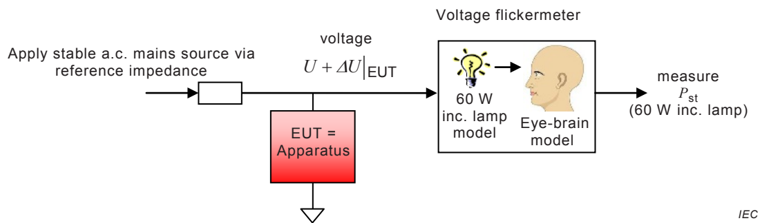
Figure 1a – Voltage fluctuation emission test IEC 61000-3-3, using the IEC voltage flickermeter IEC 61000-4-15
