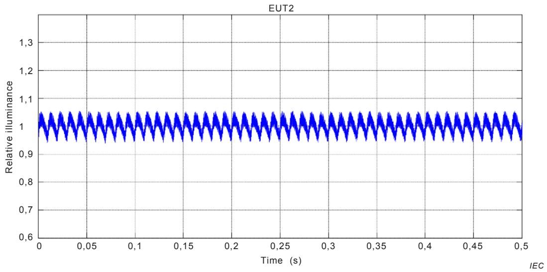
Figure C.3 – EUT2: relative illuminance: mains voltage modulation d = 0,407\% at 13,5 Hz ( P_{st} = 1 )
