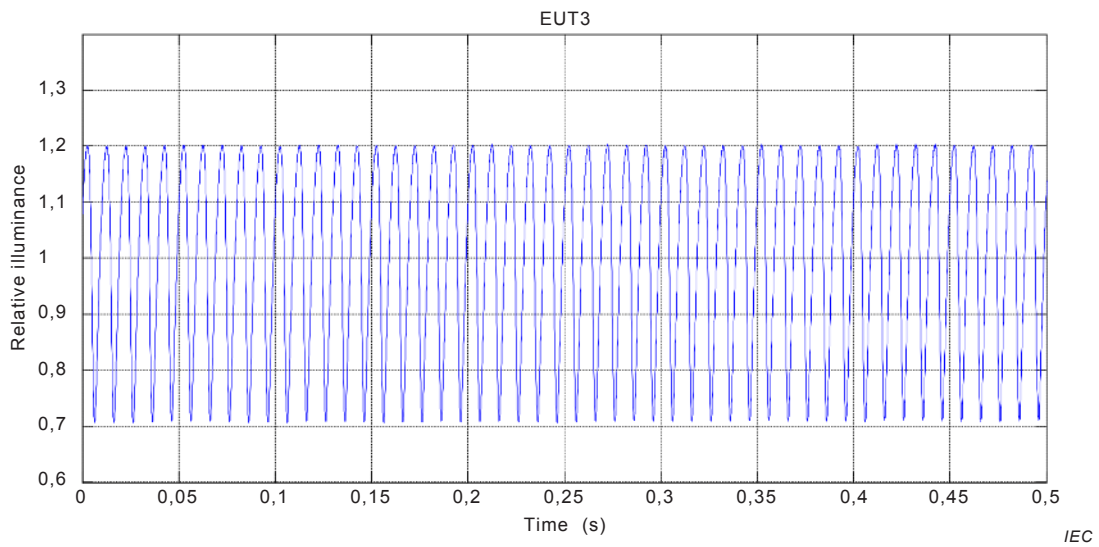
Figure C.4 – EUT3: relative illuminance: mains voltage modulation d = 0,407\% at 13,5 Hz ( P_{st} = 1 )
