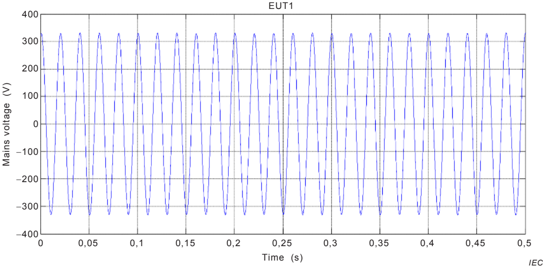
a) Mains signal with modulation d = 0,407\% at 13,5\text{ Hz} ( P_{st} = 1 )
