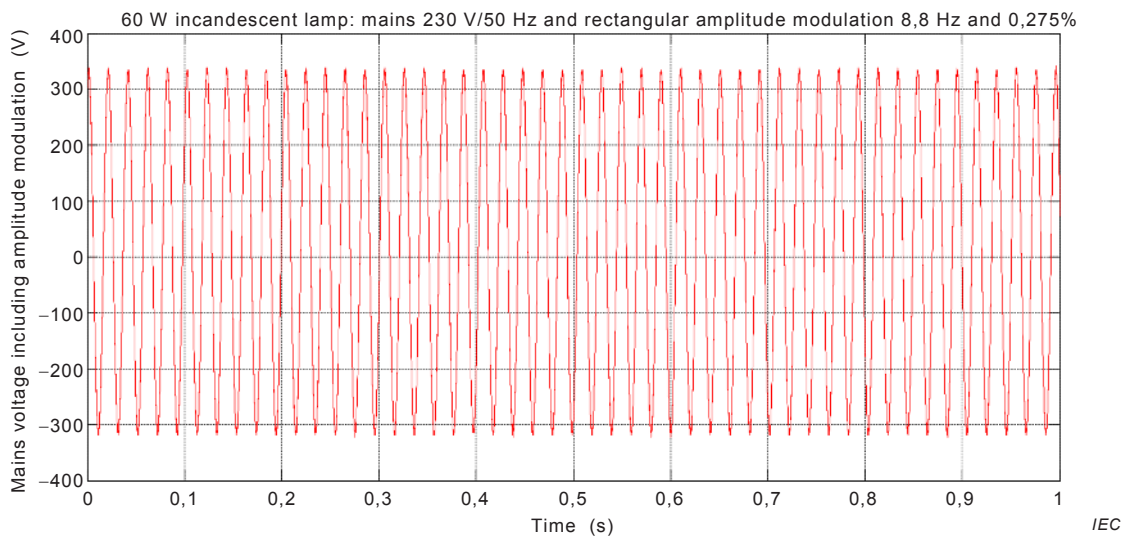
a) Mains voltage fluctuation with rectangular modulated of 8,8 Hz and d = 0,275 \%
