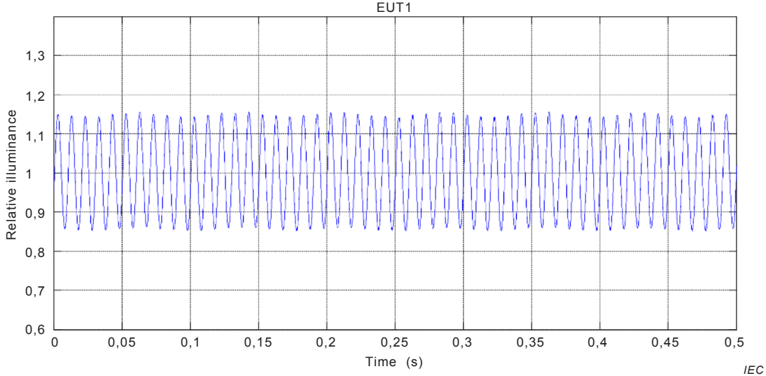
b) Relative illuminance
