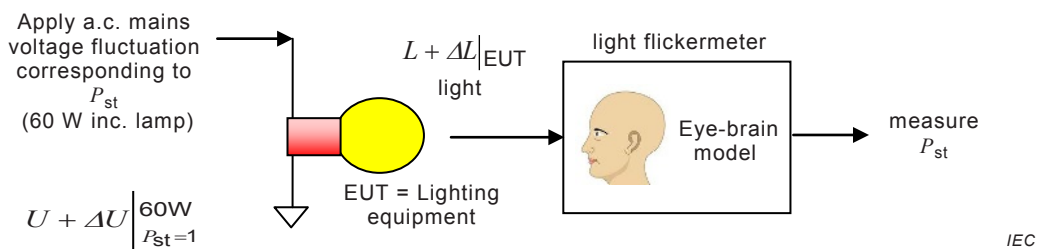
Figure 1b – Voltage fluctuation immunity test specified in this technical report
