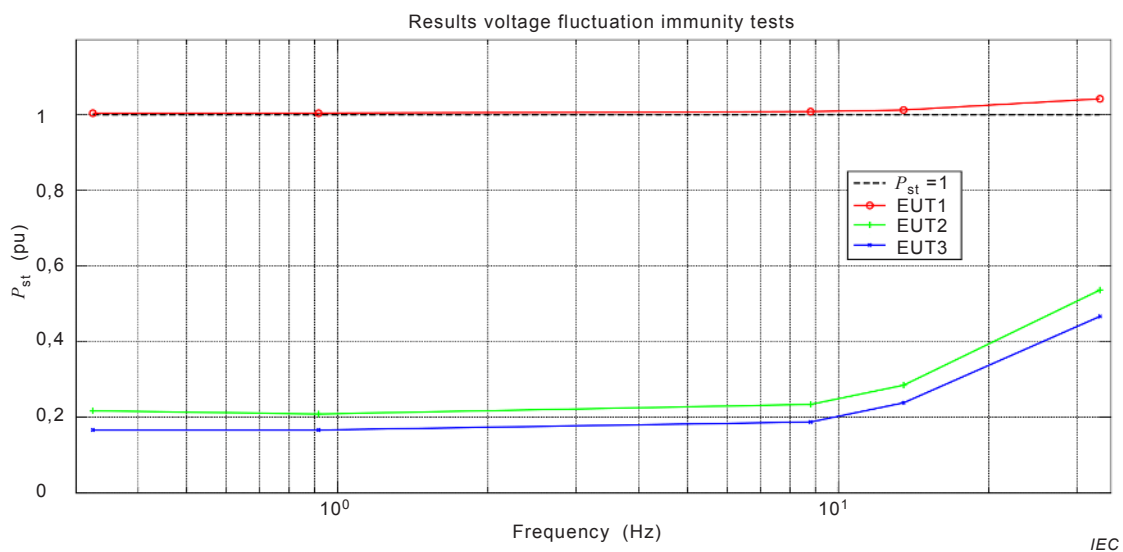
Figure C.5 – Graphical P_{st} results for three EUTs with rectangular modulation at five frequencies ( P_{st} = 1 )
