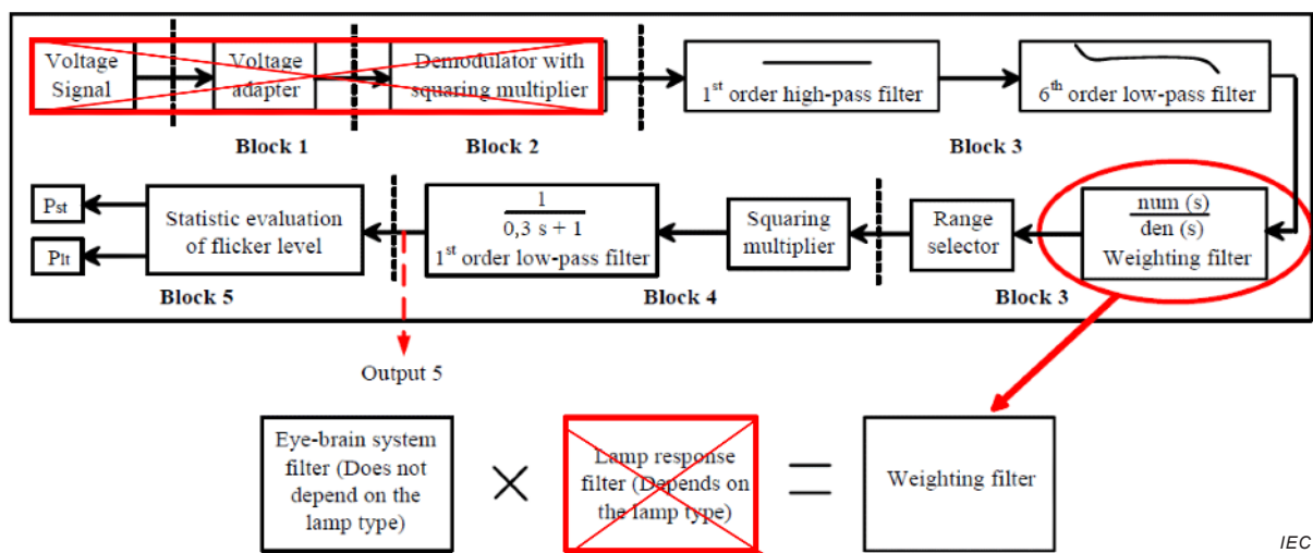
Figure A.1 – Structure of the IEC 61000-4-15 flickermeter which uses voltage as input
