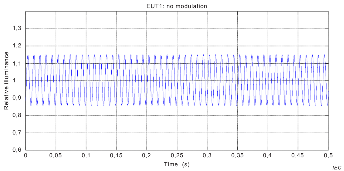
a) Mains signal
