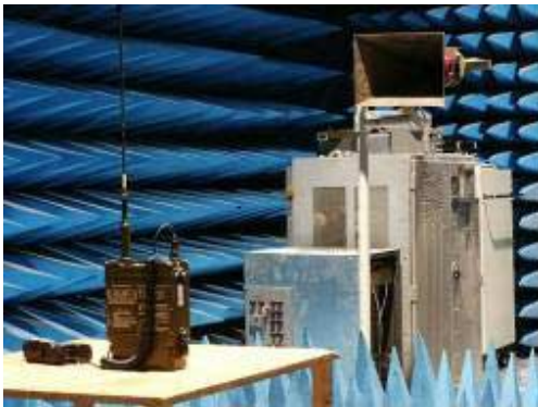
HPM generator 3 GHz during testing in semianechoic chamber
