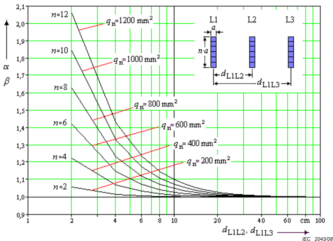
a) For one bar per main conductor; a = 10 mm
