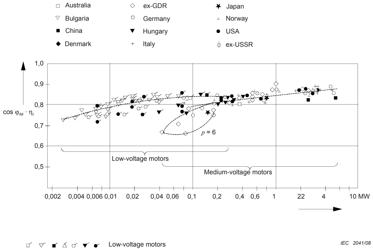
Figure 14 – Product \cos \varphi_{TM} \times \eta_{rM} of low-voltage and medium-voltage motors, 50 Hz and 60 Hz
