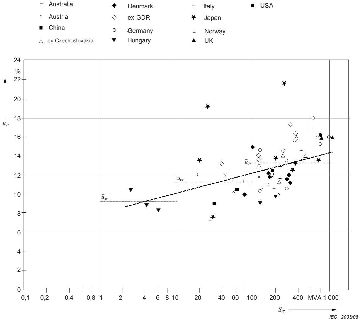
Figure 6 – Rated short-circuit voltages u_{kr} of network transformers
