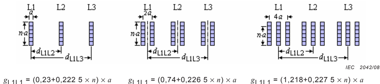
Figure 15 – Geometric mean distance g_{L1L1} = g_{L2L2} = g_{L3L3} of the main conductors
