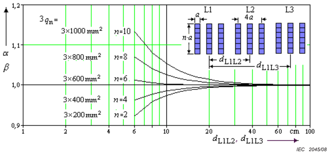
c) For three bars per main conductor; a = 10 \text{ mm}
