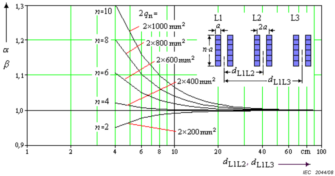
b) For two bars per main conductor; a = 10 \text{ mm}
