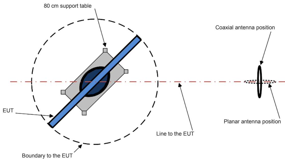
Figure 1 – Setup of a plasma display panel TV for magnetic-field measurement
