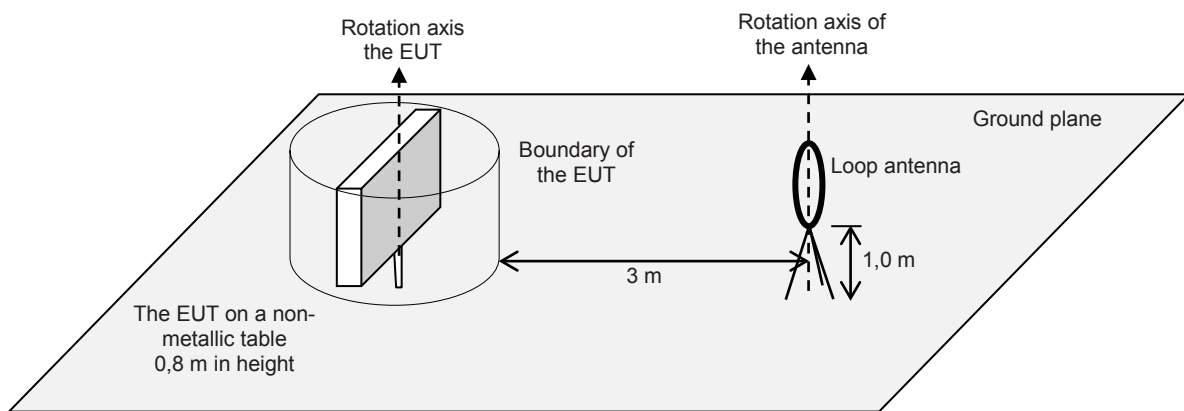
Figure 1 – Setup of a plasma display panel TV for magnetic-field measurement
