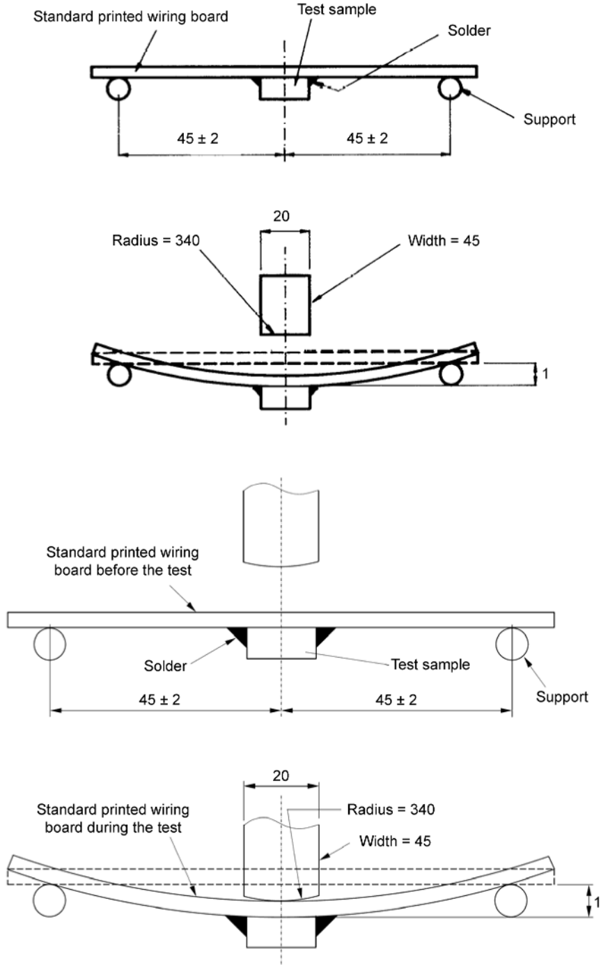
Figure 4 – Bending jig for surface mount fuse resistors with particular overcurrent protection
