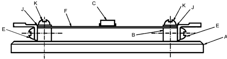
Figure 3b – Surface mount fuse resistor with particular overcurrent protection (printed circuit track on top)
