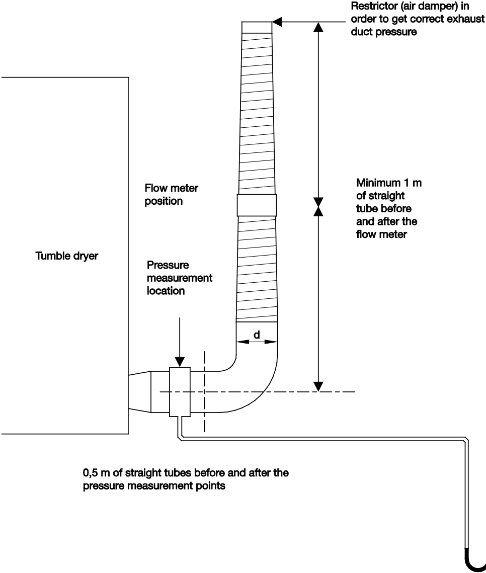
Figure B.2 — Exhaust duct Type 2
