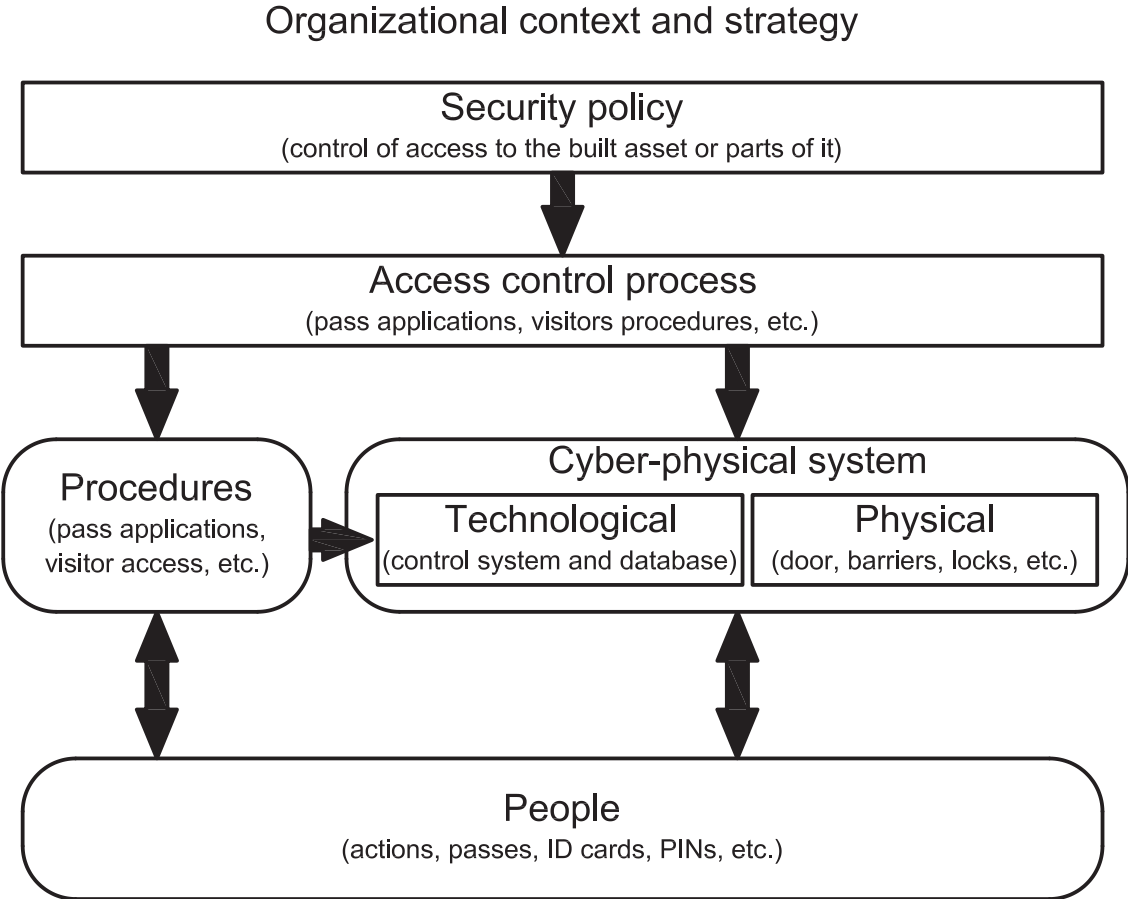
Figure 4 – Example of interaction of security aspects to provide access control to a building
