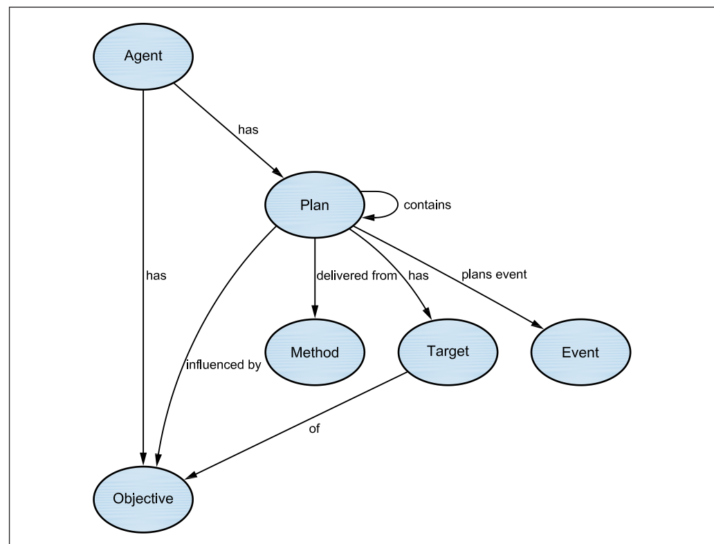
Figure 14 PLANS view
