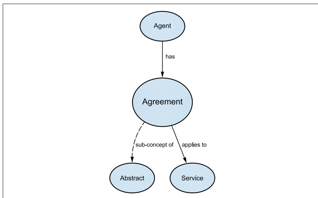
Figure 19 AGREEMENT relationships
