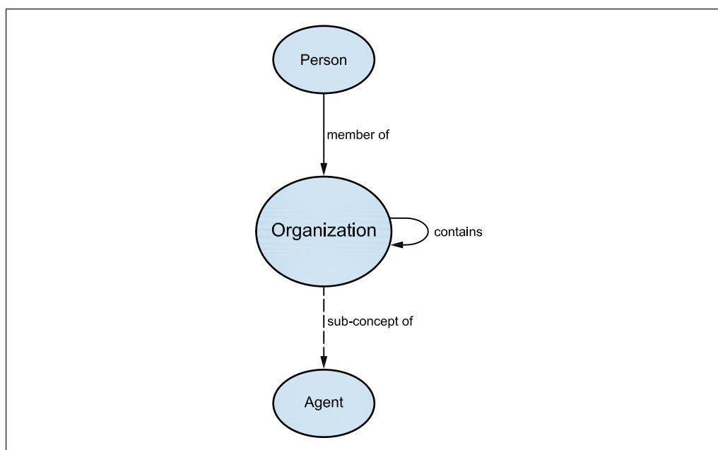
Figure 34 ORGANIZATION relationships
