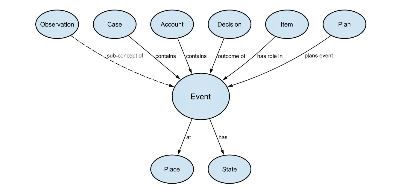
Figure 26 EVENT relationships
