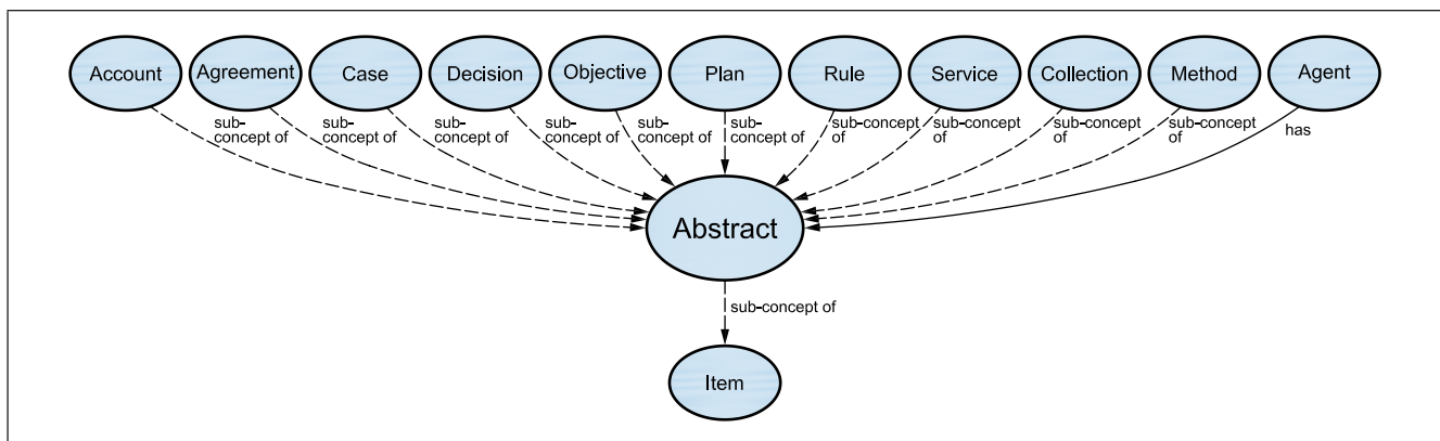
Figure 16 ABSTRACT relationships
