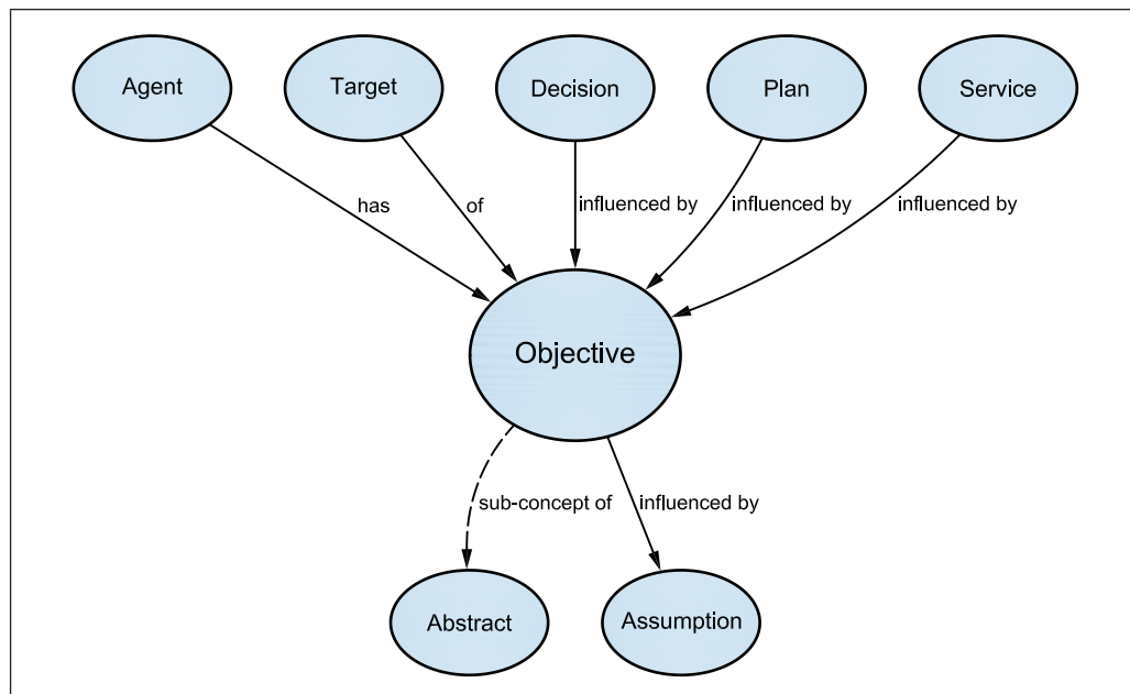
Figure 32 OBJECTIVE relationships
