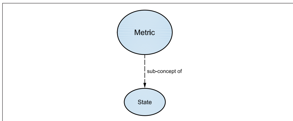
Figure 30 METRIC relationships
