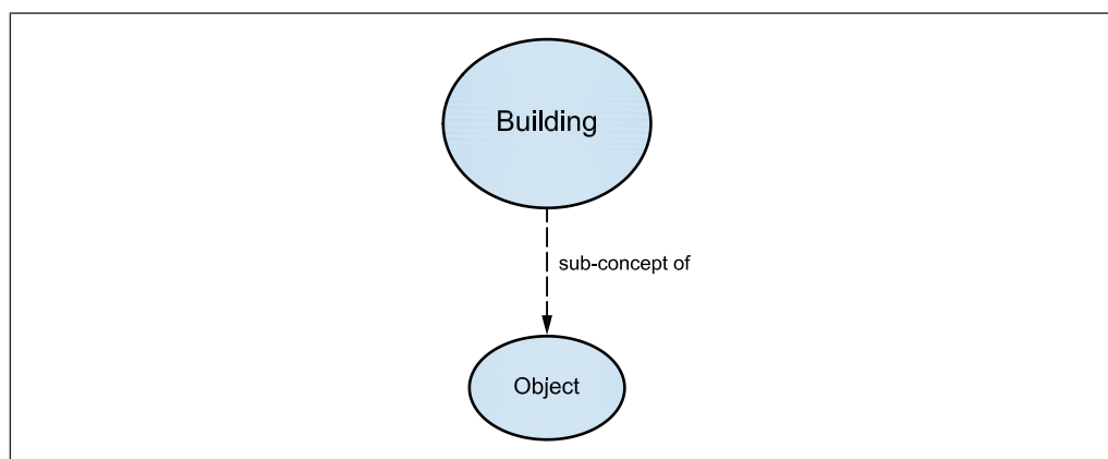
Figure 21 BUILDING relationships
