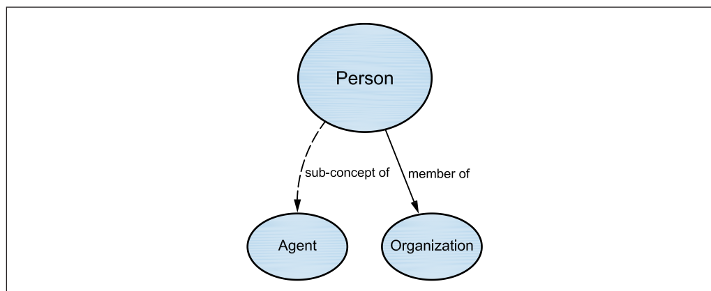
Figure 35 PERSON relationships
