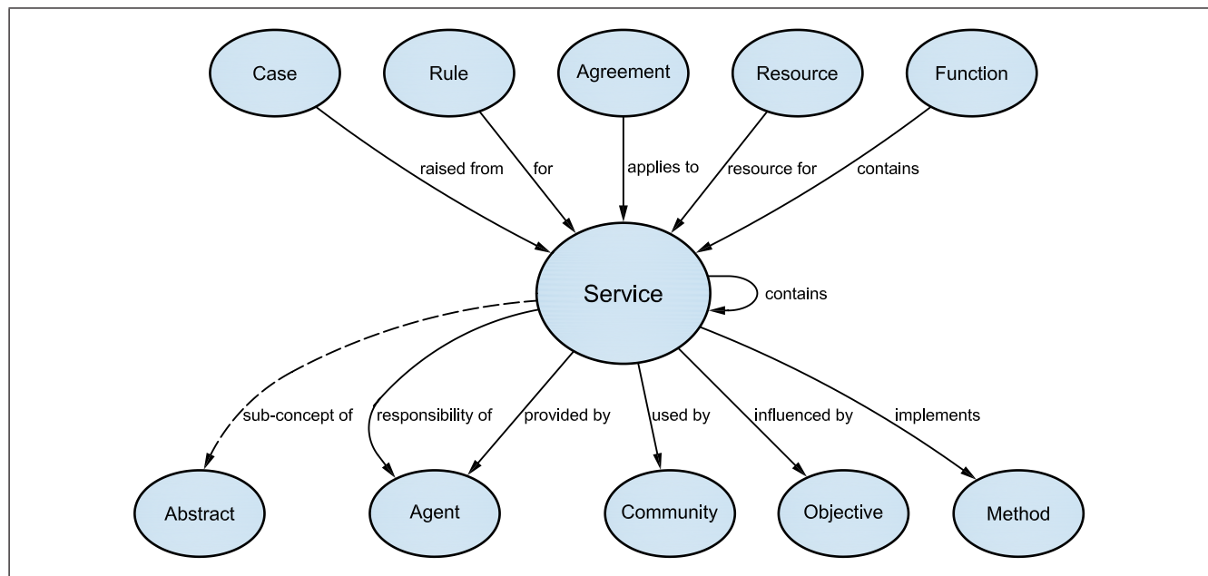
Figure 40 SERVICE relationships
