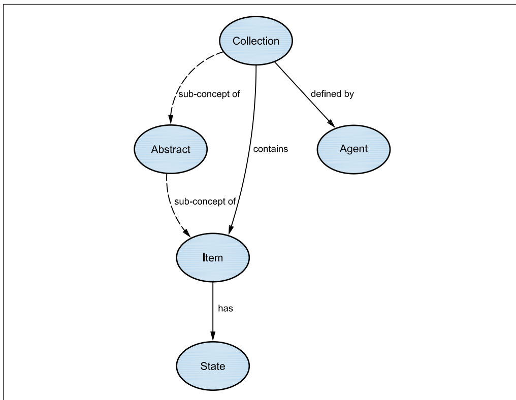
Figure 8 COLLECTIONS view
