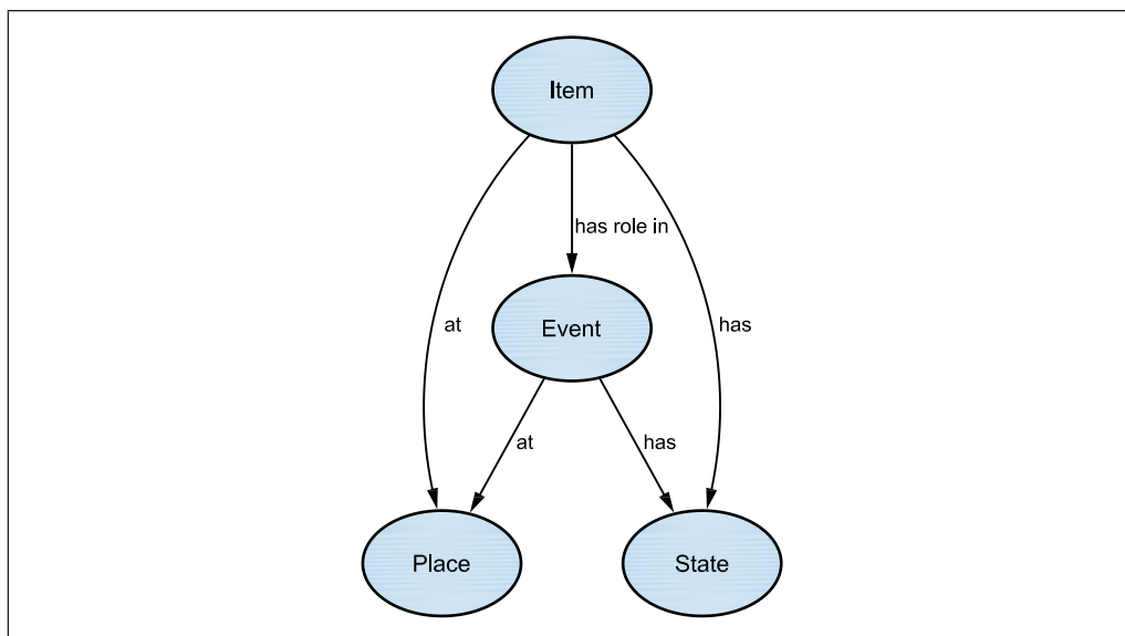
Figure 9 EVENTS view
