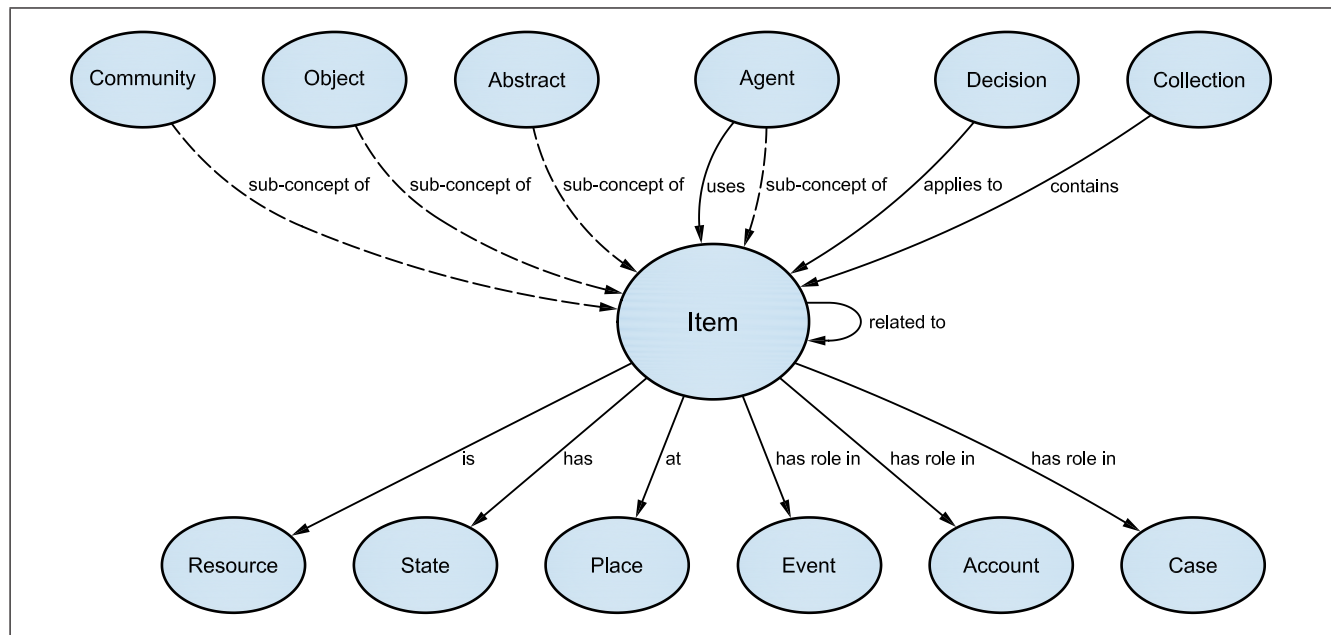
Figure 28 ITEM relationships
