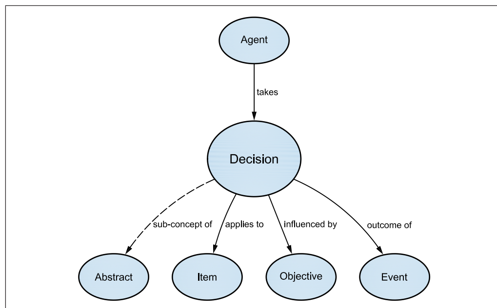
Figure 25 DECISION relationships
