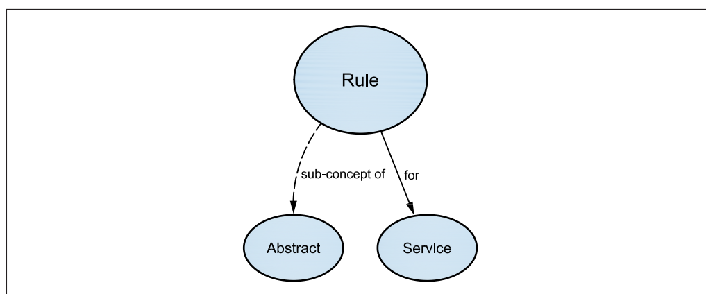
Figure 39 RULE relationships
