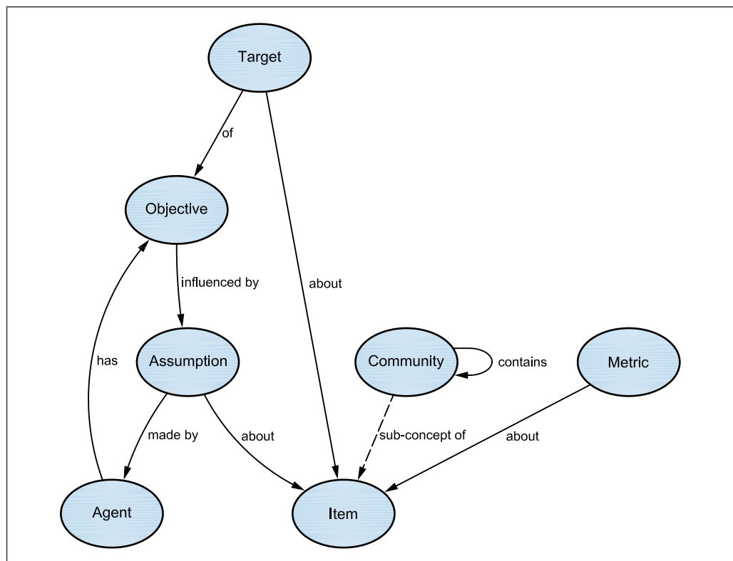
Figure 10 OBJECTIVES view
