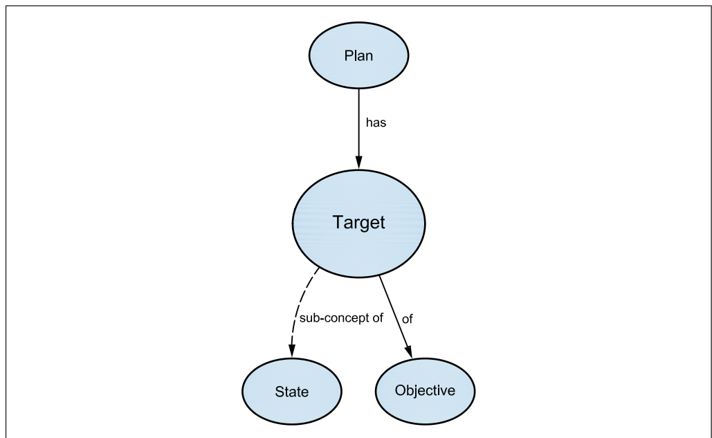
Figure 42 TARGET relationships
