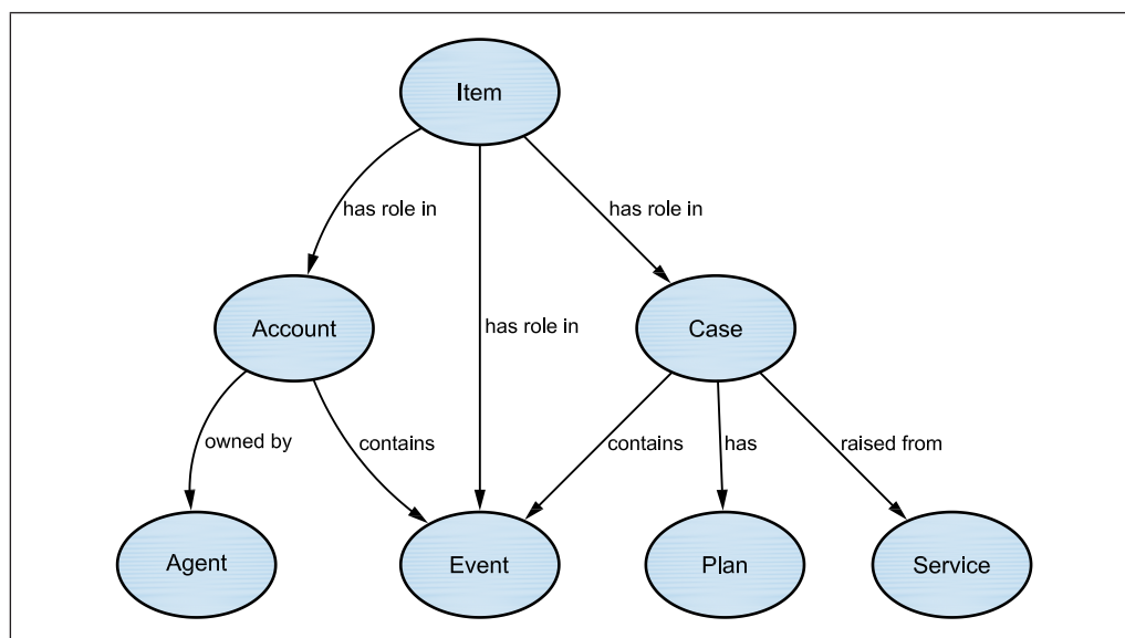
Figure 13 CASEs view
