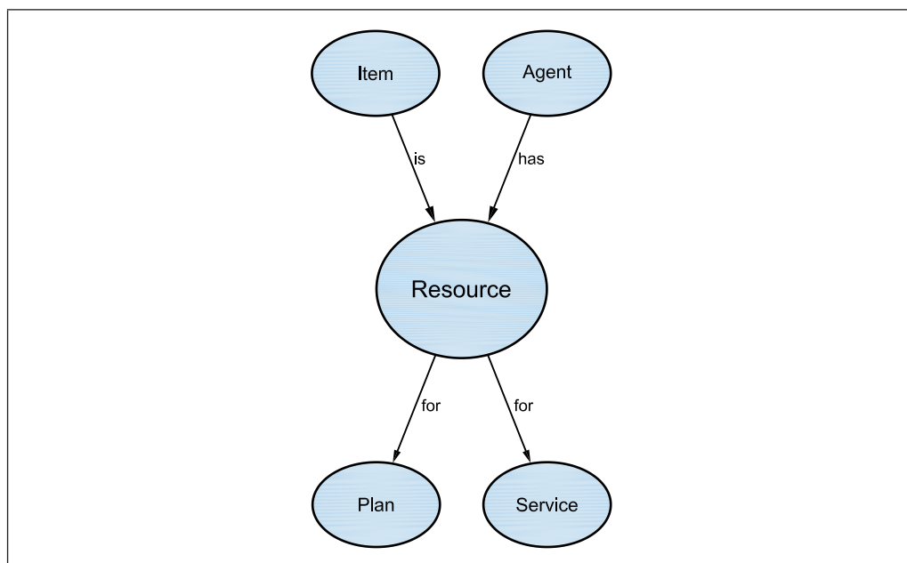
Figure 38 RESOURCE relationships
