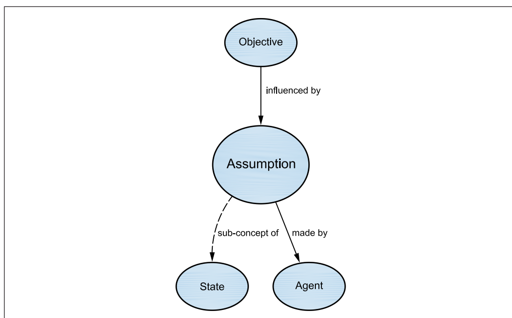
Figure 20 ASSUMPTION relationships
