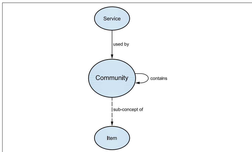
Figure 24 COMMUNITY relationships
