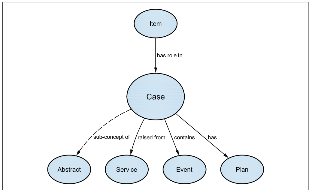
Figure 22 CASE relationships
