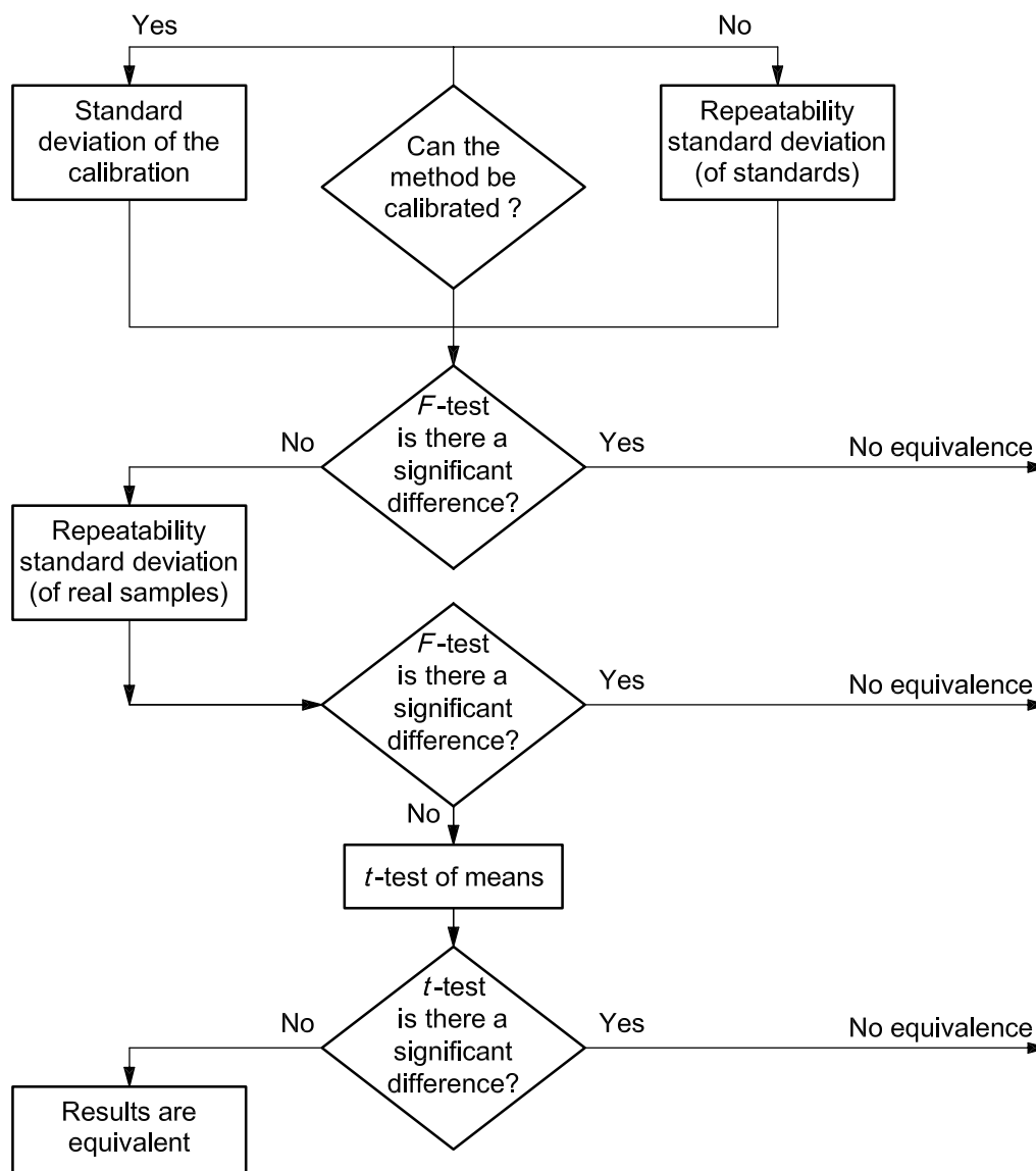
Figure G.1 — Schematic diagram where concentration levels are similar
