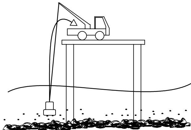
Figure 4 — Diagram of the submersible-pump version of a moveable-orifice pumping sampler
