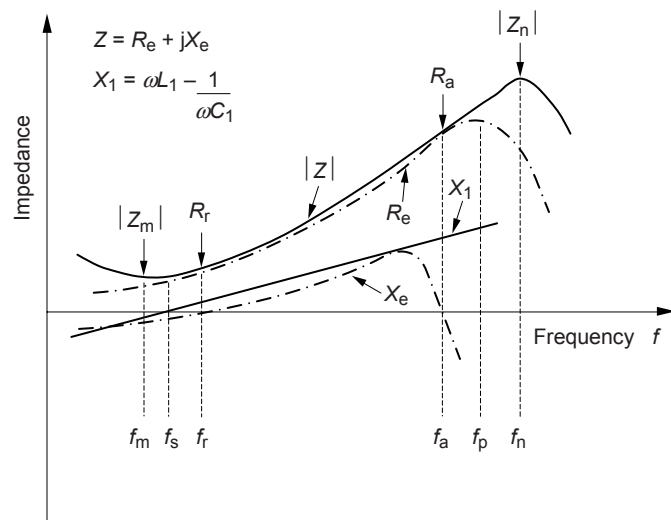
Figure 3 – Frequency characteristics of the impedance near resonance
