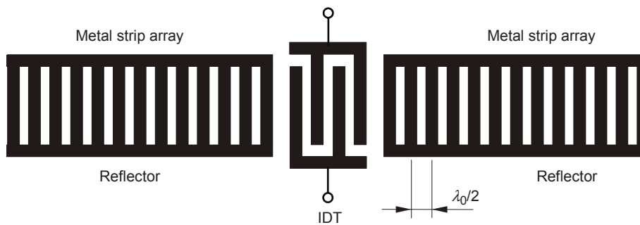
Figure 6 – Configuration of a one port SAW resonator
