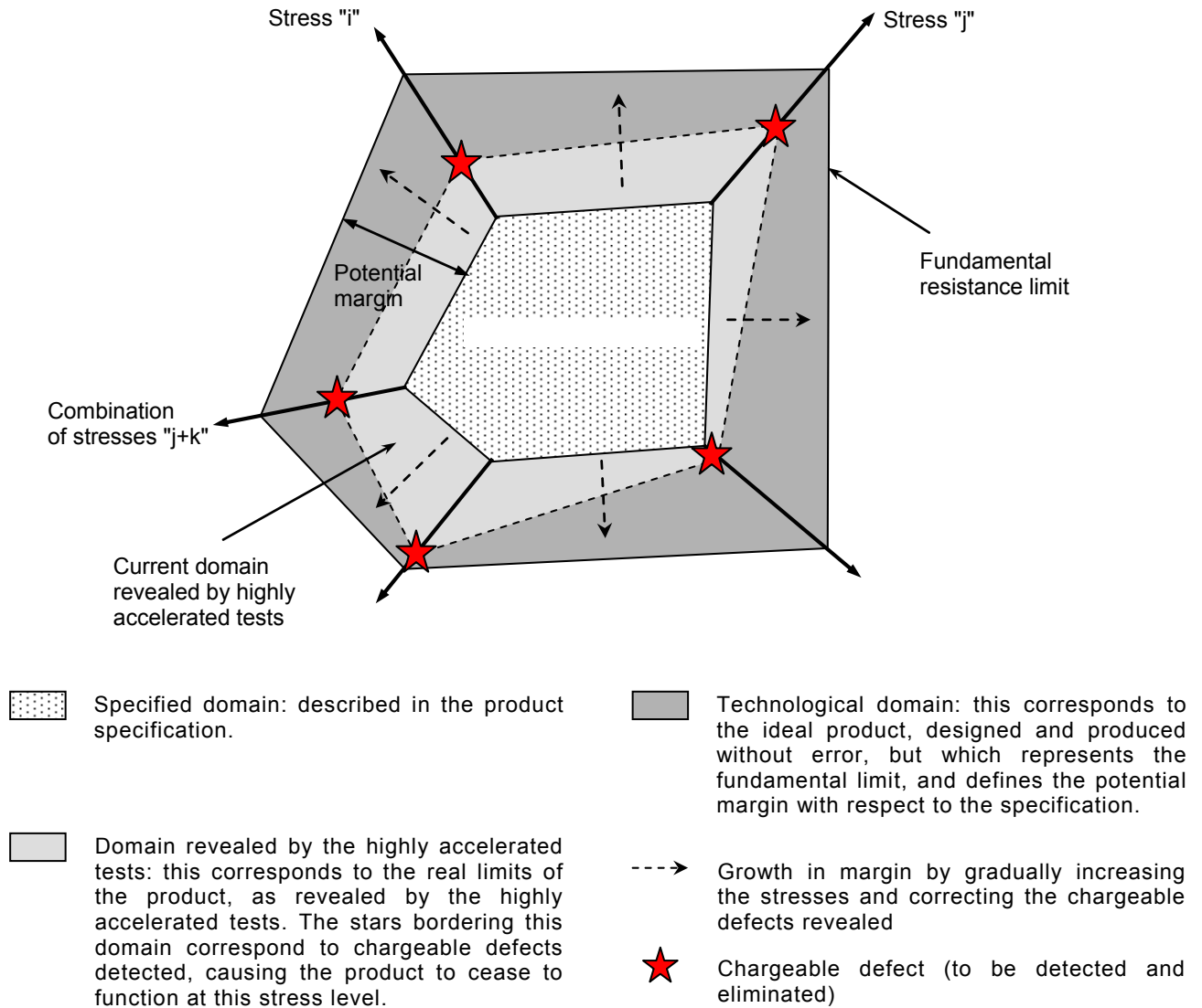
Figure 1 – Exploration of margins using a highly accelerated test
