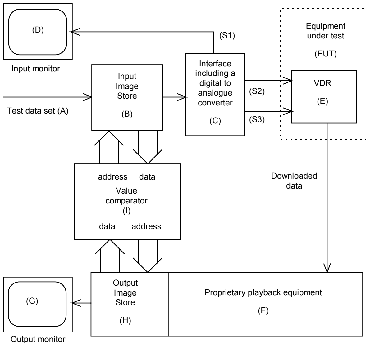
Figure 1 – Test set-up block diagram
