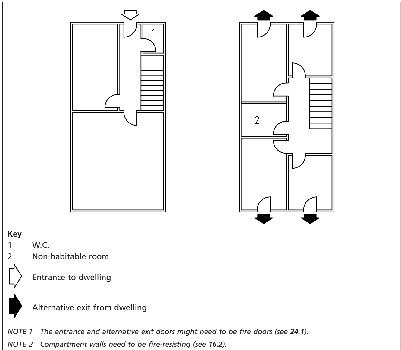
Figure 2 Maisonette with alternative exits from each room not on the floor of entrance
