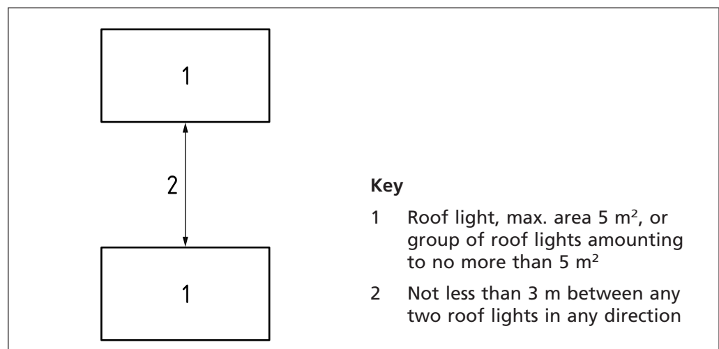
Figure 23 Limitations on spacing and size of plastic roof lights having a Class 3 or TP(b) lower surface
