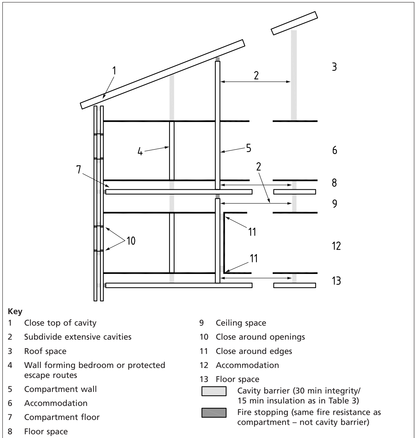
Figure 24 Provisions for cavity barriers
