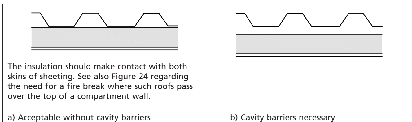
Figure 27 Provisions for cavity barriers in double skinned insulated roof sheeting
