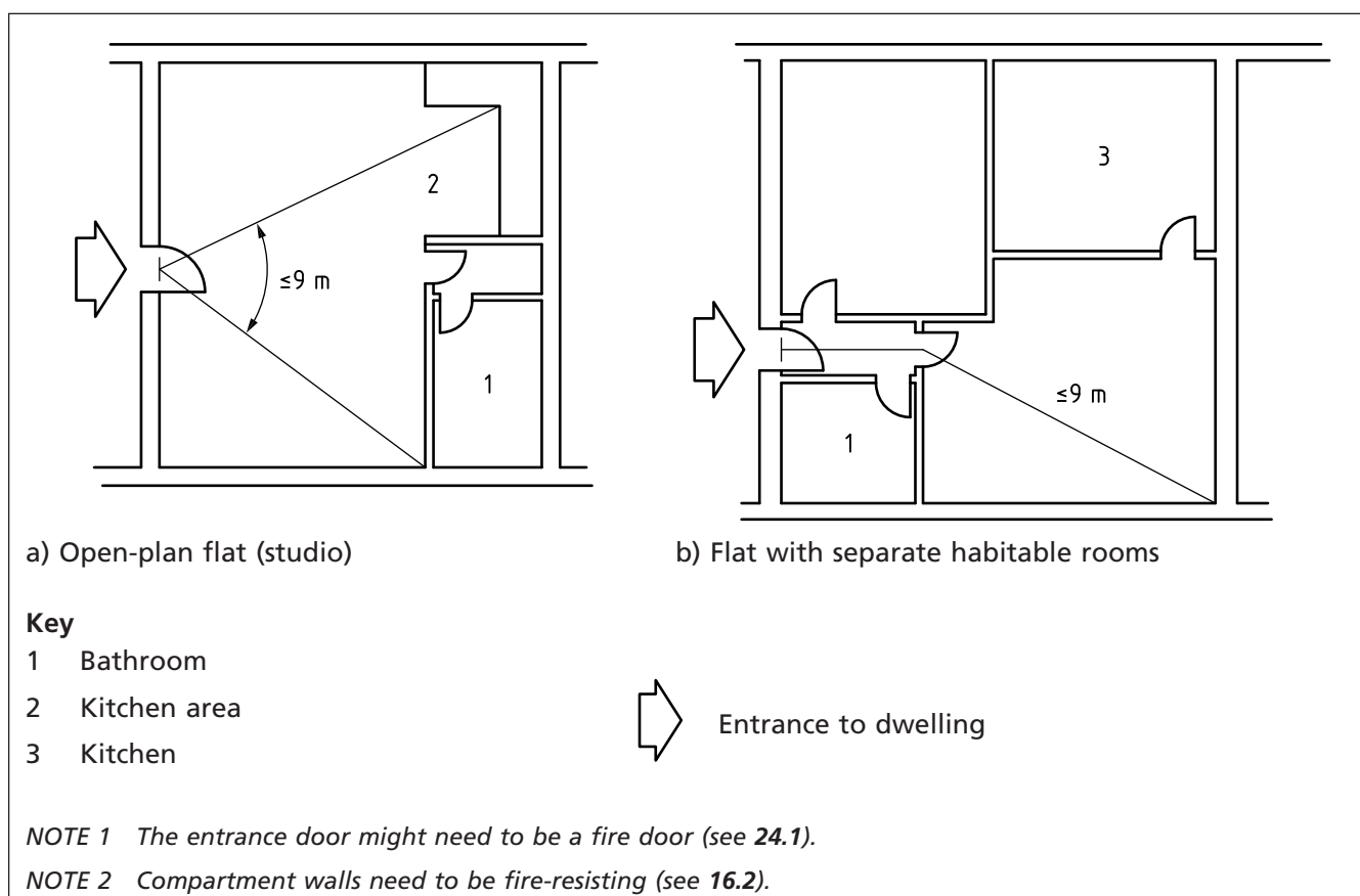
Figure 10 Flat with restricted travel distance
