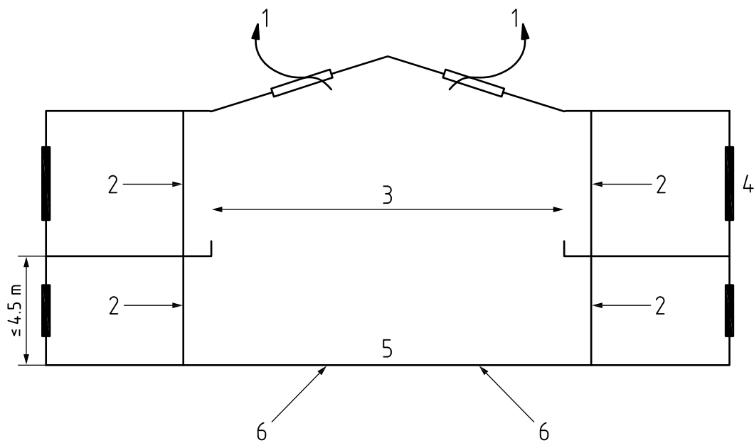
Figure C.2 Exemplar 1: Atrium base: no control required
