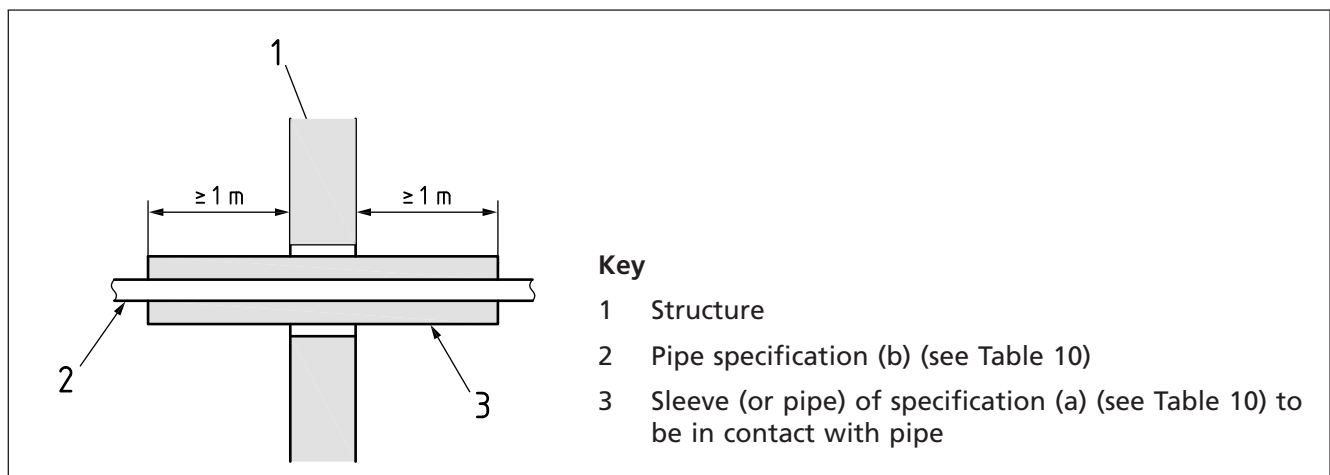
Figure 30 Pipes penetrating structure
