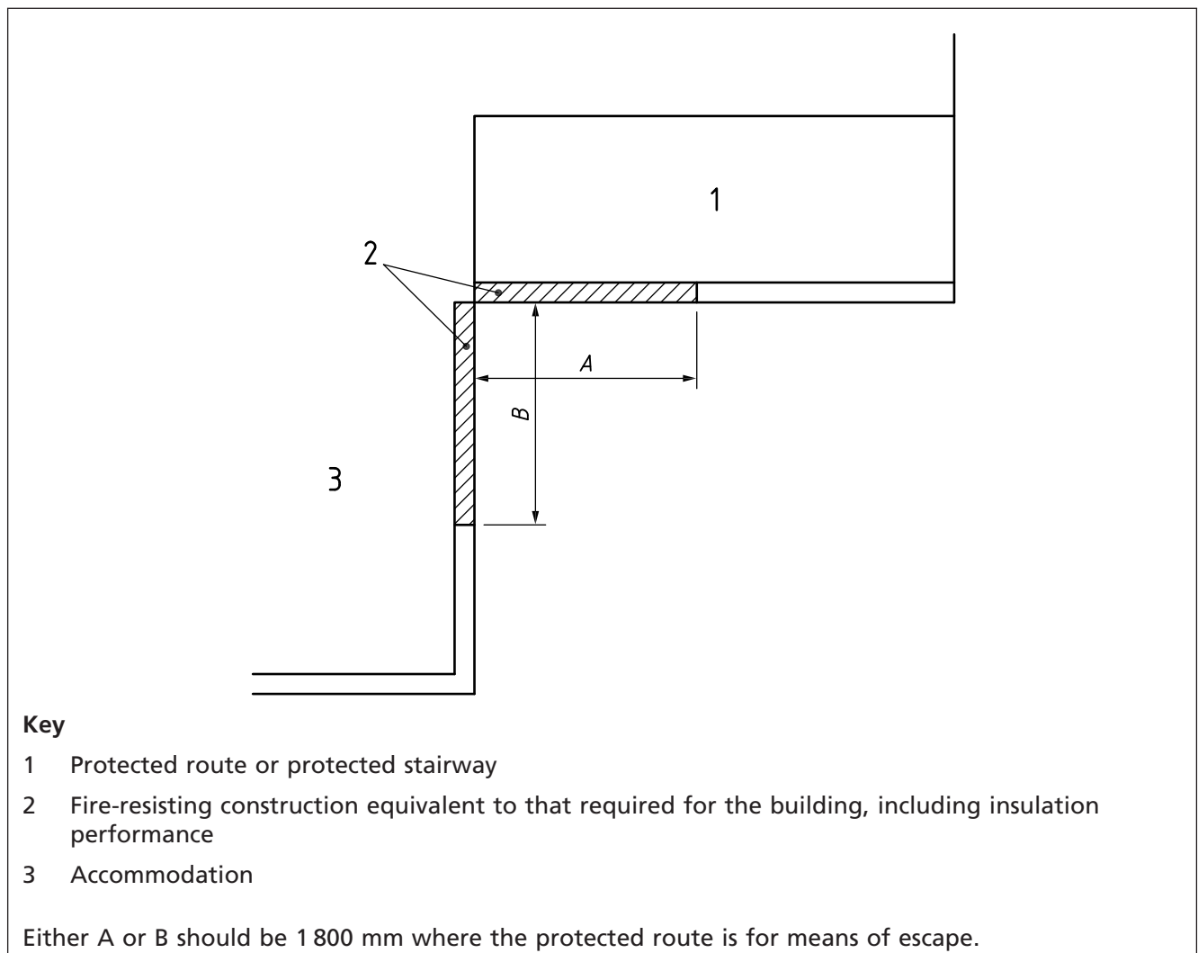
Figure 31 Protected routes forming an internal angle
