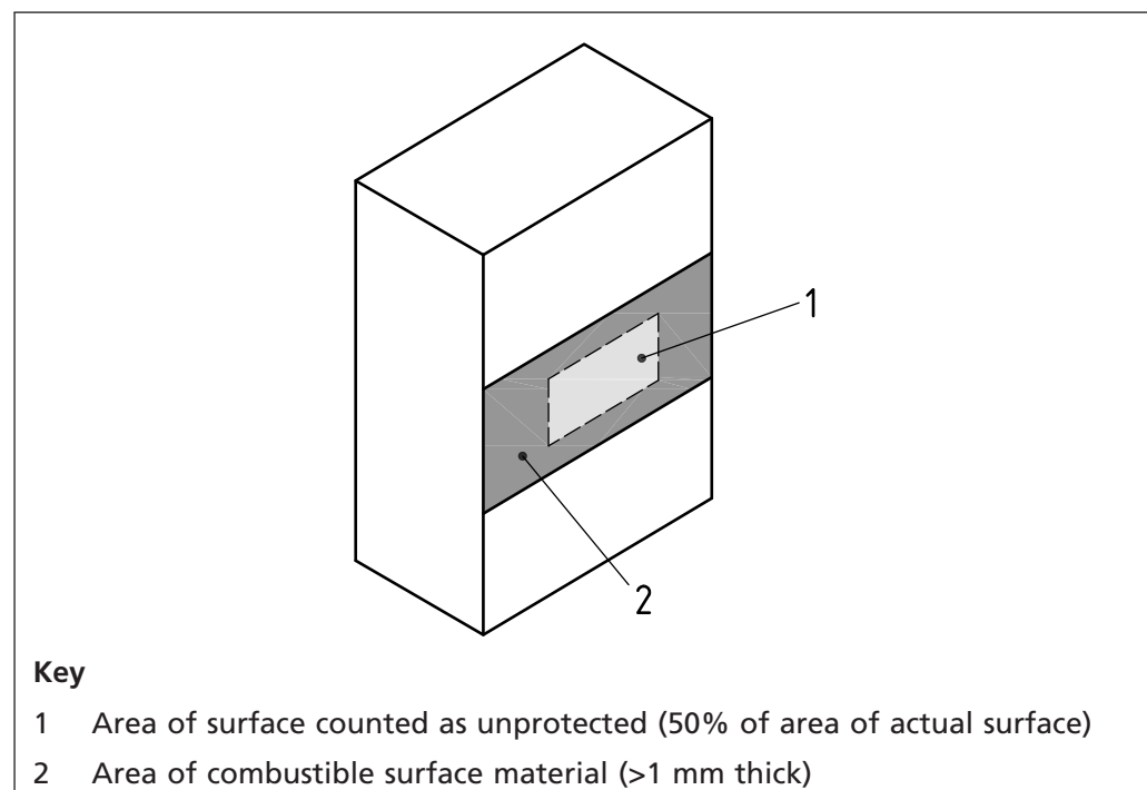
Figure 20 Combustible surface material as unprotected area
