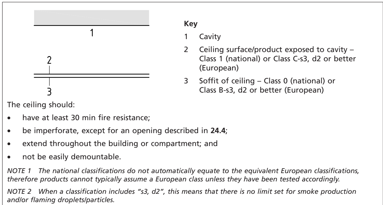
Figure 26 Fire-resisting ceiling below concealed space
