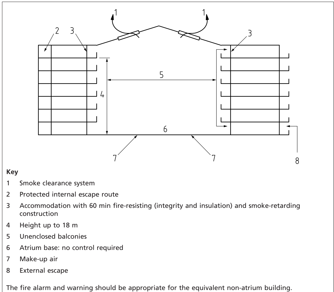
Figure C.3 Exemplar 2: Atrium base: no control required
