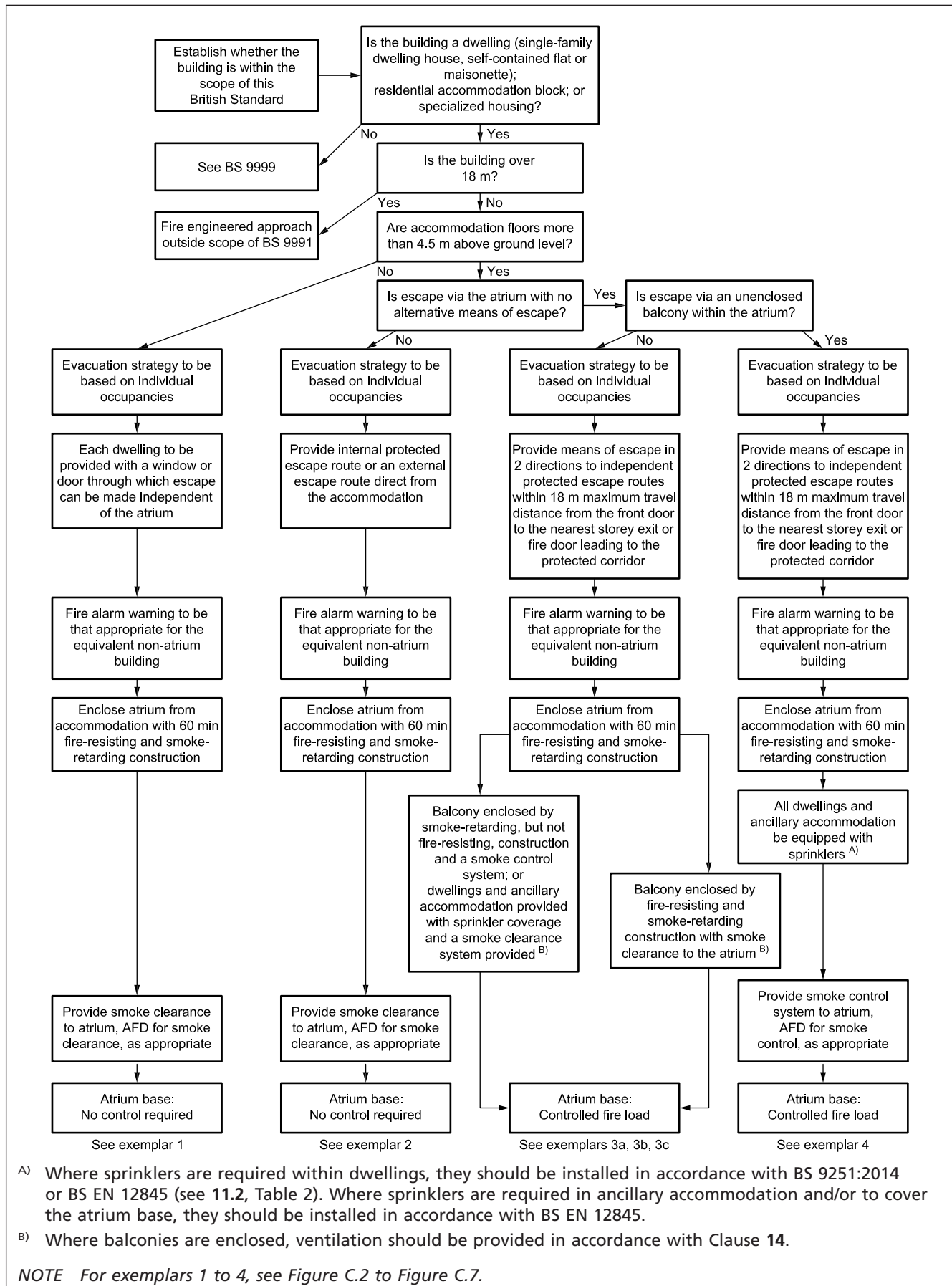
Figure C.1 Occupancy category decision process
