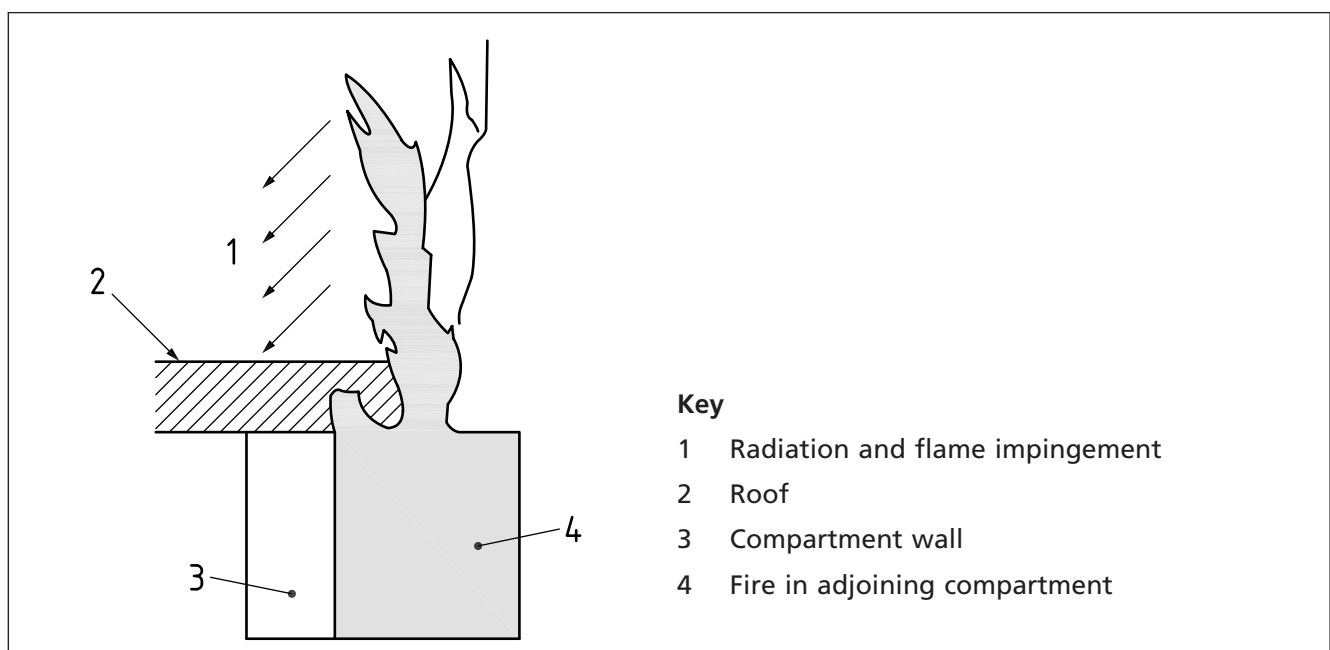
Figure 22 Roof covering adjoining line of compartmentation
