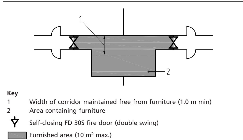
Figure 9 Furnished areas in specialized housing corridors
