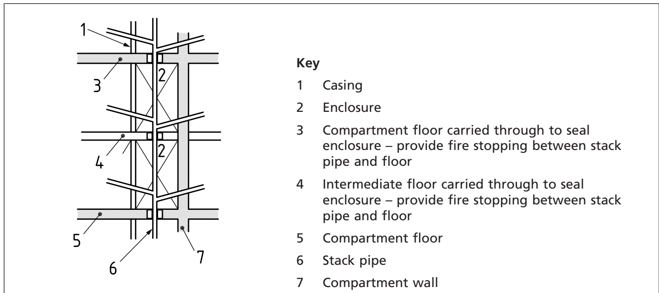
Figure 30 Pipes penetrating structure
