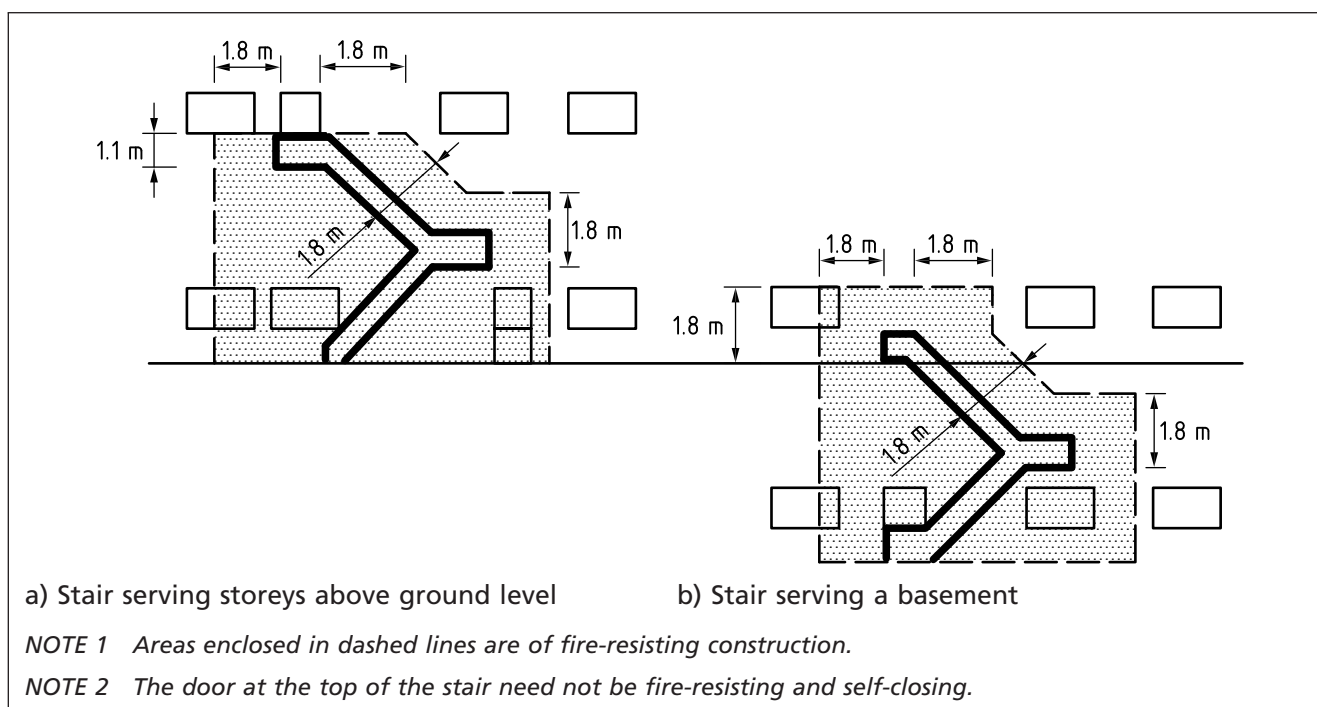
Figure 33 Fire resistance of areas adjacent to external stairs
