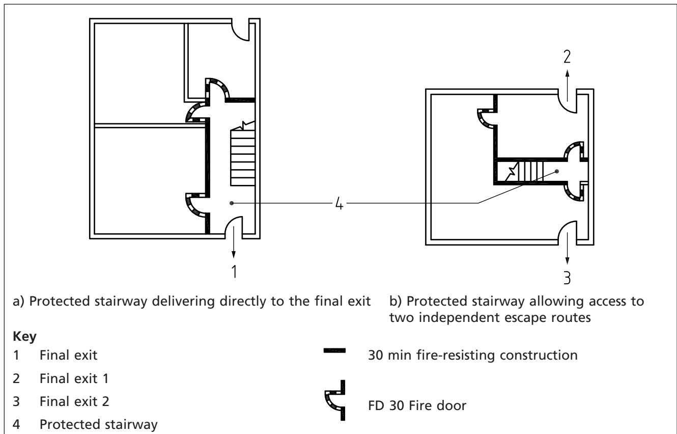
Figure 1 Alternative arrangements for escape via the ground storey in houses exceeding 4.5 m in height
