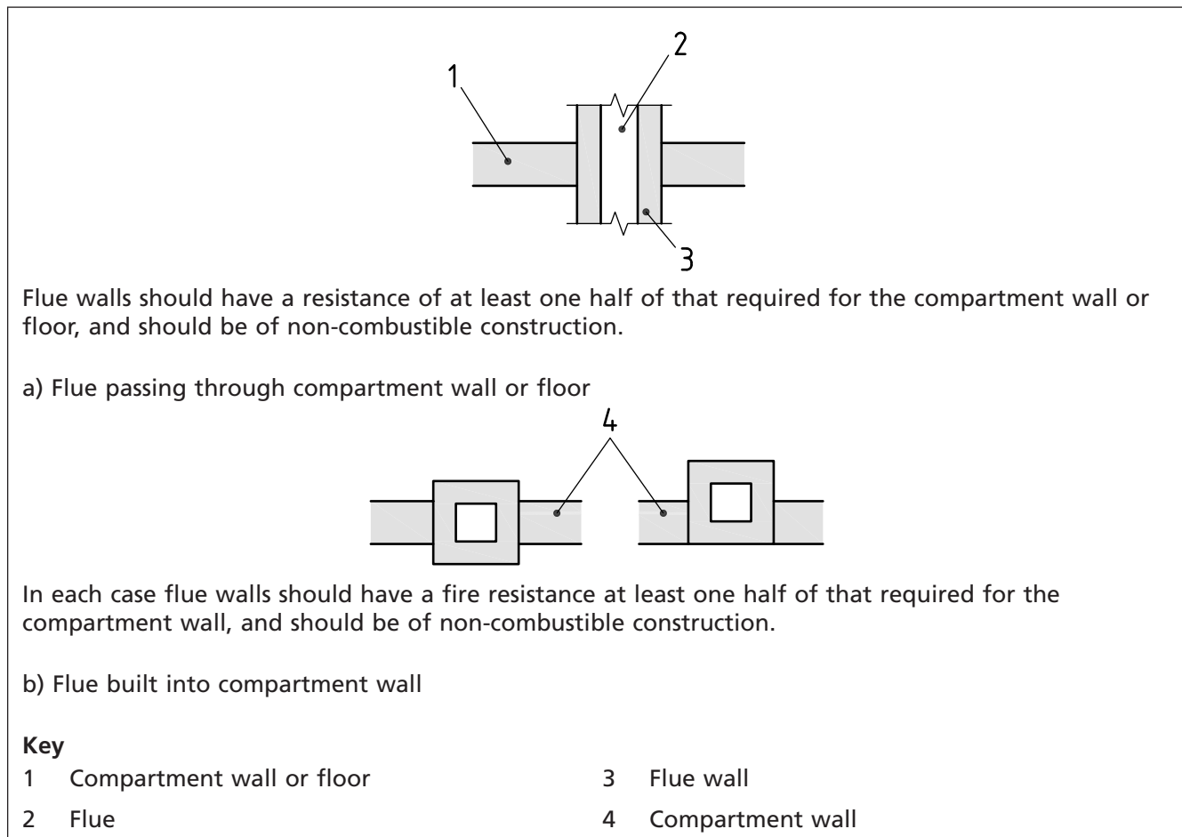
Figure 28 Flues and compartment walls and floors
