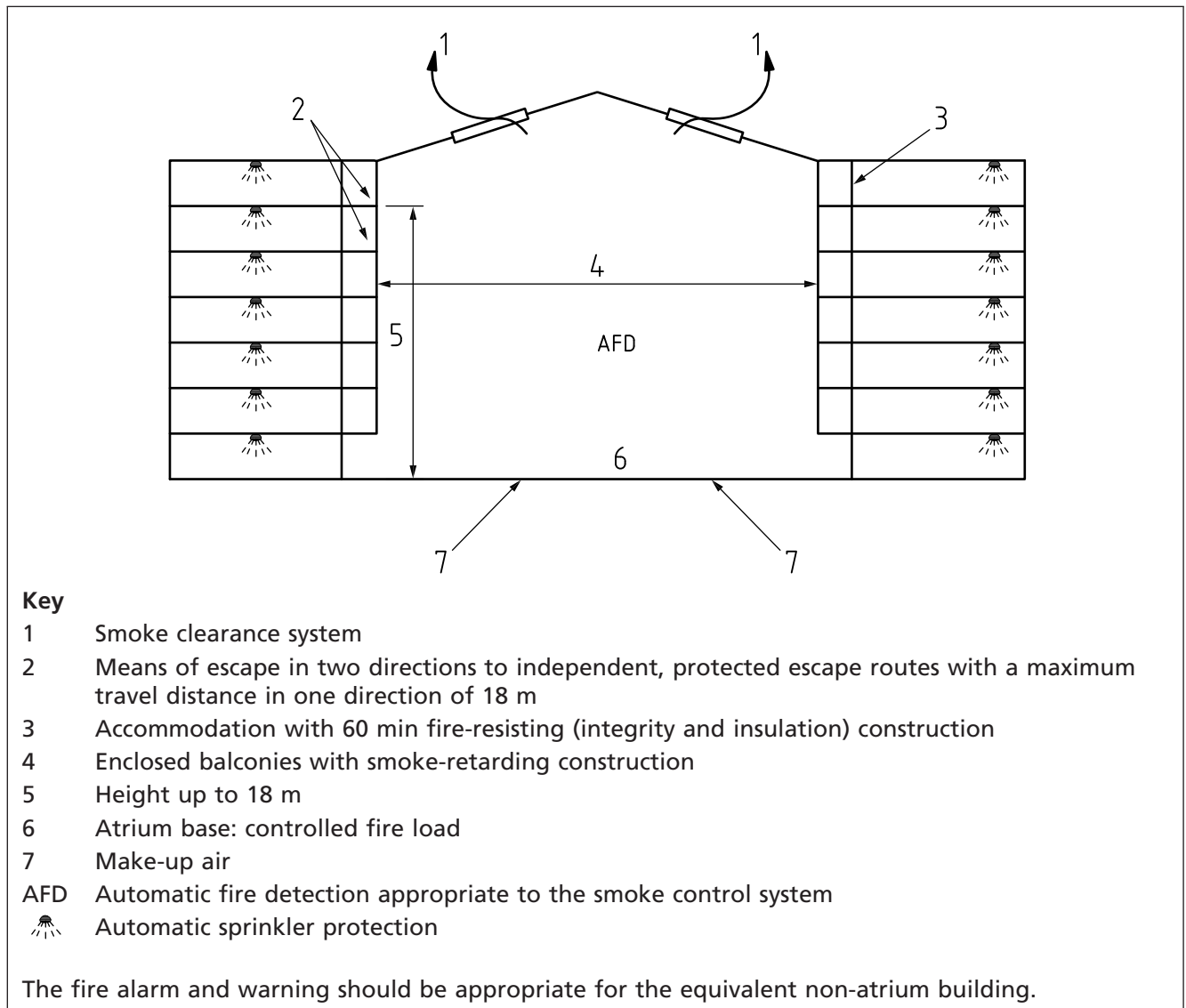
Figure C.6 Exemplar 3c: Atrium base: controlled fire load
