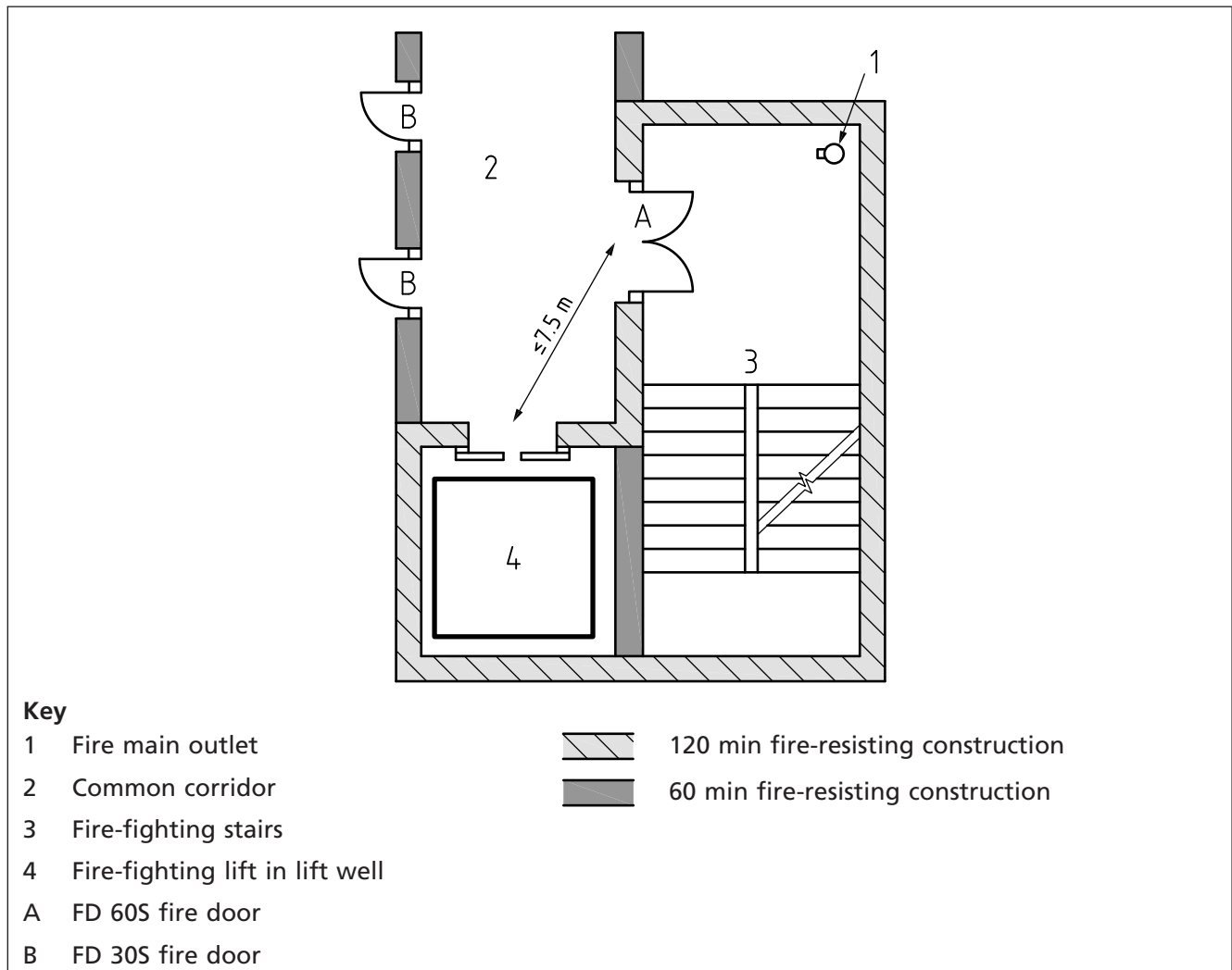
Figure 35 Components of a residential fire-fighting shaft
