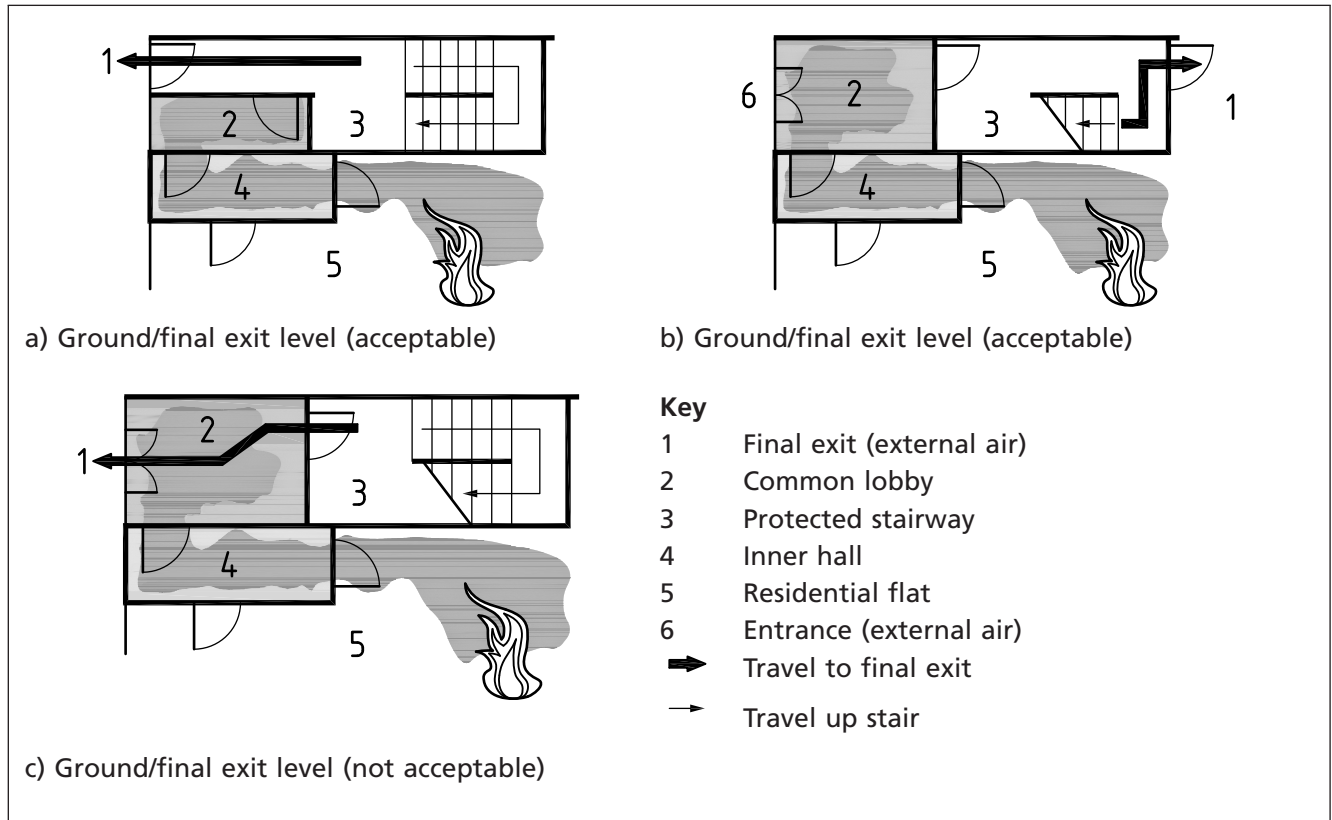
Figure 34 Lobby protection to final exit from stairway
