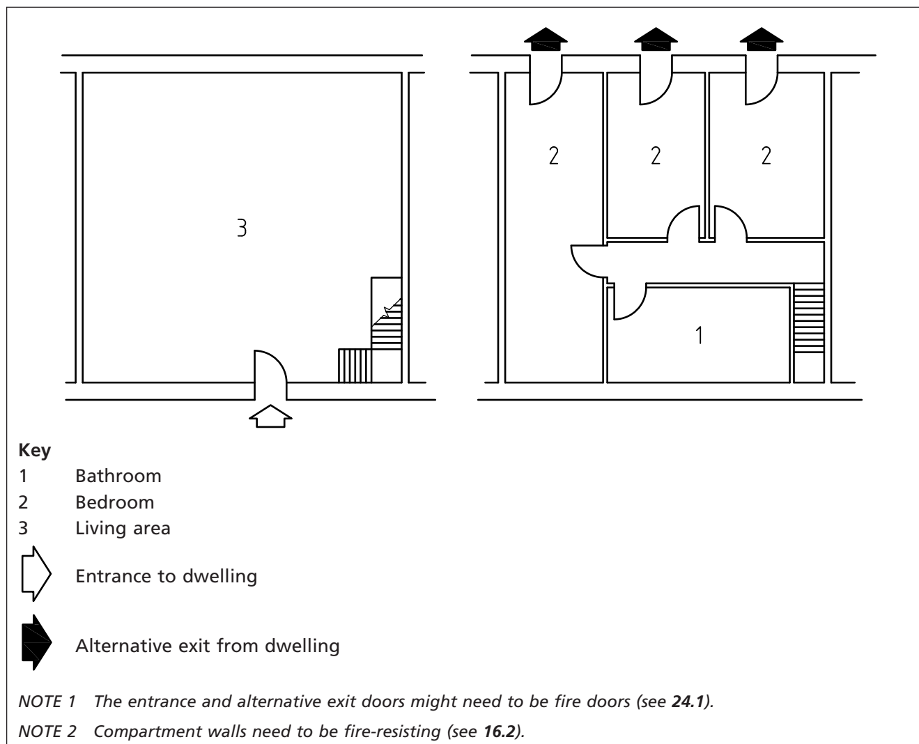
Figure 4 Open-plan maisonette
