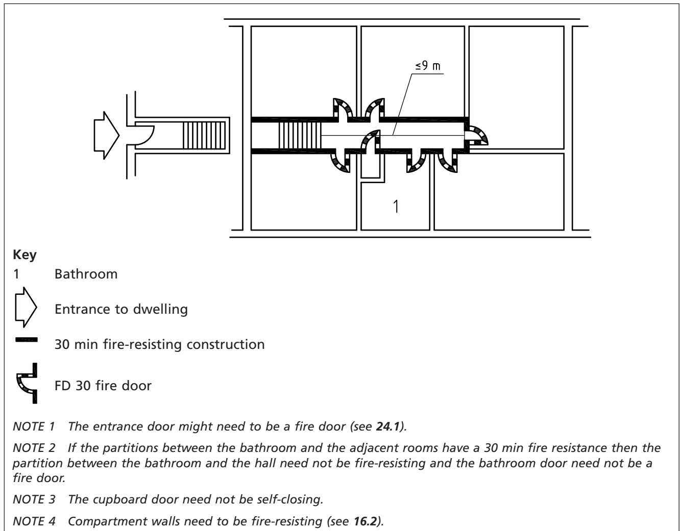
Figure 14 Flat (entered from below) with a protected entrance hall and restricted travel distance
