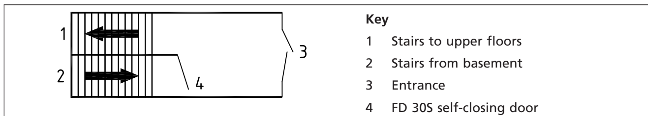
Figure 32 Staircase separating basement and upper storeys in single stair residential buildings
