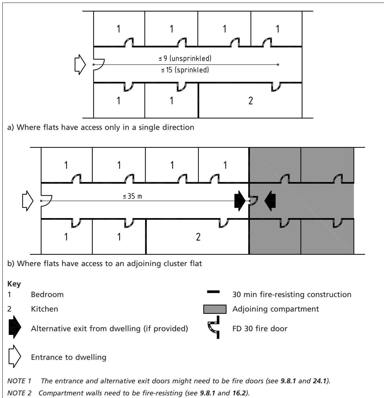
Figure 16 Typical cluster accommodation layout
