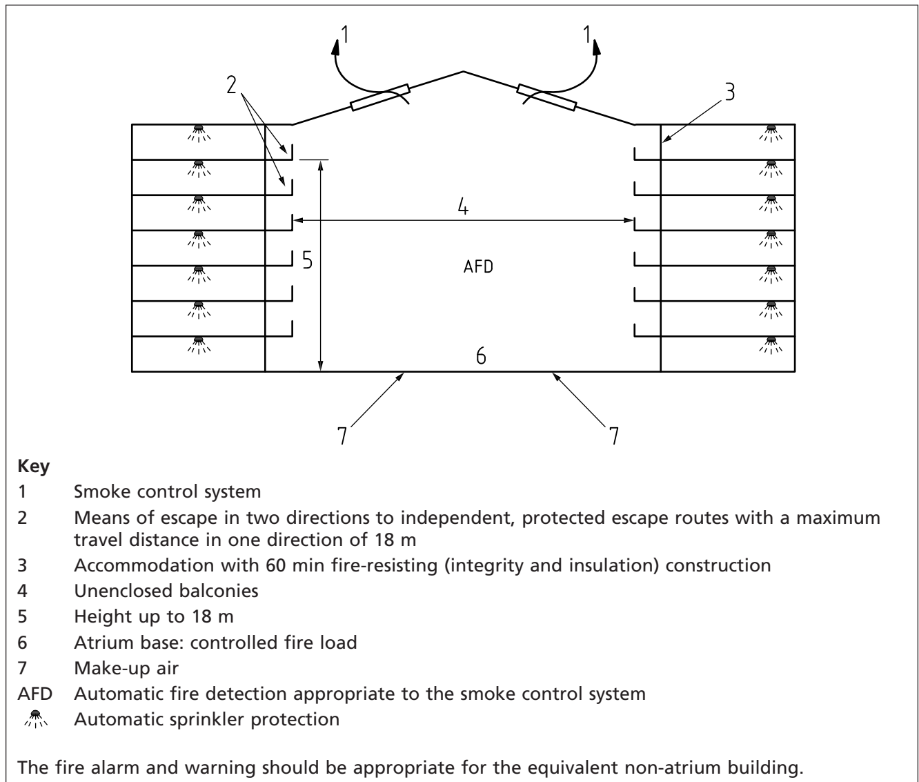
Figure C.7 Exemplar 4: Atrium base: controlled fire load
