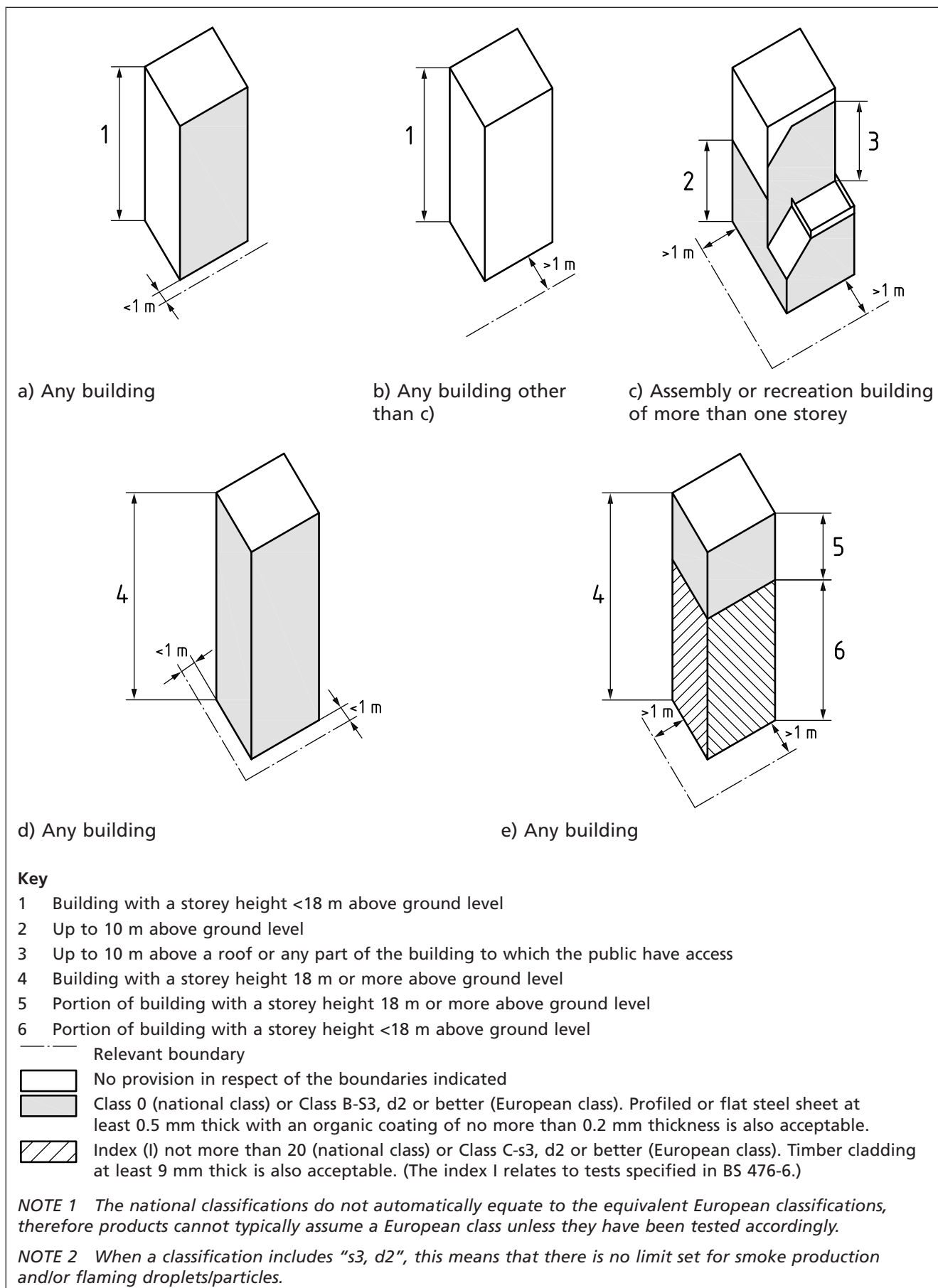
Figure 17 Provisions for external surfaces of walls
