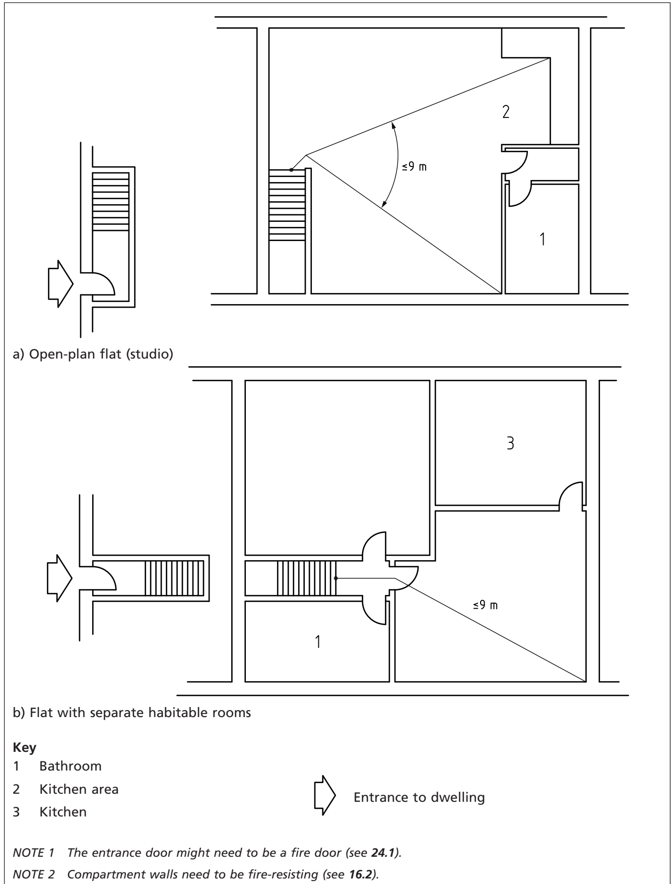
Figure 13 Flat (entered from below) with a restricted travel distance
