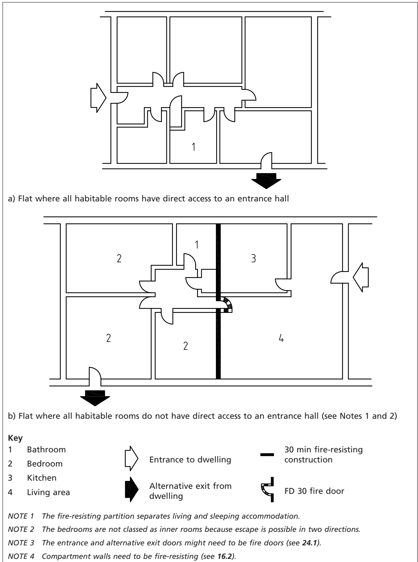
Figure 12 Flat with an alternative exit
