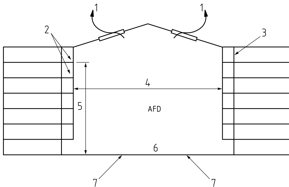
Figure C.4 Exemplar 3a: Atrium base: controlled fire load
