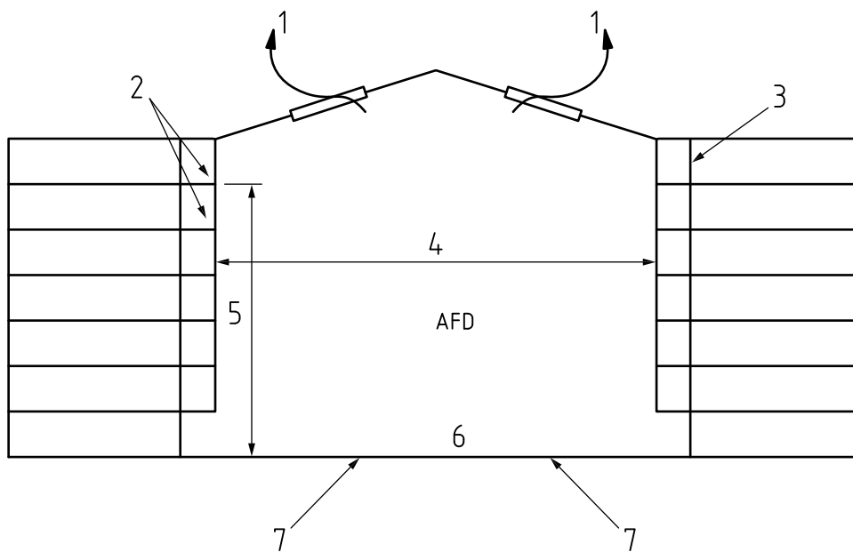
Figure C.5 Exemplar 3b: Atrium base: controlled fire load
