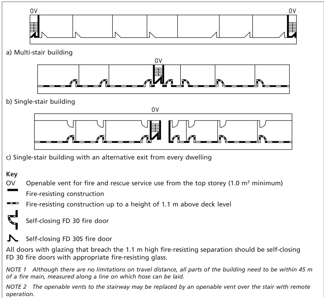
Figure 5 Common escape routes in balcony/deck approach buildings
