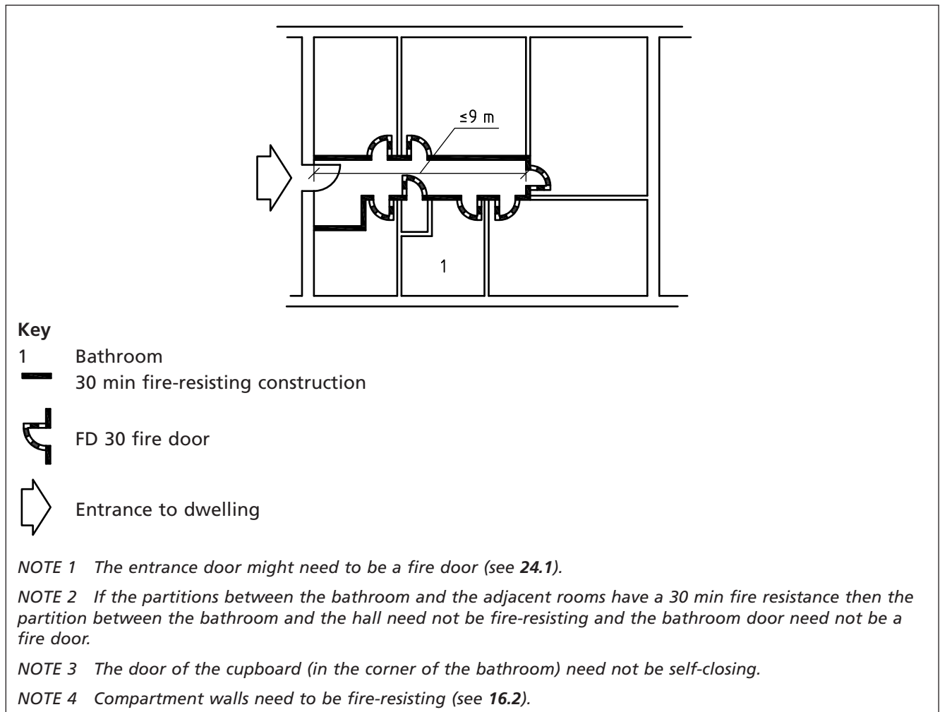
Figure 11 Flat with a protected entrance hall and restricted travel distance
