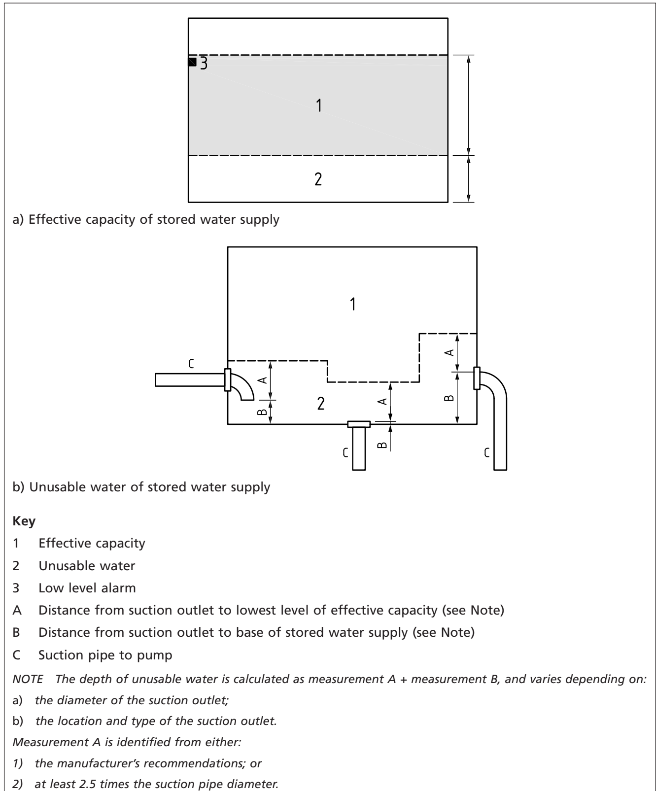
Figure 1 Stored water supply
