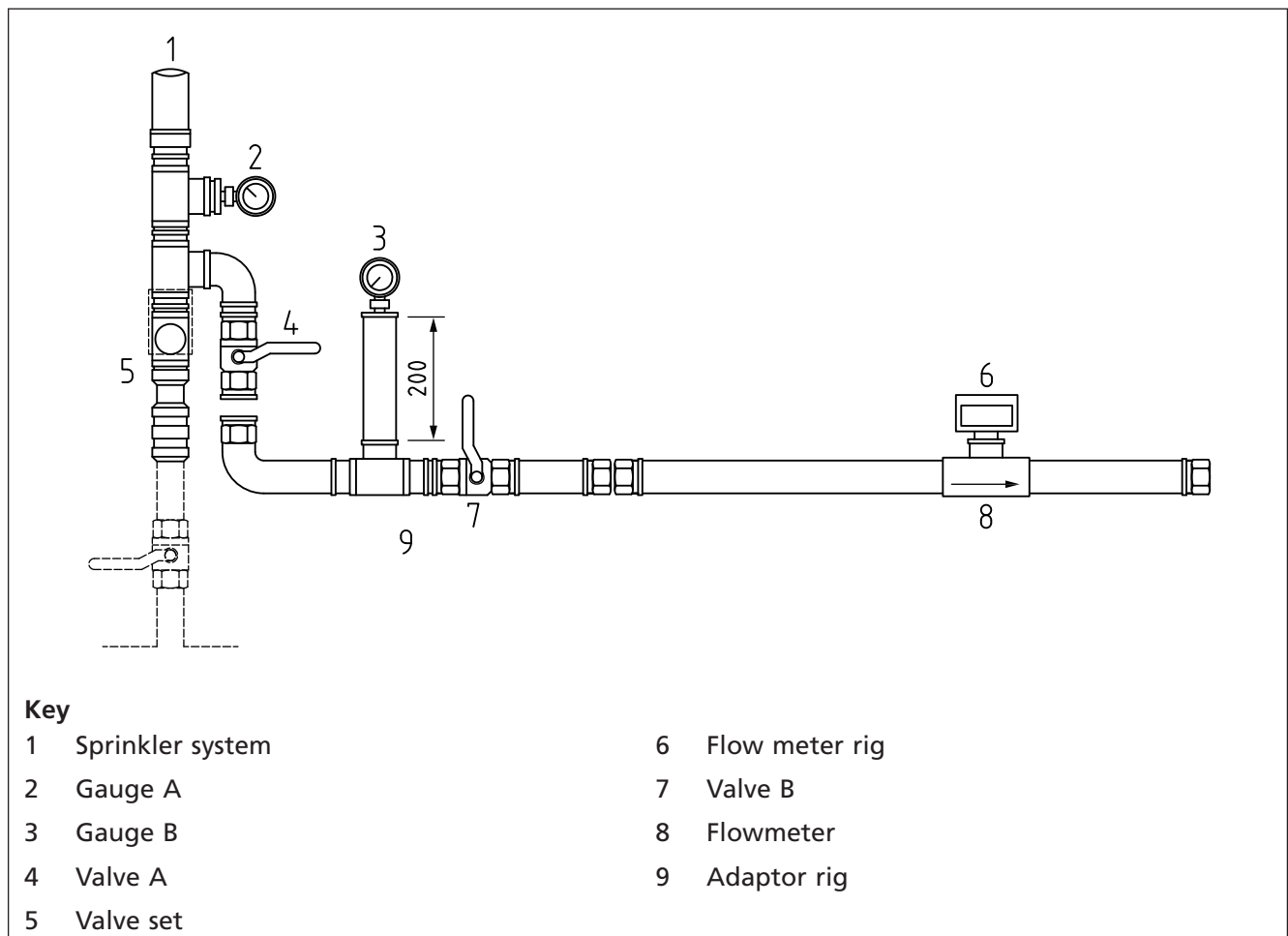
Figure E.1 Test rig for hydraulic test
