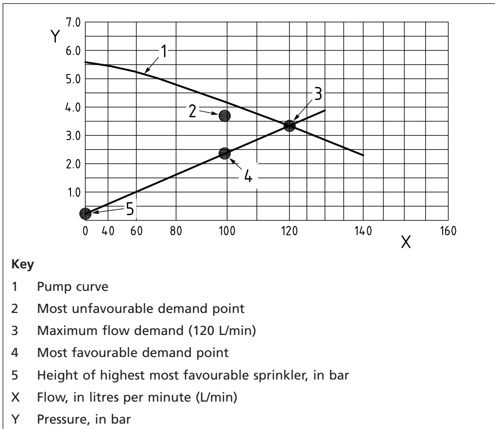
Figure C.1 Example of a square law graduation graph
