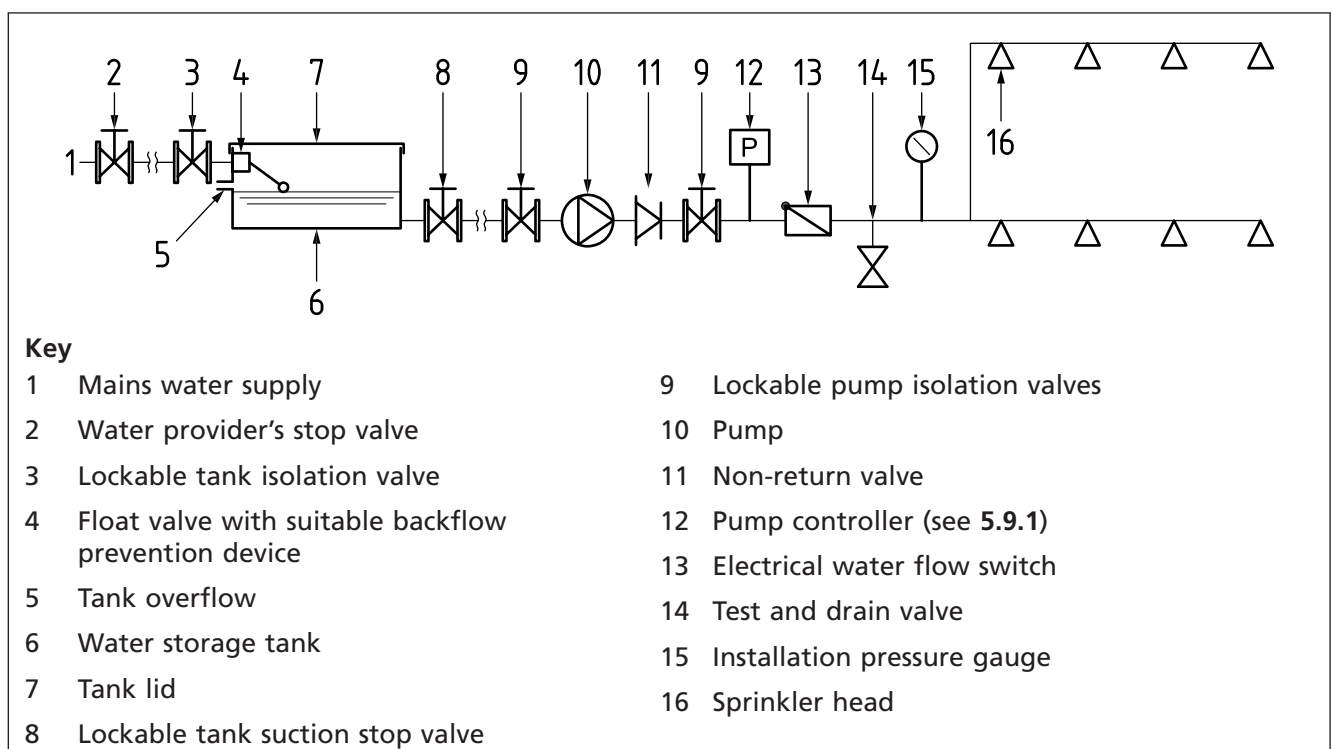
Figure A.2 Elements of a typical pump and tank sprinkler system
