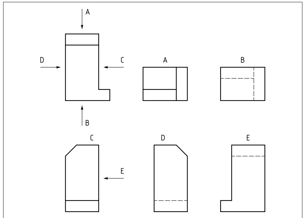
Figure 9 Labelled view method
