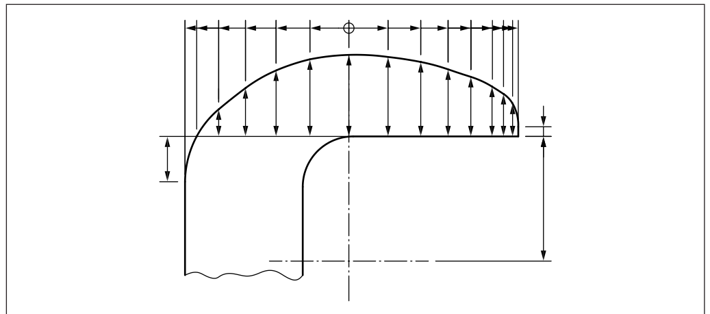
Figure 59 Curved features defined by coordinate dimensions
