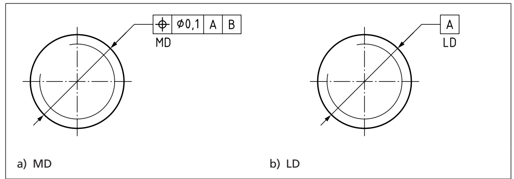
Figure 134 Examples of "MD" and "LD"
