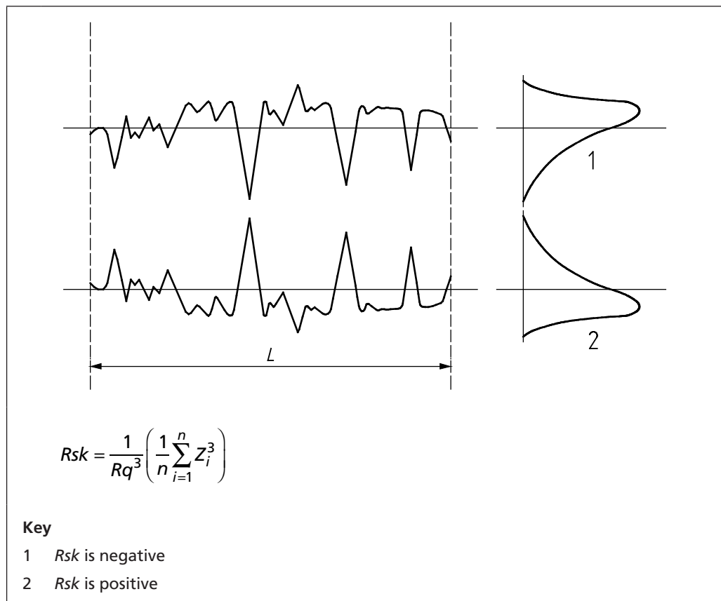
Figure 147 Mathematical derivation of surface skewness ( R_{sk} )
