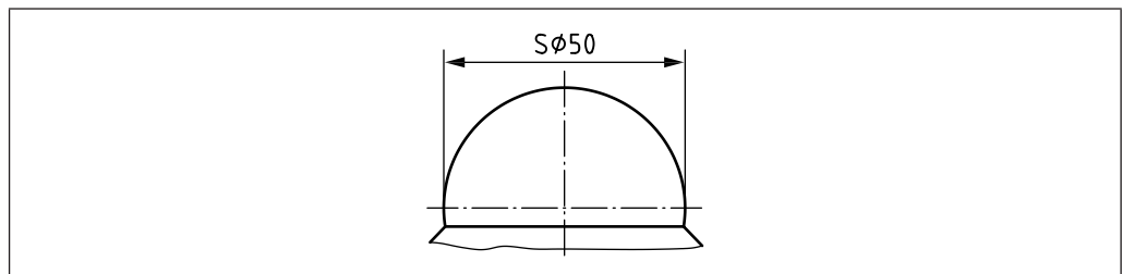
Figure 35 Indications of special dimensions: Spherical diameter
