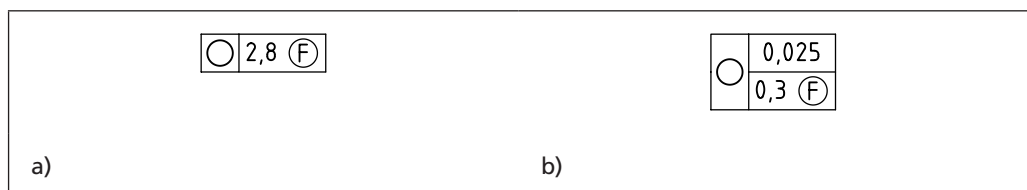
Figure 142 Free state condition
