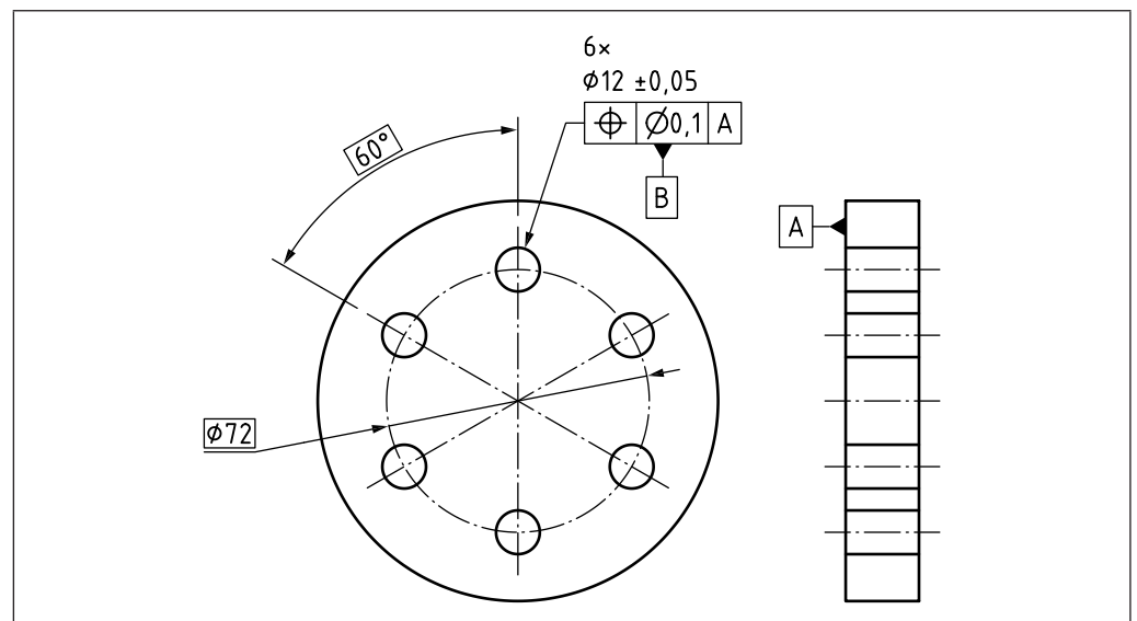
Figure 95 Common datum established by a group of identical features
