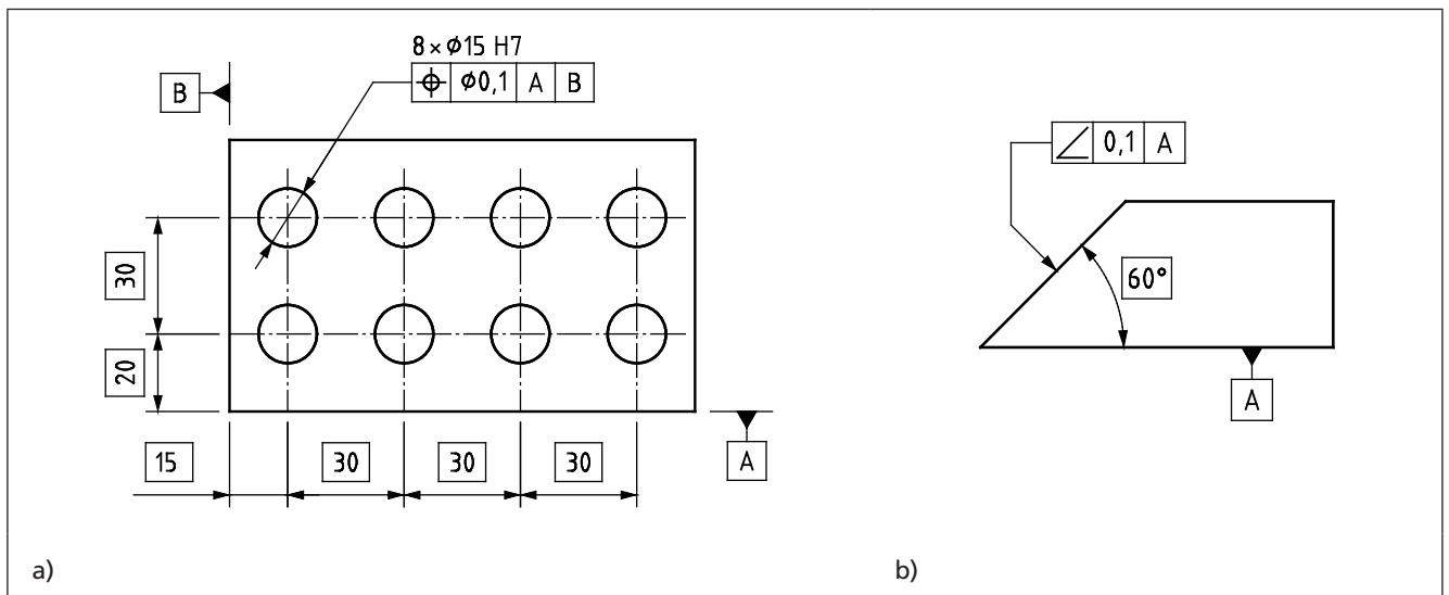
Figure 135 Use of theoretically exact dimensions (TEDs)
