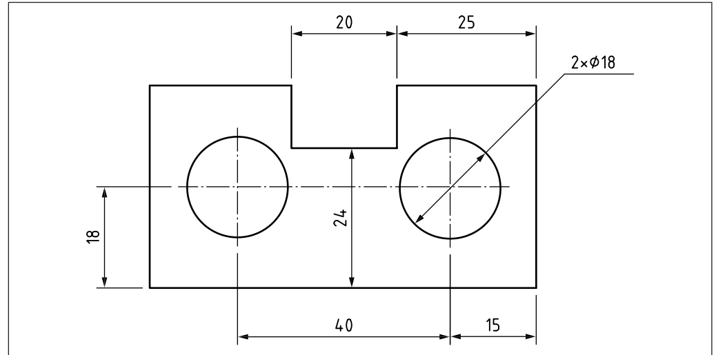
Figure 23 Dimension lines of holes
