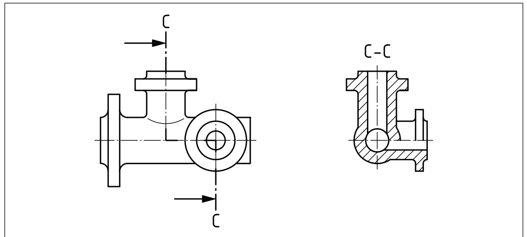
Figure 16 Section view in two parallel planes
