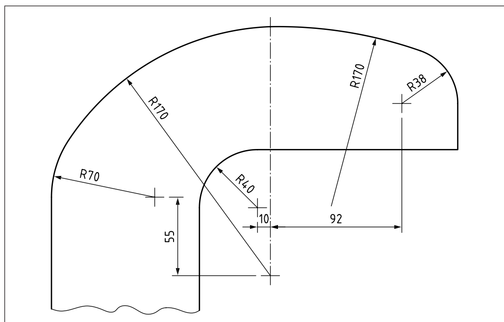
Figure 56 Example of curved feature defined by radii
