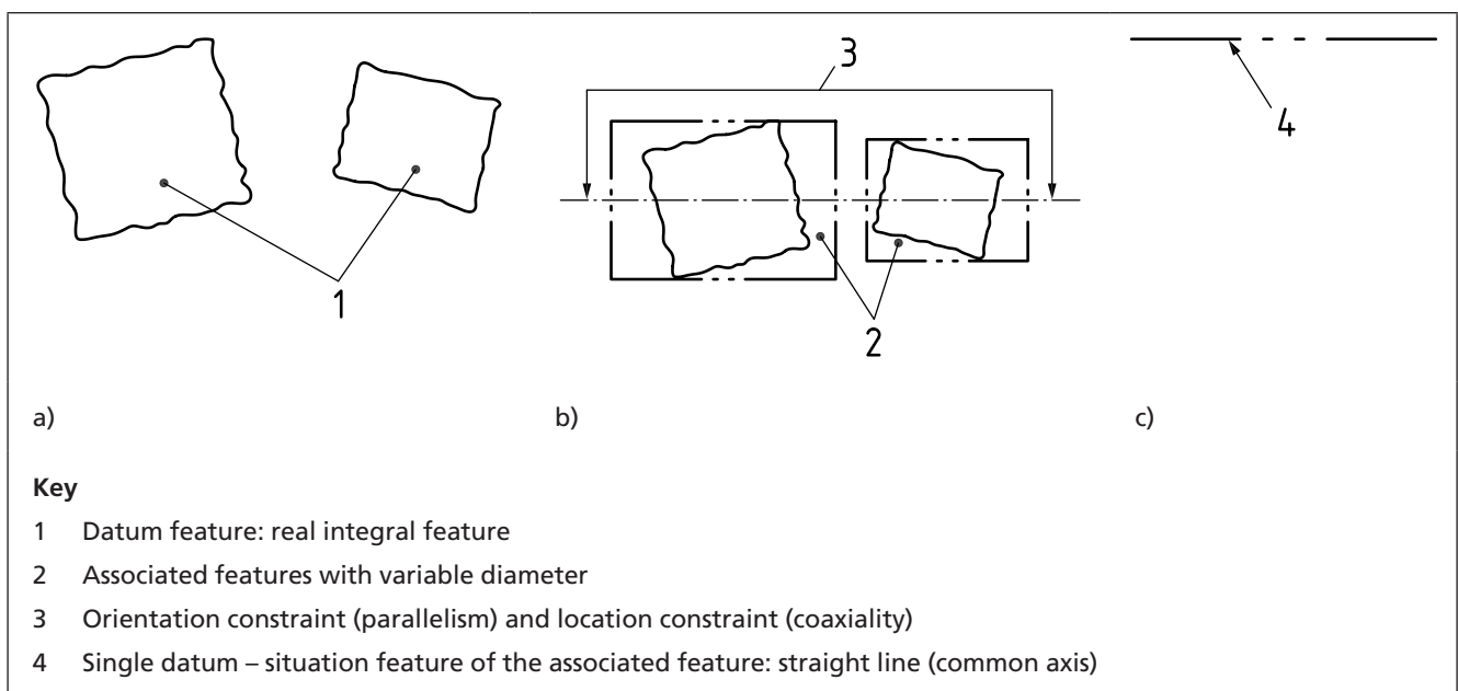
Figure 97 Establishing a common datum from two coaxial cylinders
