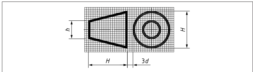
Figure 11 First angle projection method: Graphical symbol
