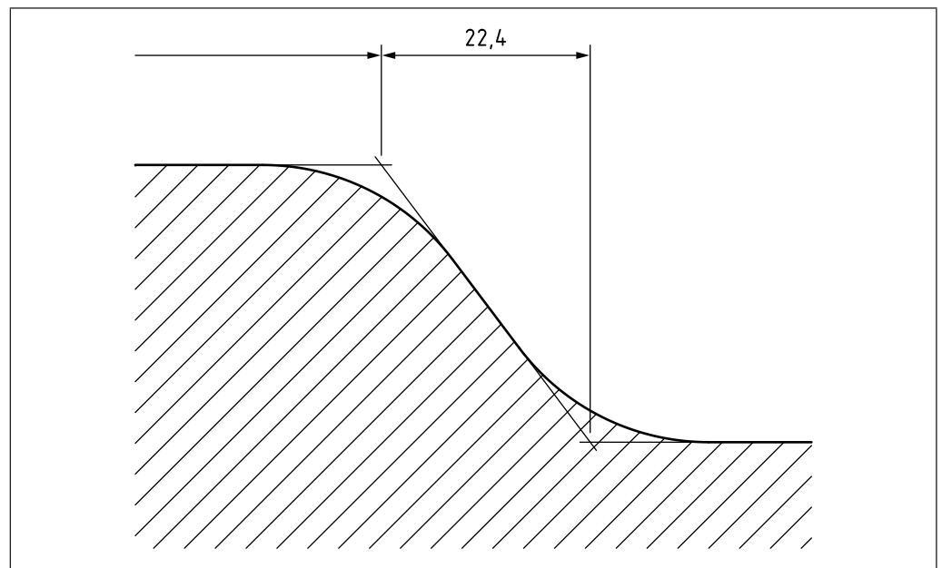
Figure 27 Intersection of projected contours of transitions and similar features
