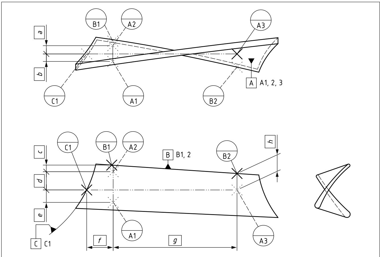
Figure 115 Application of datum targets
