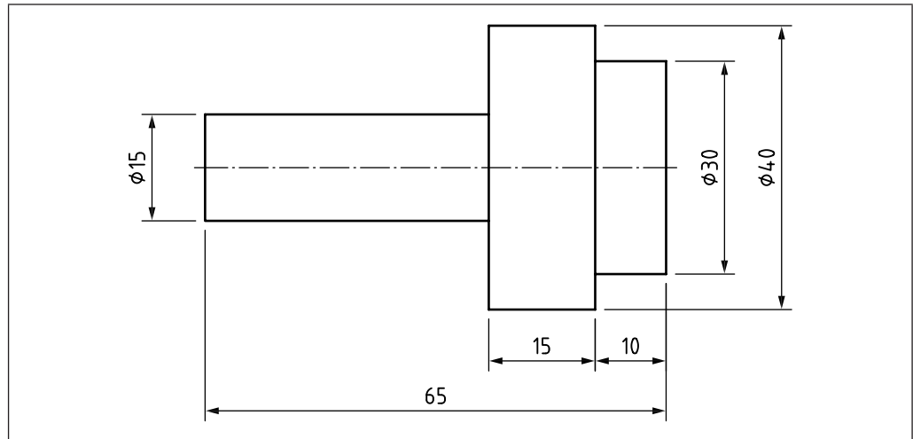
Figure 29 Position of dimensional values
