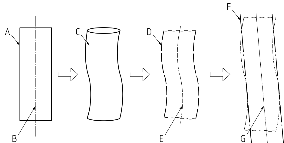
Figure 2 Interrelationship of the geometrical feature definitions
