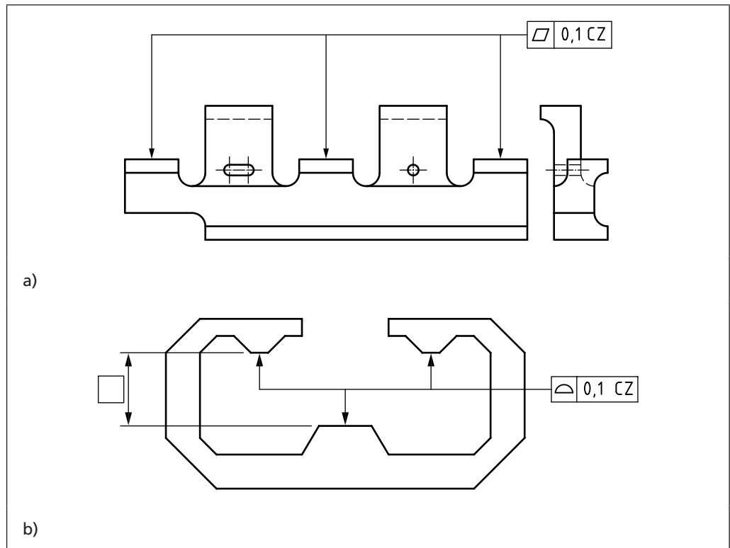
Figure 131 Single tolerance zone applied to separate features
