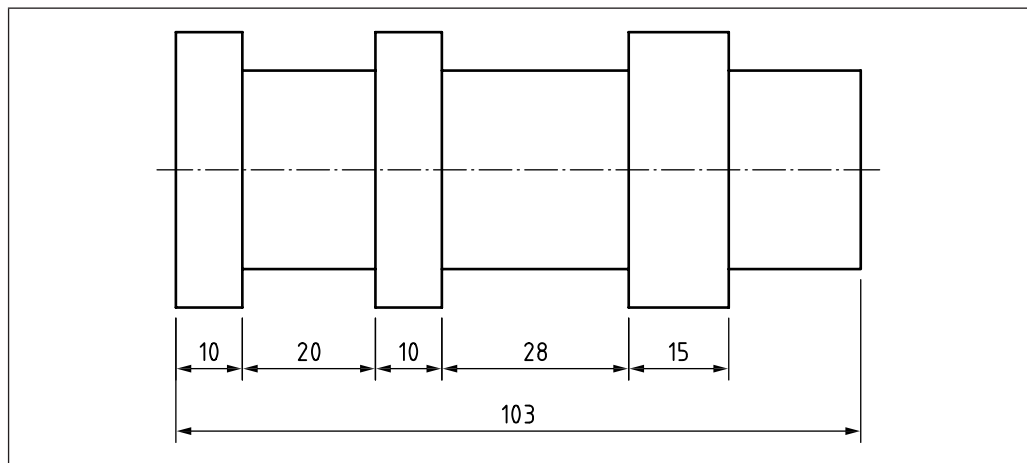
Figure 60 Example of chain dimensioning
