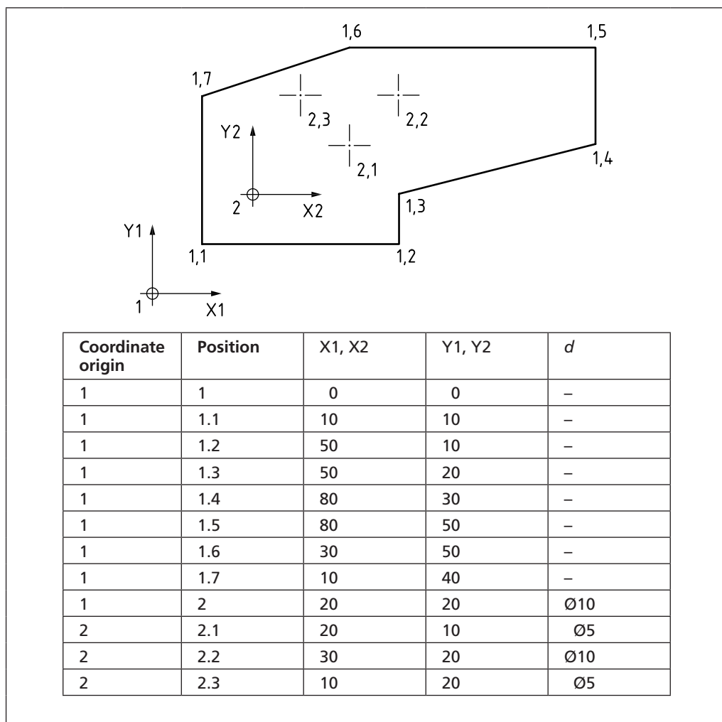
Figure 66 Cartesian coordinate dimensioning
