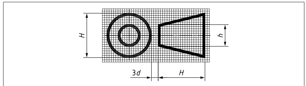
Figure 13 Third angle projection method: Graphical symbol
