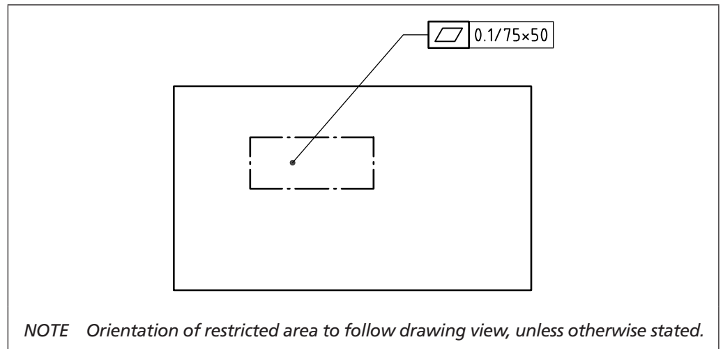
Figure 138 Tolerance applied to an area
