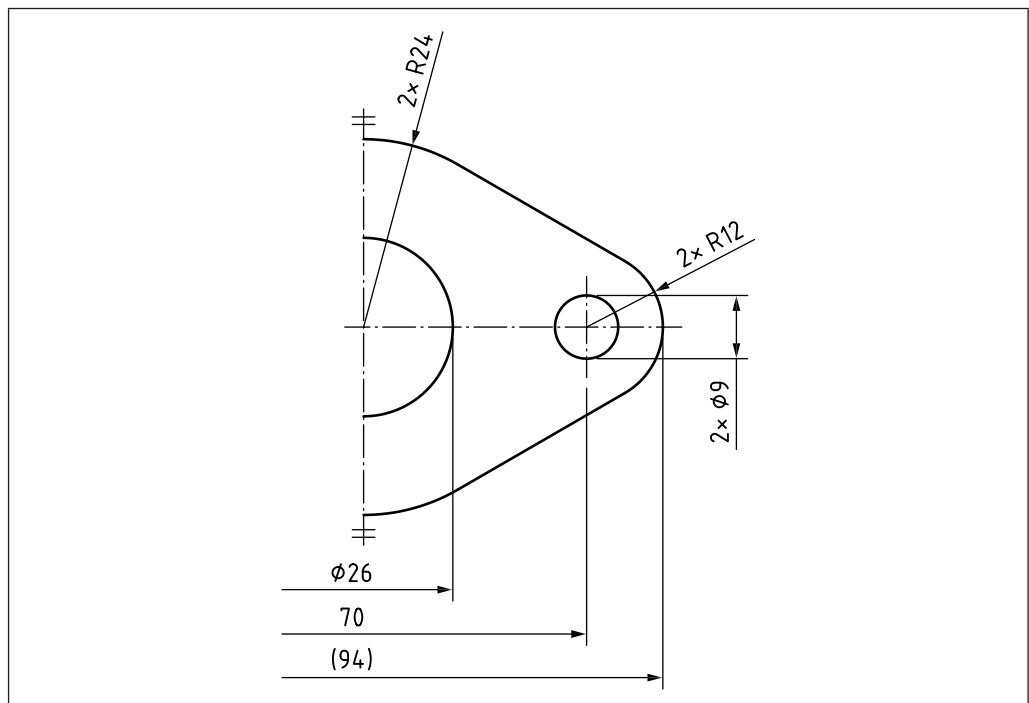
Figure 51 Symmetrical parts
