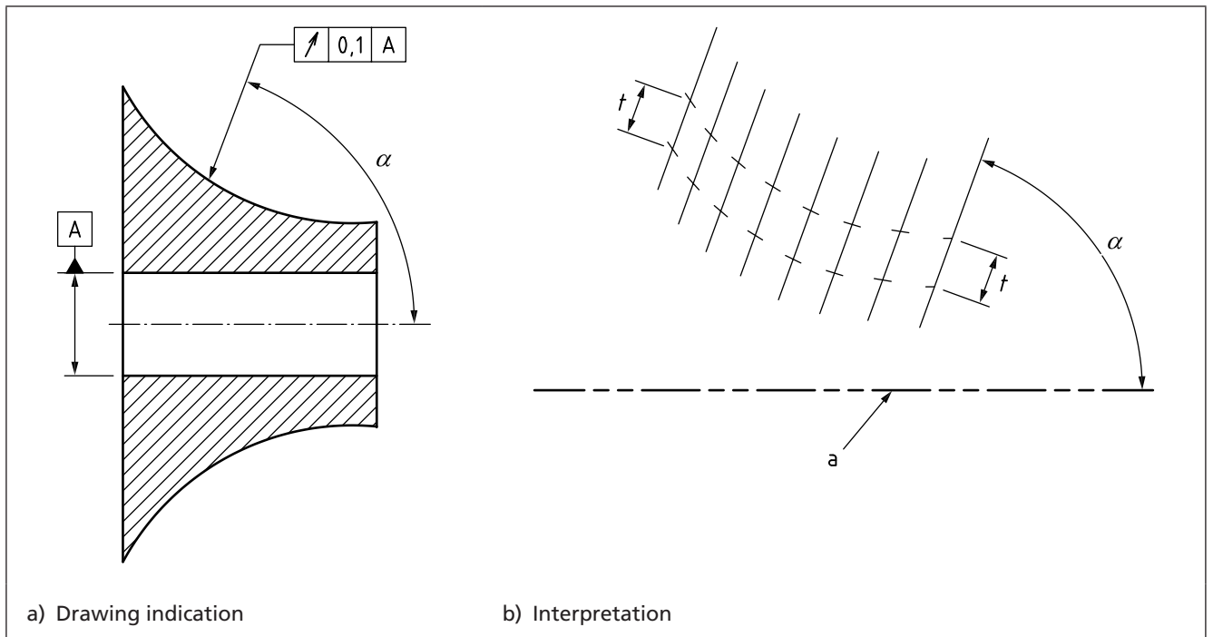
Figure 125 Width of tolerance zone, otherwise indicated
