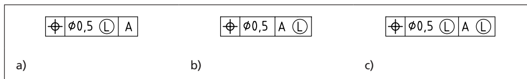
Figure 141 Indication of the least material requirement
