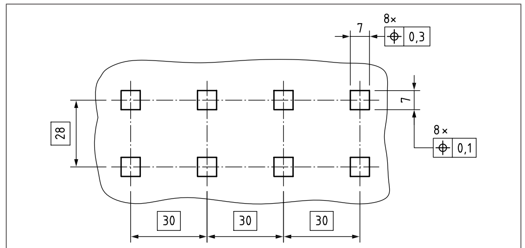
Figure 126 Orientation of the width of a positional tolerance zone
