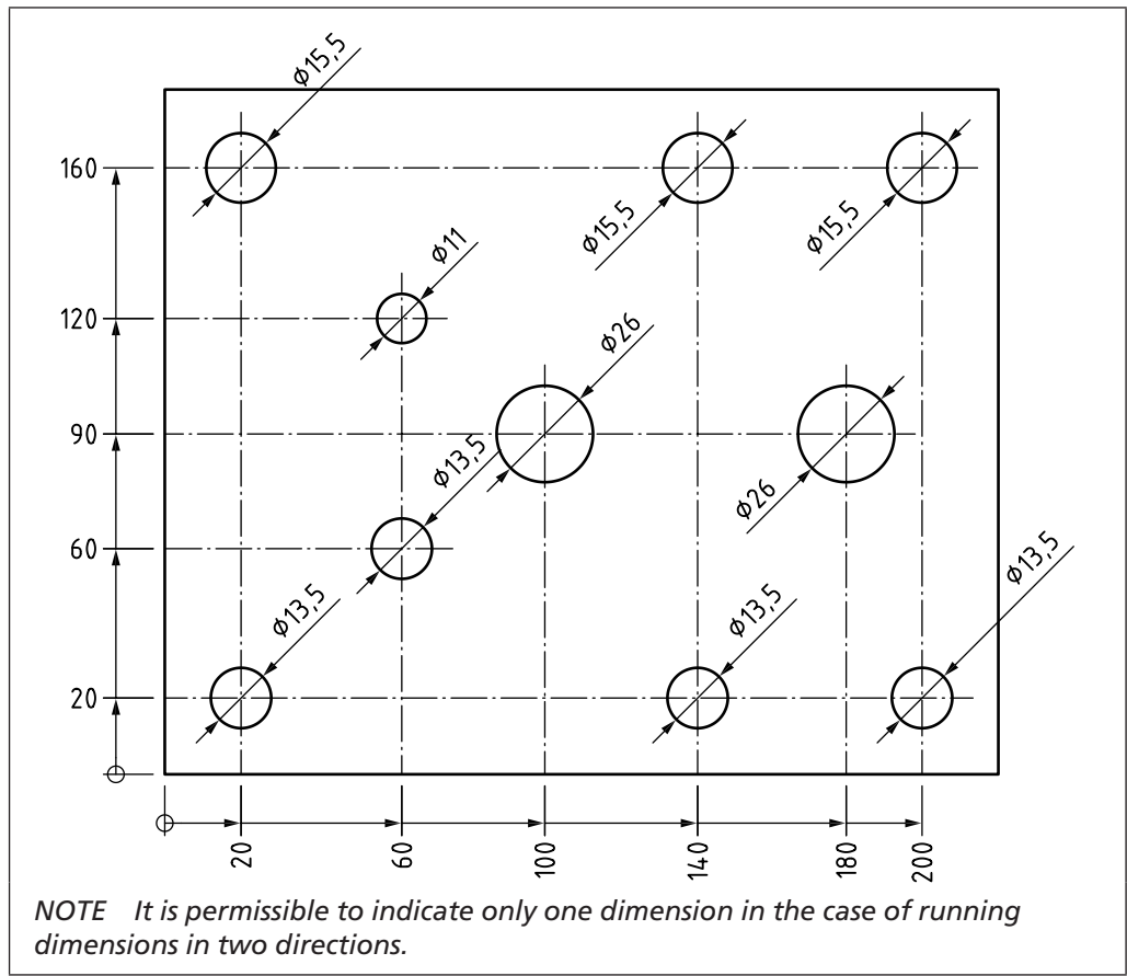
Figure 63 Two dimension lines, inclined to each other, and two origins
