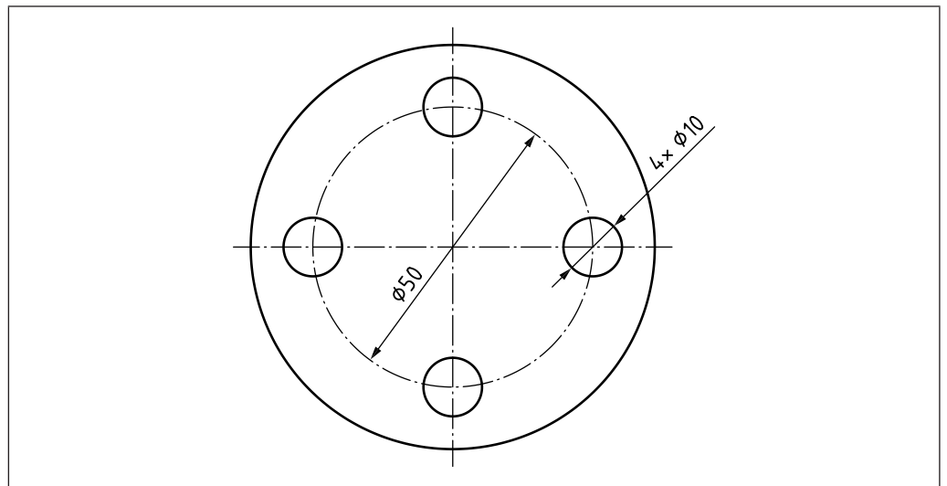
Figure 42 Angles of spacings
