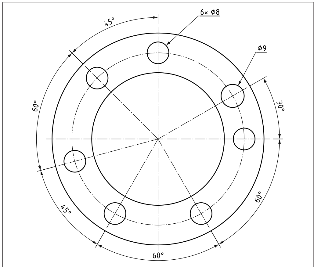
Figure 44 Indication of features having the same dimensional value
