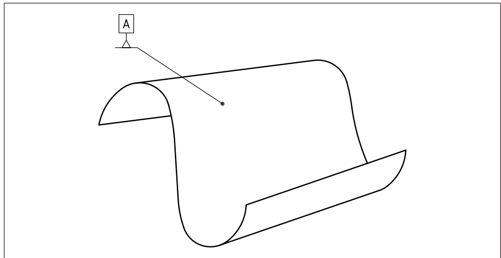
Figure 88 Datum for prismatic feature
