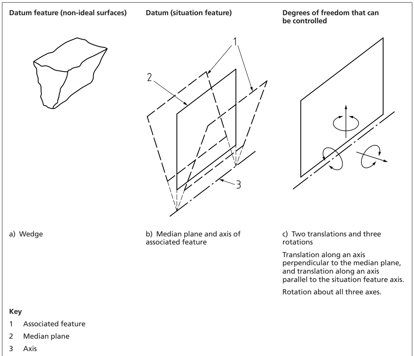
Figure 87 Datum feature consisting of a non-ideal wedge
