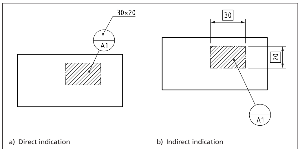
Figure 110 Direct and indirect indication for single datum target area
