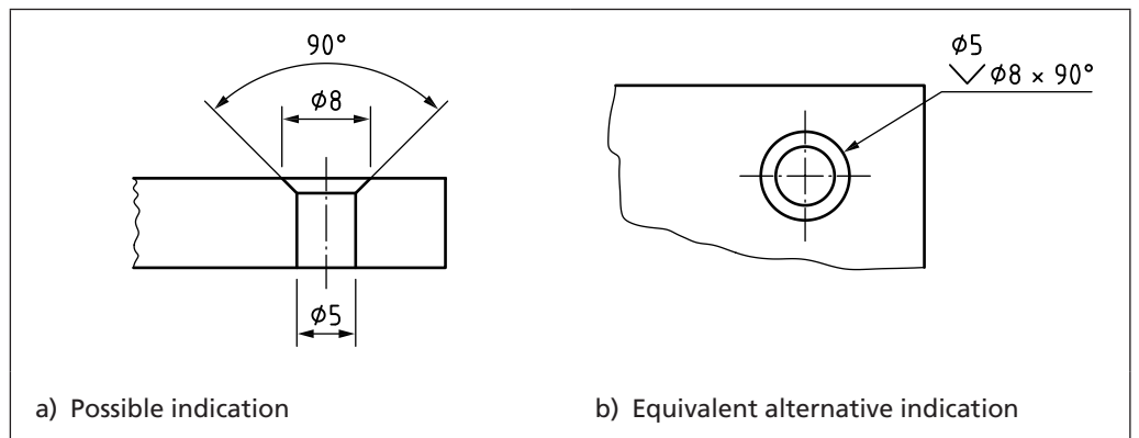
Figure 39 Size and angle of countersink
