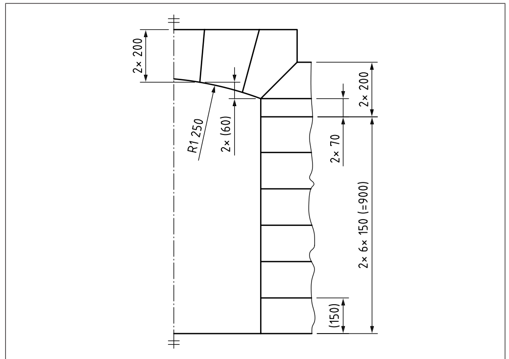
Figure 52 Symmetrical parts
