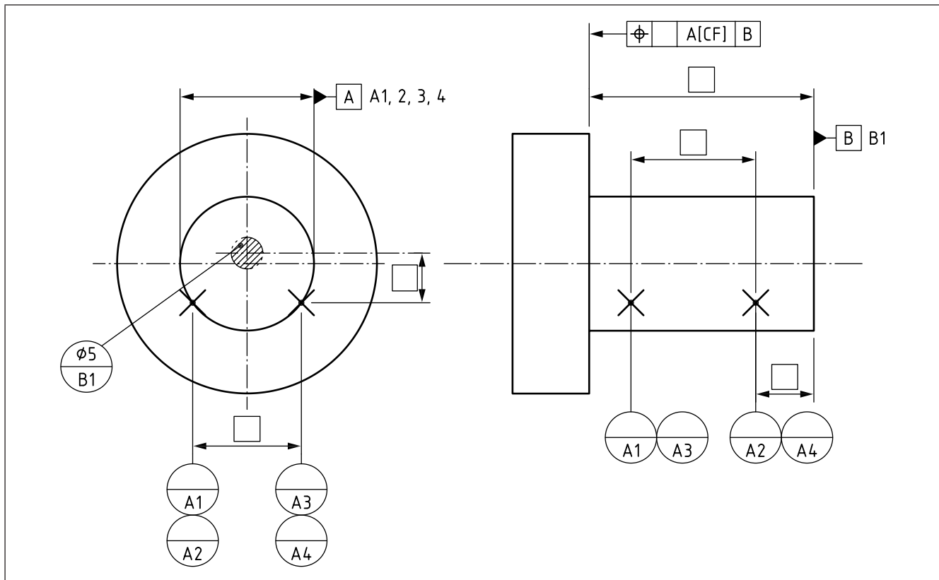
Figure 113 Datums based on more than one datum target
