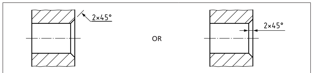
Figure 48 Dimension of internal chamfer equal to 45°
