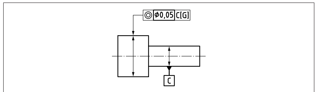
Figure C.1 Example of individual specification operator for a datum association
