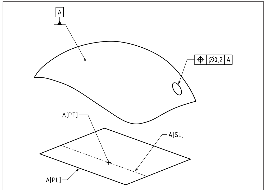
Figure E.1 Implementation according to BS 8888 and BS EN ISO 5459
