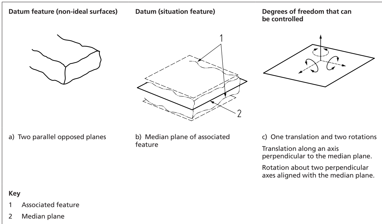
Figure 83 Datum based on two parallel, opposed planes
