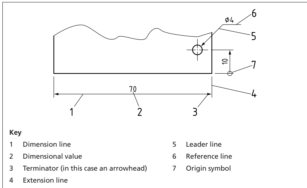
Figure 21 Elements of dimensioning
