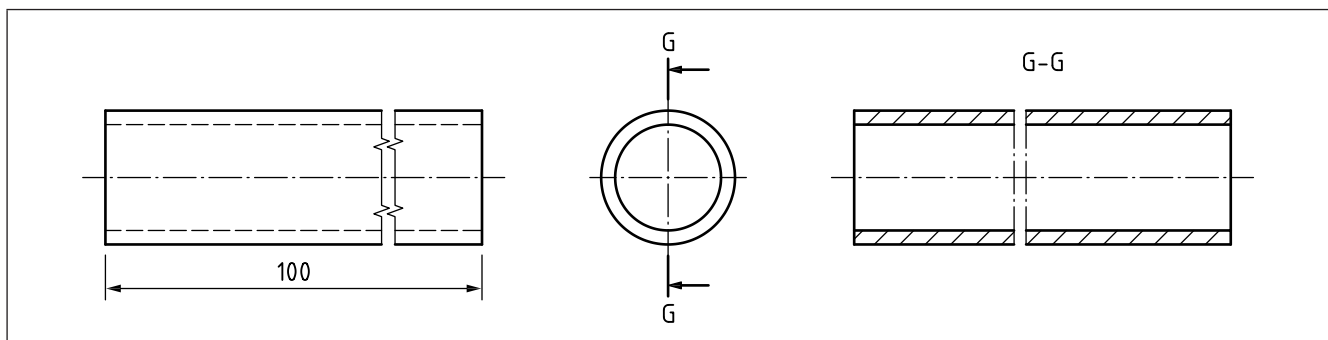
Figure 22 Dimension line of feature that is broken
