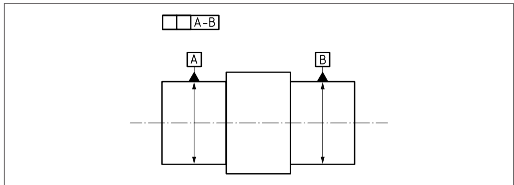
Figure 96 Common datum established from two coaxial cylinders
