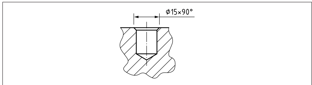
Figure 50 Dimension of countersink: simplification
