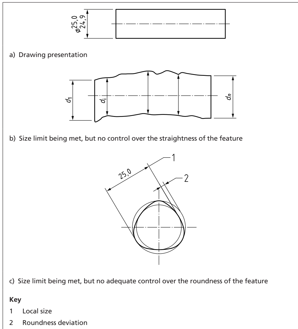
Figure 3 Possible interpretations of size limits where no form control is defined and the specification is incomplete
