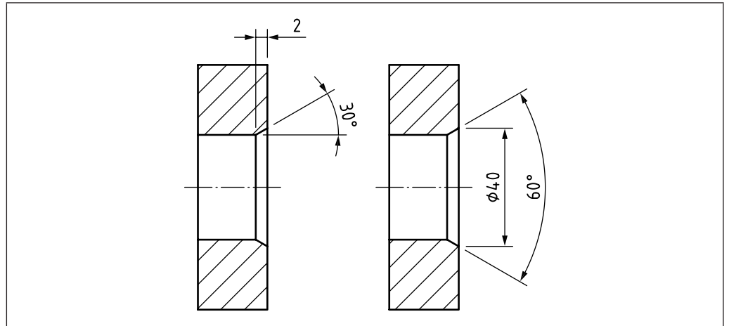
Figure 47 Dimension of internal chamfer not equal to 45°
