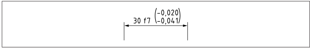
Figure 68 Example: expression of two deviations to the same number of decimal places
