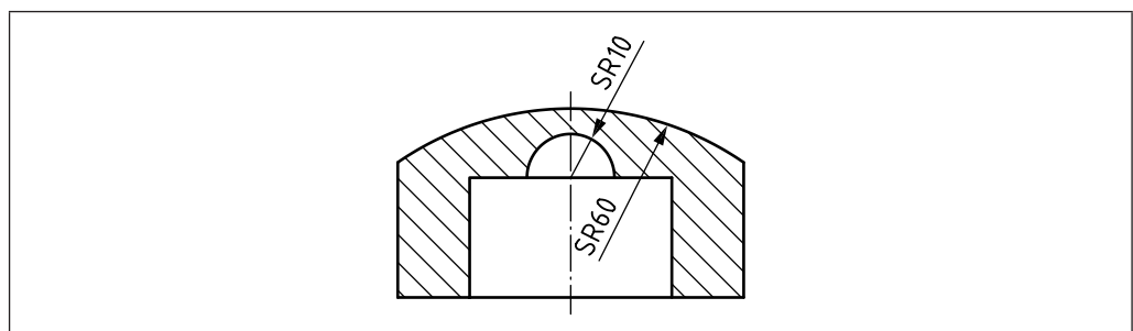
Figure 36 Indications of special dimensions: Spherical radius
