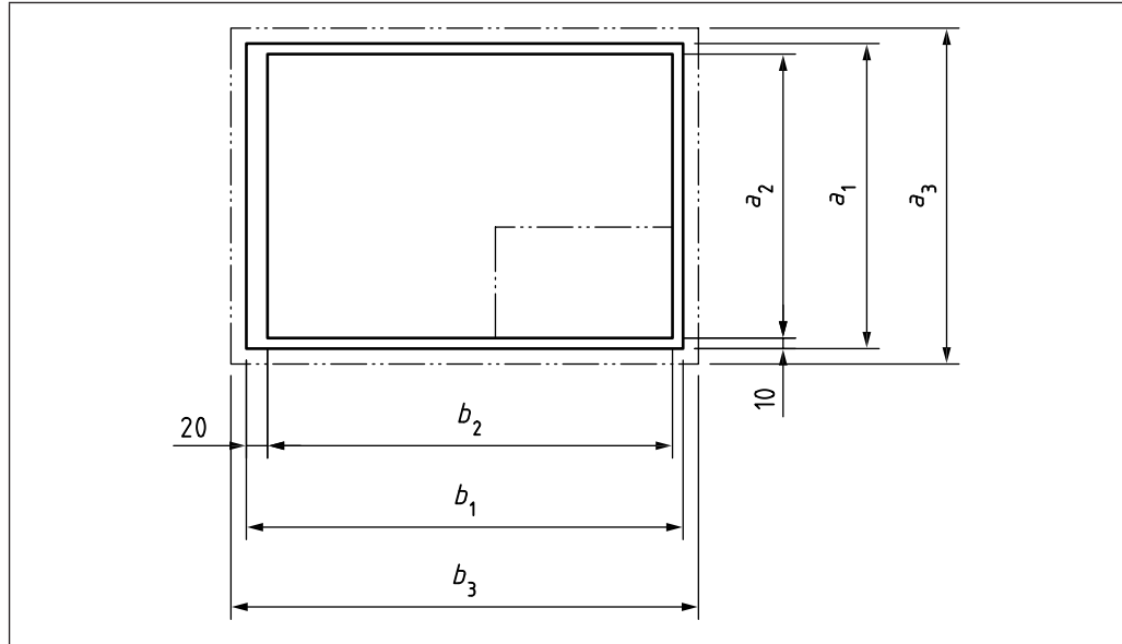
Figure 7 Size A4 to A0
