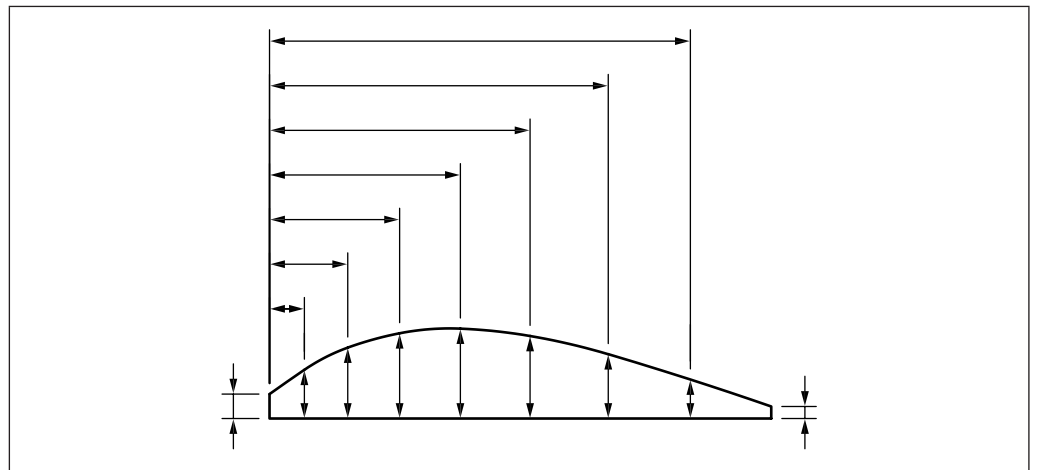
Figure 58 Curved feature defined by coordinate dimensions
