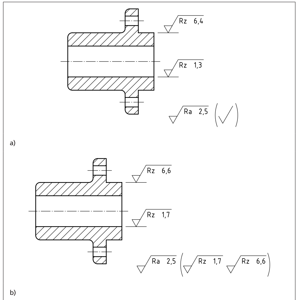
Figure 153 Simplified indication: Majority of surfaces with same surface texture requirement
