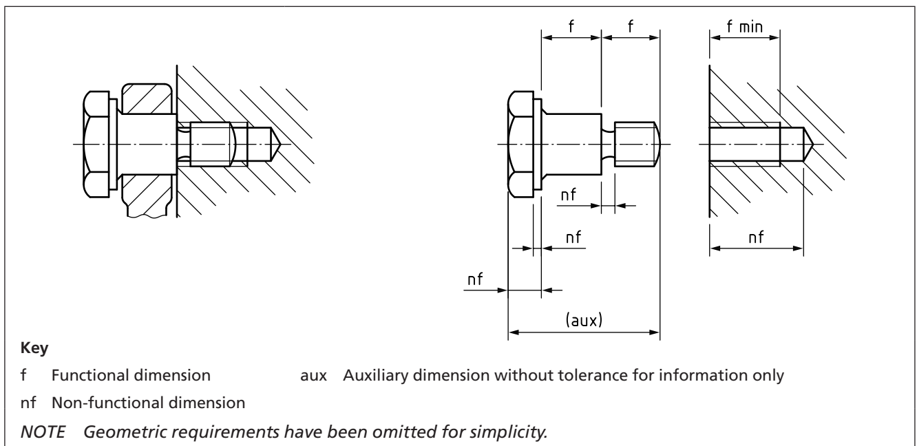
Figure 77 Application of dimensions to suite functional requirements
