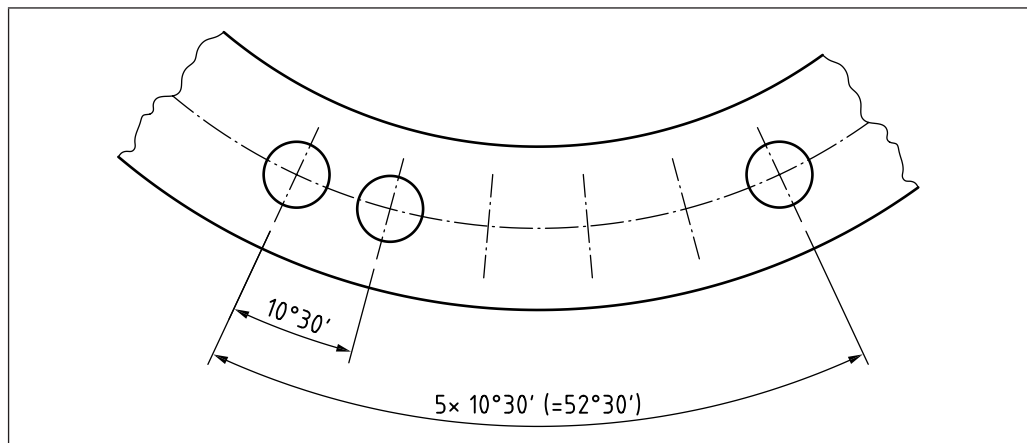
Figure 41 Dimensioning of angular spacing
