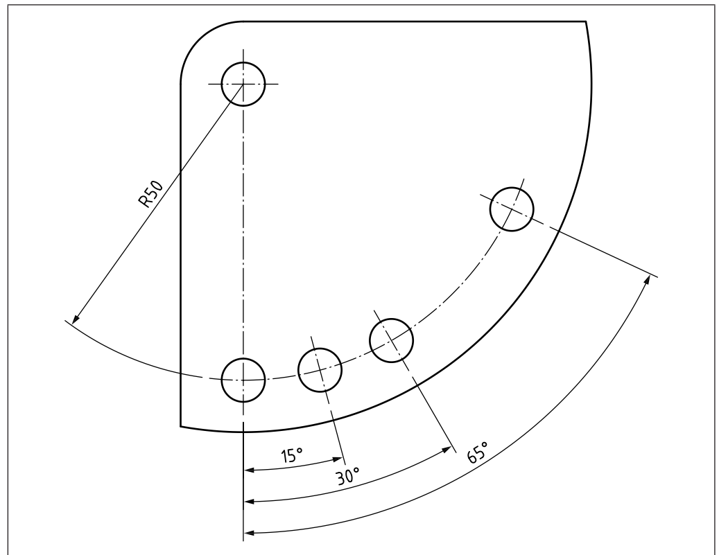
Figure 62 Example of parallel dimensioning
