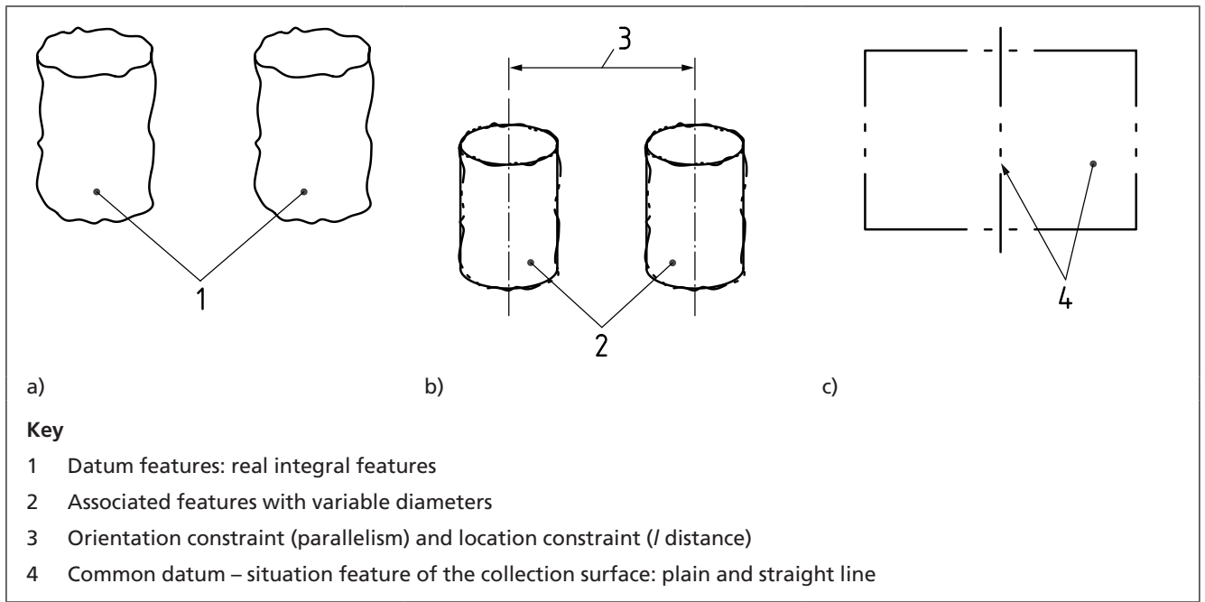
Figure 98 Establishing a common datum from two parallel cylinders
