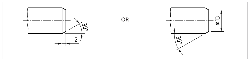
Figure 45 Dimension of external chamfer not equal to 45°
