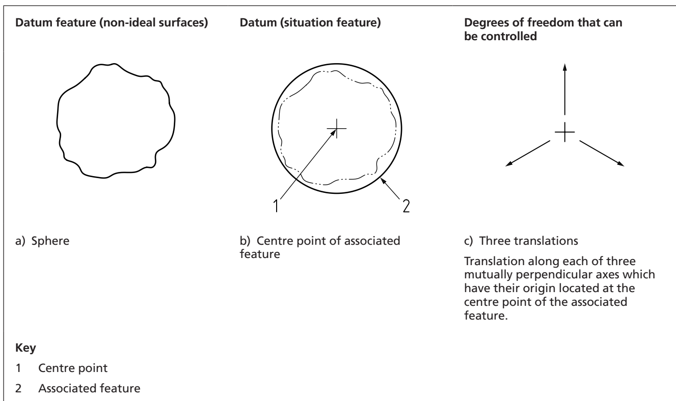
Figure 85 Datum feature consisting of a non-ideal sphere
