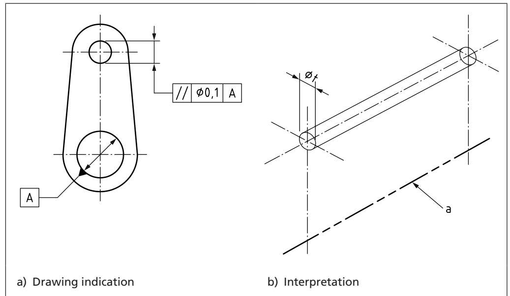
Figure 129 Cylindrical and circular tolerance zones
