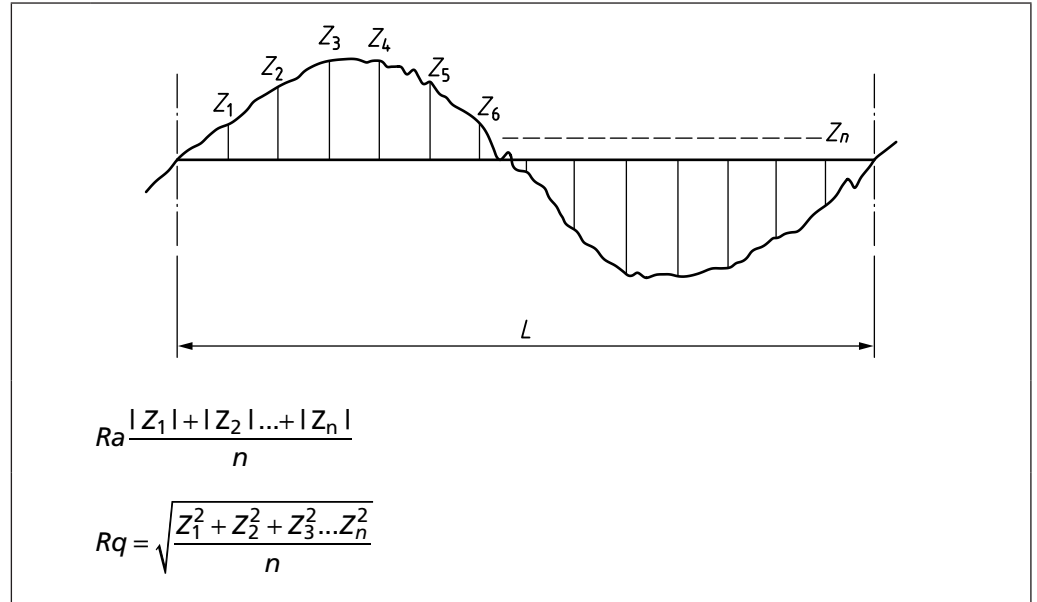
Figure 145 Mathematical derivation of R_a and R_q
