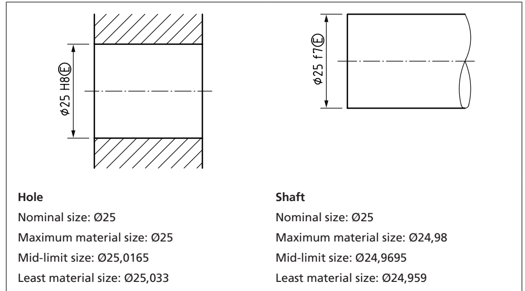
Figure 1 Hole and shaft sizes
