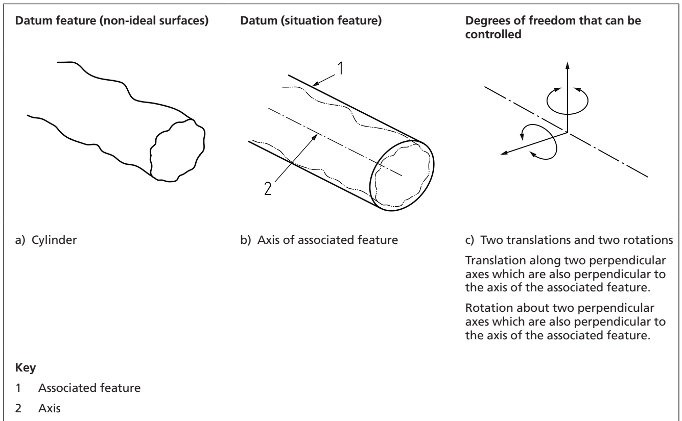
Figure 84 Datum feature consisting of a non-ideal cylinder
