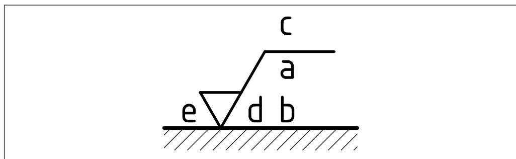
Figure 150 Positions (a to e) for location of texture requirements
