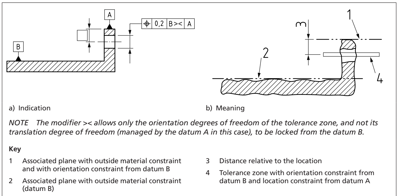
Figure 117 Application of "orientation-only" modifier
