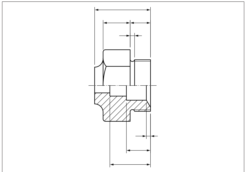
Figure 19 Arrangement and indication of dimensions internal and external features
