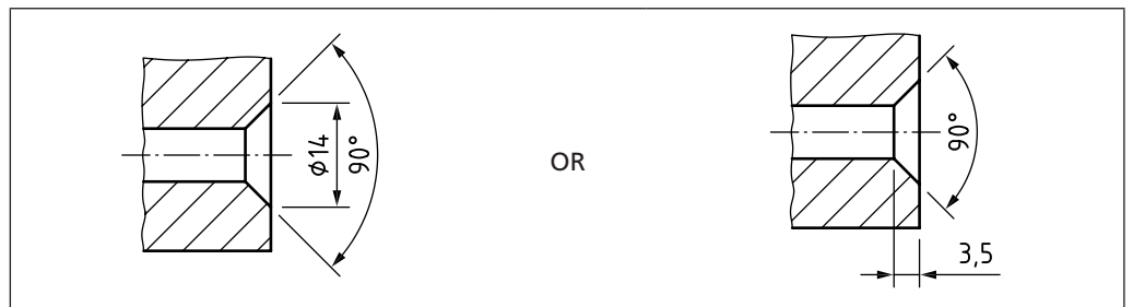
Figure 49 Dimension of countersink
