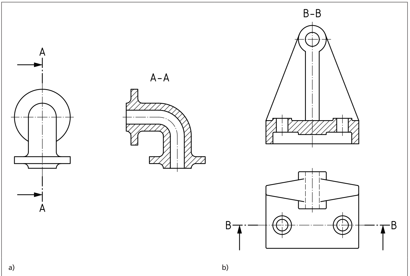
Figure 15 Section view in one plane
