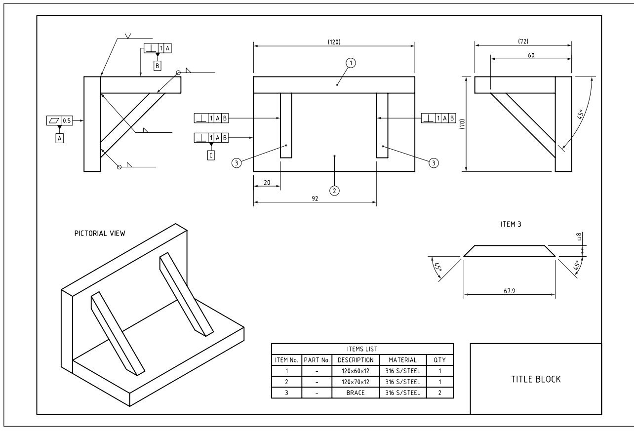
Figure 6 Example of fabrication drawing
