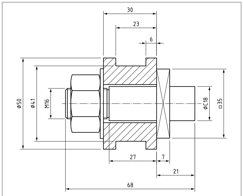
Figure 20 Grouping of relative dimensions of features or objects in close proximity
