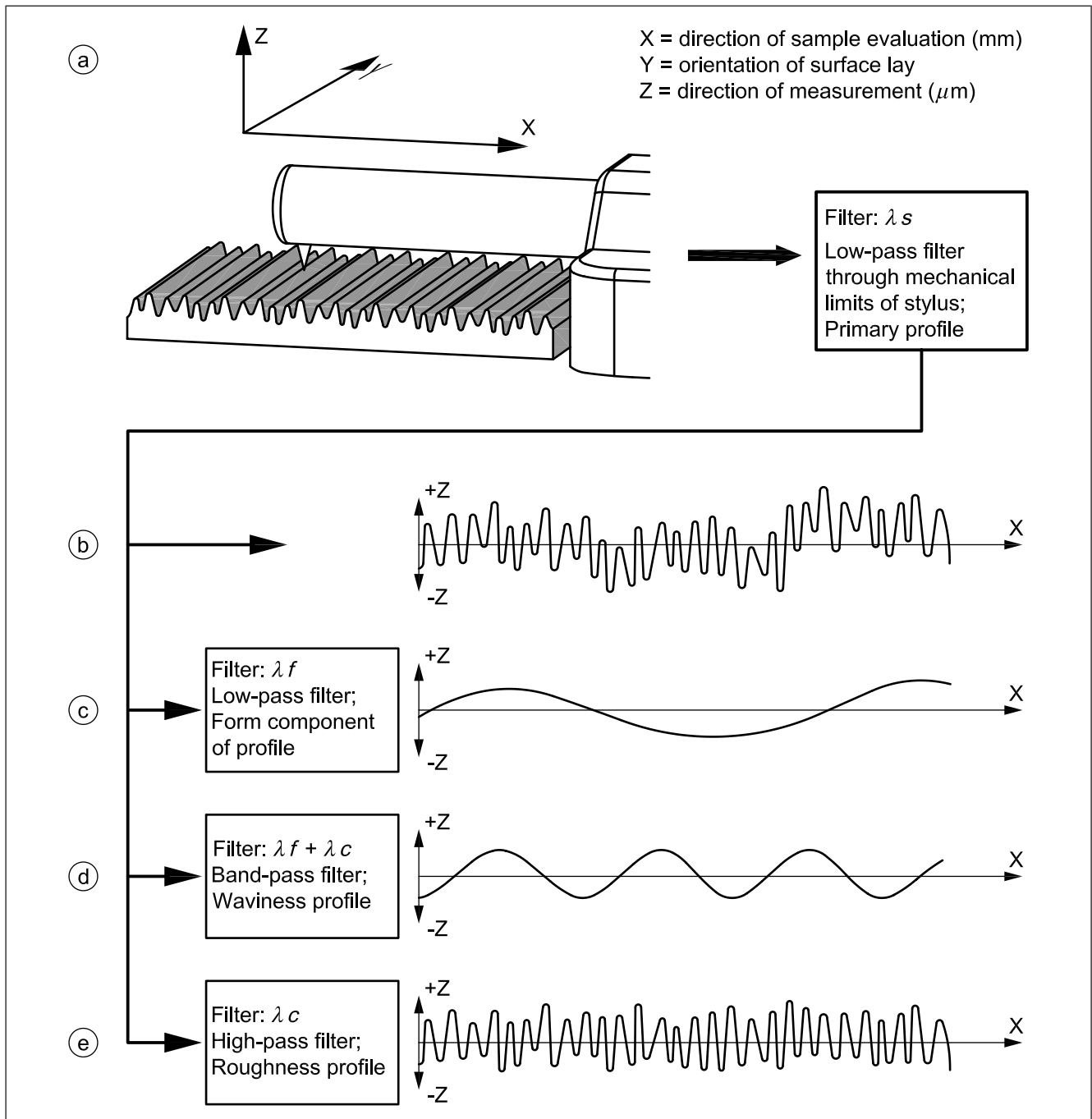
Figure 144 Use of several specification modifiers
