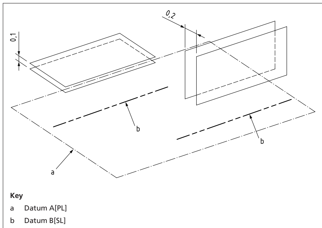
Figure 128 Tolerances perpendicular to each other
