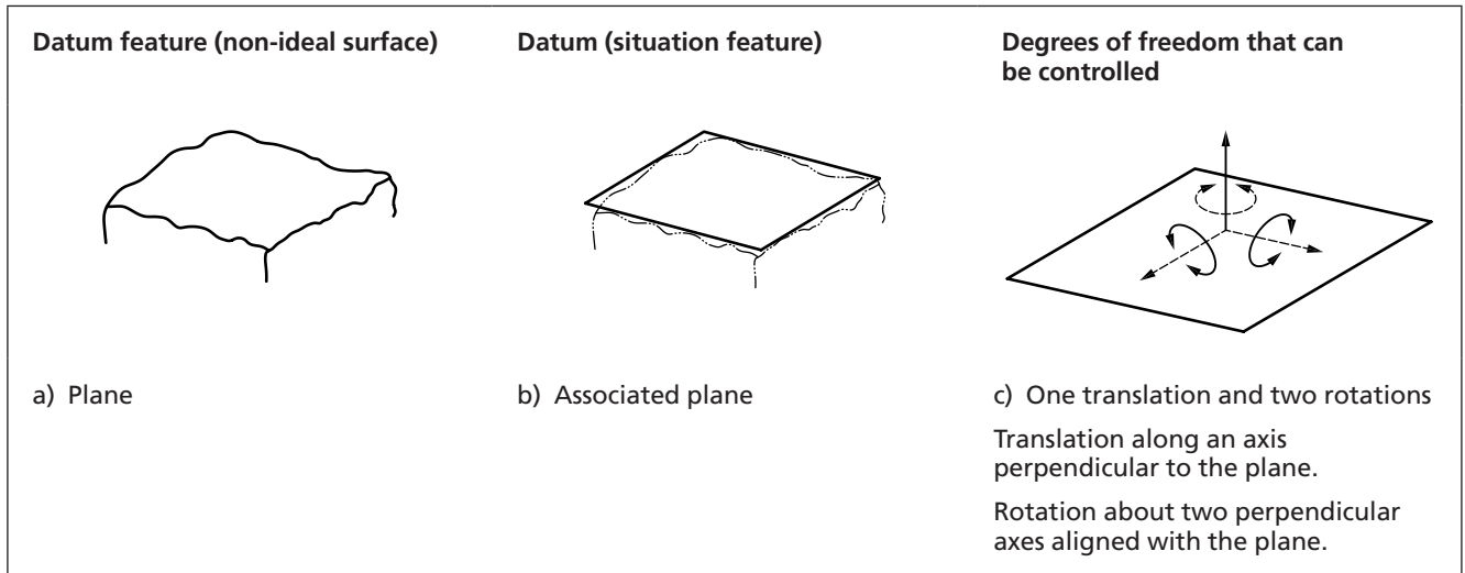
Figure 81 Datum based on a planar datum feature
