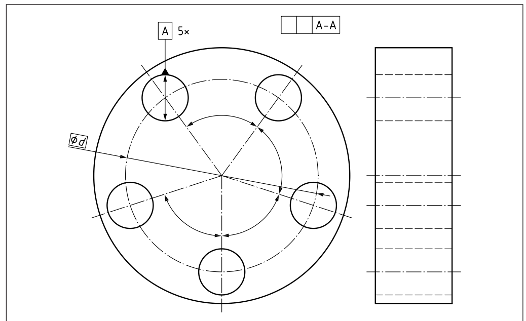
Figure 99 Pattern of five cylinders: input for reading (drawing indication) and for writing (design intent)
