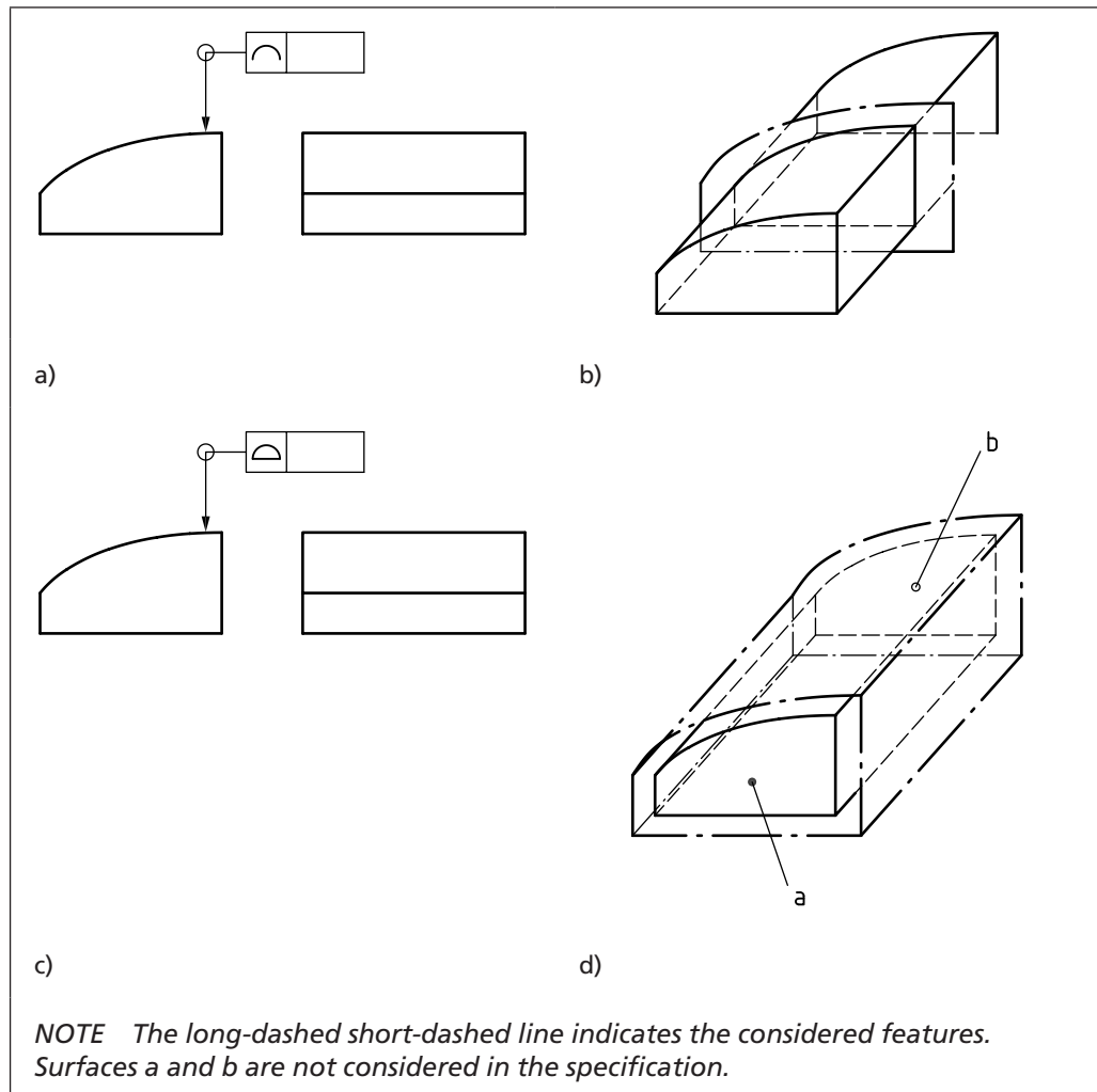
Figure 133 Examples of the use of the “all around” symbol
