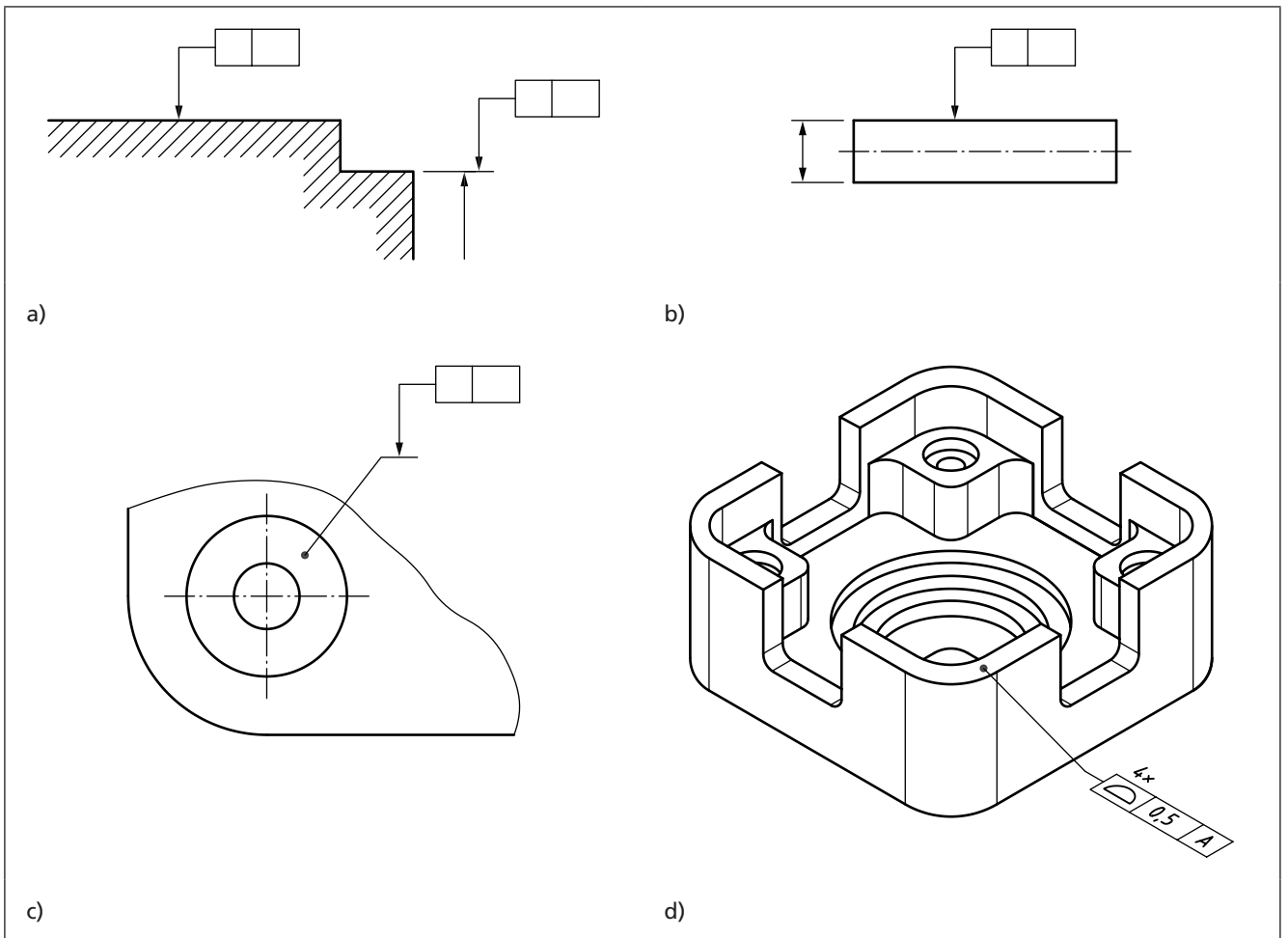
Figure 122 Terminator on the outline or the surface of a feature or as an extension
