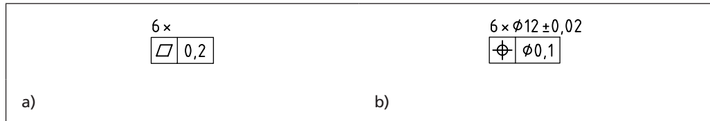
Figure 119 Tolerance applying to more than one feature
