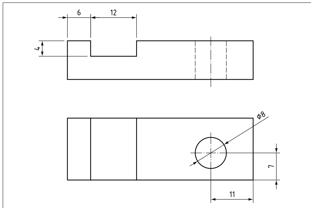
Figure 18 Positioning of dimensions
