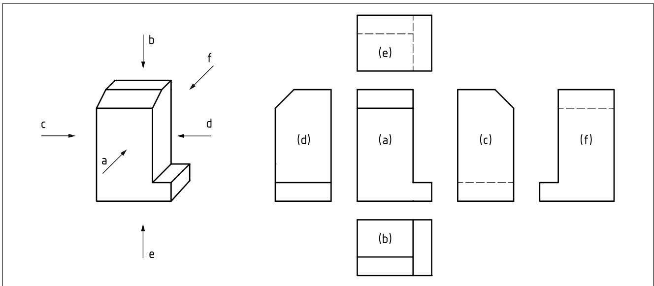
Figure 10 First angle projection method
