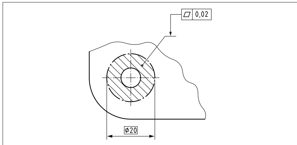
Figure 137 Tolerance applied to a restricted part of a feature
