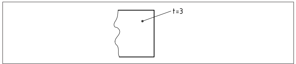
Figure 37 Indications of special dimensions: Thickness
