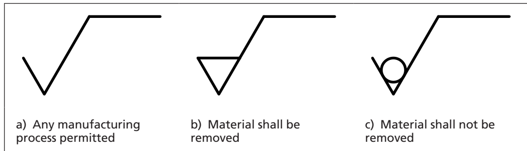
Figure 149 Surface texture graphical symbol
