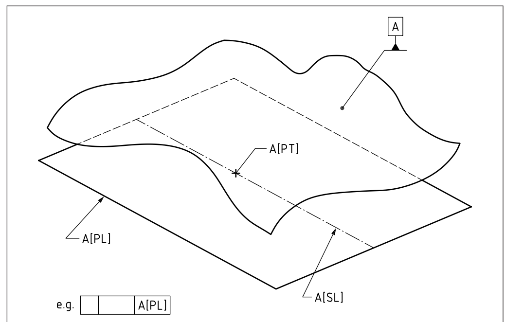
Figure 94 Example identifiers for situation features
