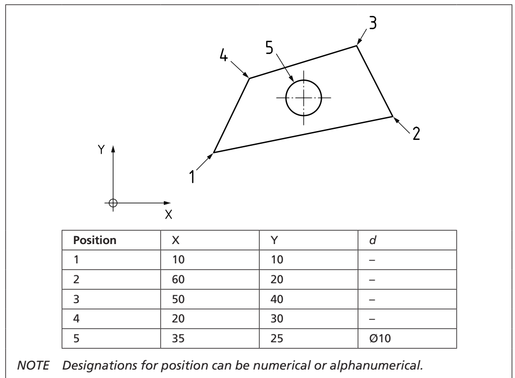
Figure 65 Cartesian coordinate dimensioning
