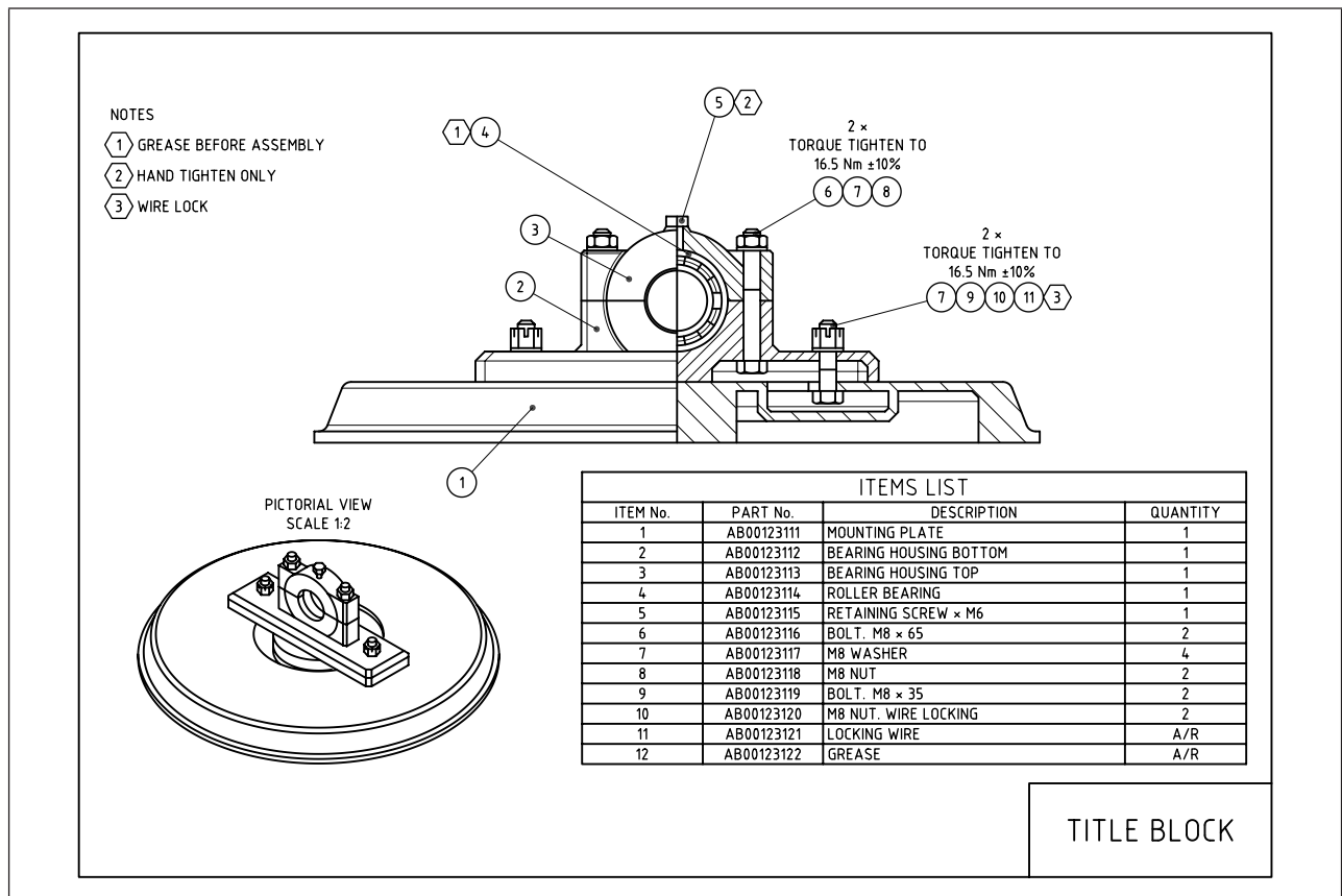
Figure 4 Example of assembly drawing
