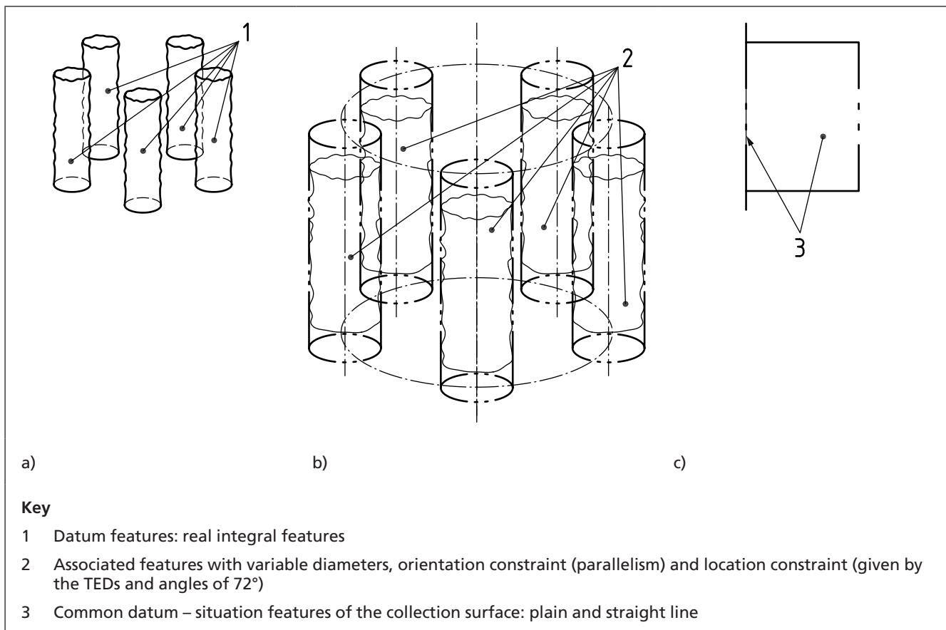
Figure 100 Establishing a common datum from a pattern of five cylinders
