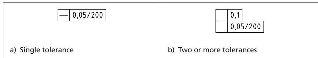
Figure 136 Examples of tolerances of the same characteristic
