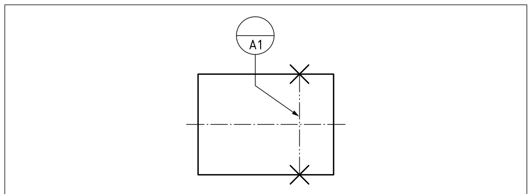
Figure 107 Indicator for single datum target line
