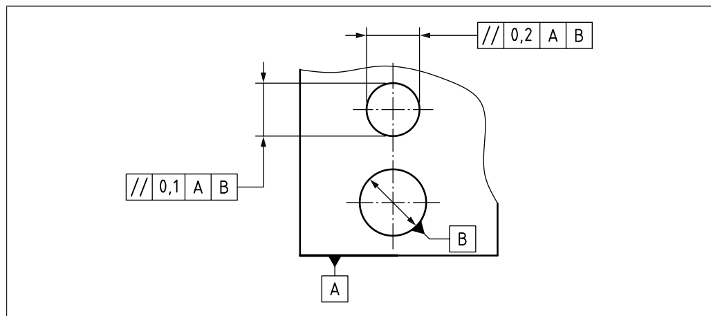
Figure 127 Orientation of the width of an orientation tolerance zone
