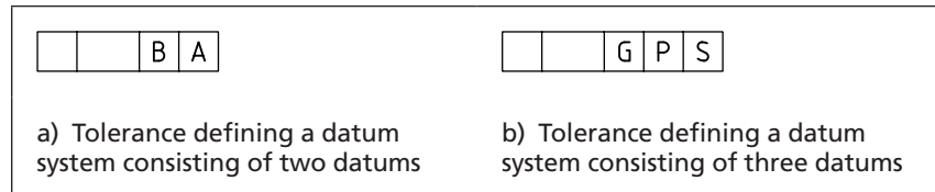
Figure 79 Tolerance defining a datum system
