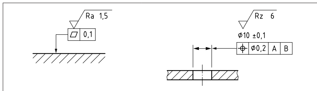
Figure 152 Surface texture requirement: Geometrical tolerance indication
