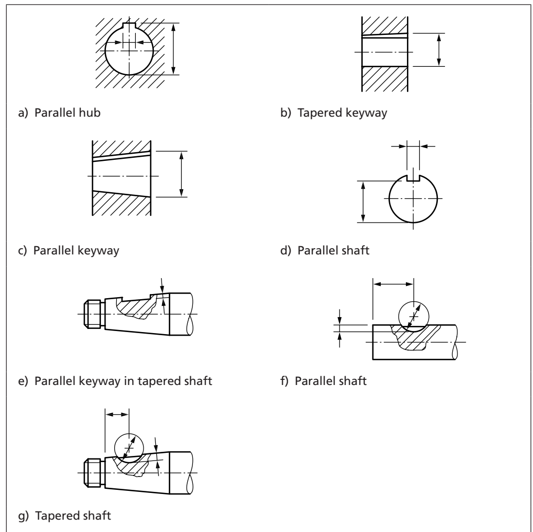
Figure 67 Dimensioning of keyways
