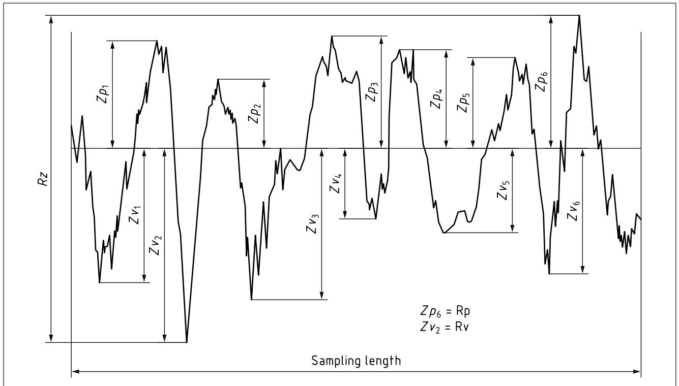
Figure 146 Peak height ( R_p ), valley depth ( R_v ) and maximum height of profile ( R_z )
