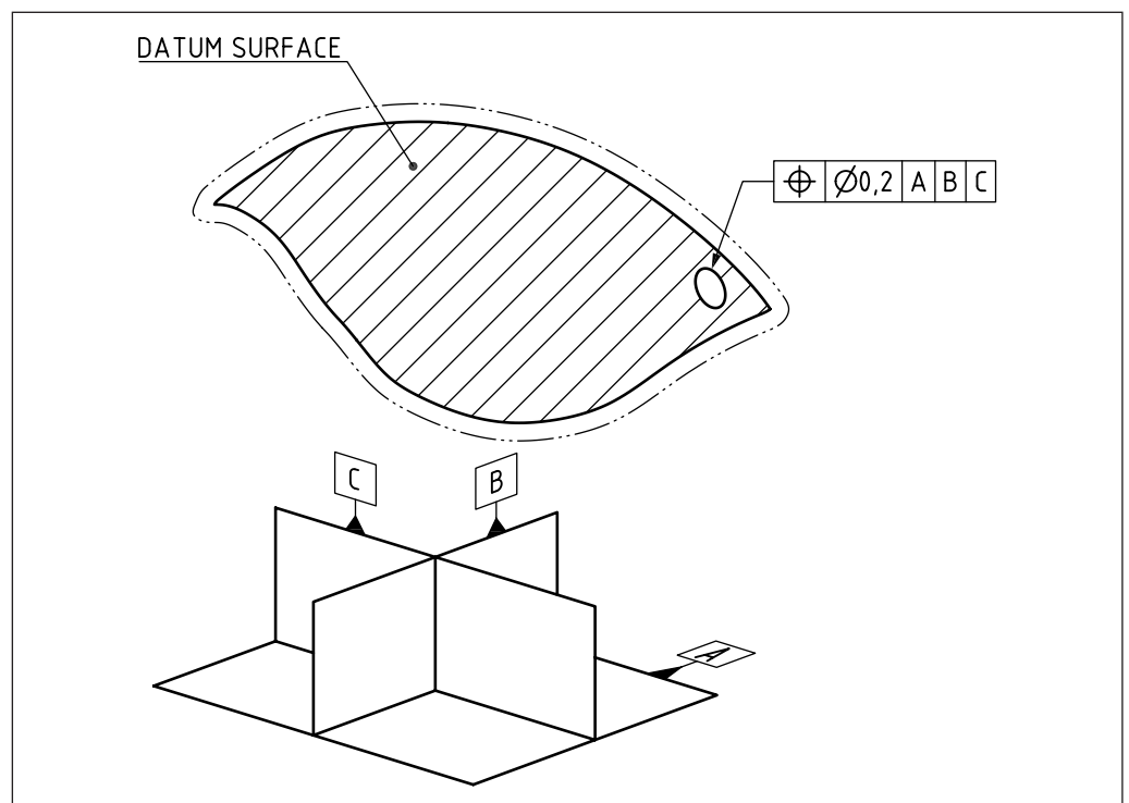
Figure E.2 Implementation according to most CAD software
