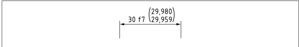
Figure 69 Example: expression of two limits of size to the same number of decimal places
