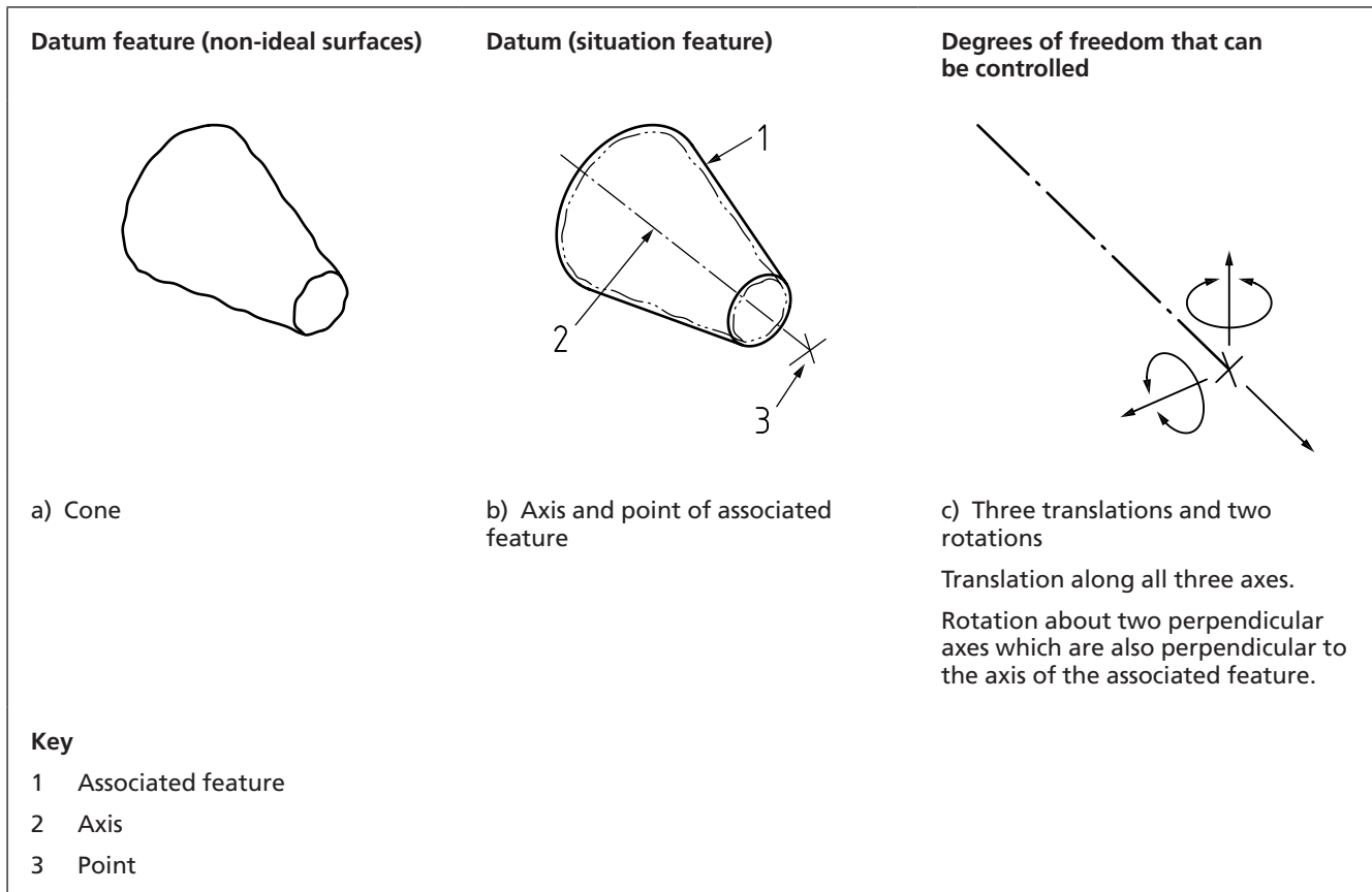
Figure 86 Datum feature consisting of a non-ideal cone
