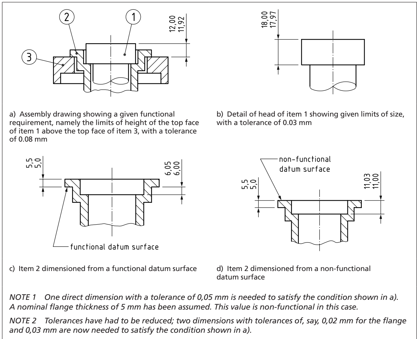
Figure 78 Effect of changing datum surfaces from those determined by functional
