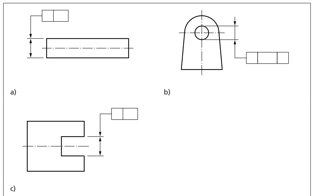
Figure 123 Terminator as an extension of the dimension line
