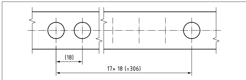
Figure 40 Number of equally-spaced features and the dimensional value
