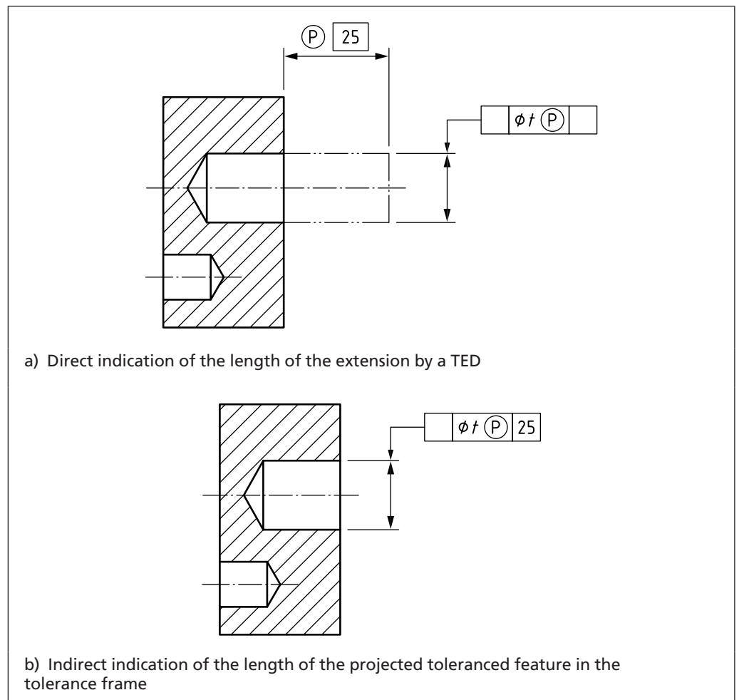
Figure 139 Two ways of indicating a geometrical specification with projected tolerance modifier
