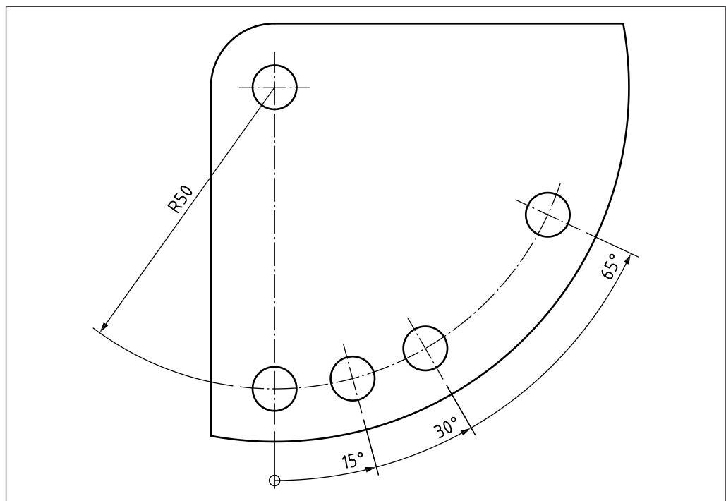
Figure 64 Running dimensioning of angles
