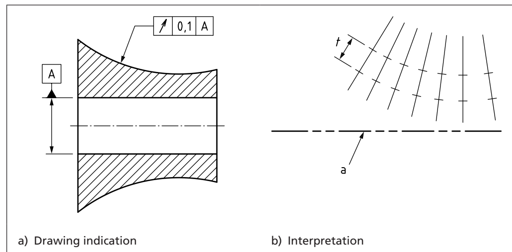
Figure 124 Width of tolerance zone applying to the specified geometry
