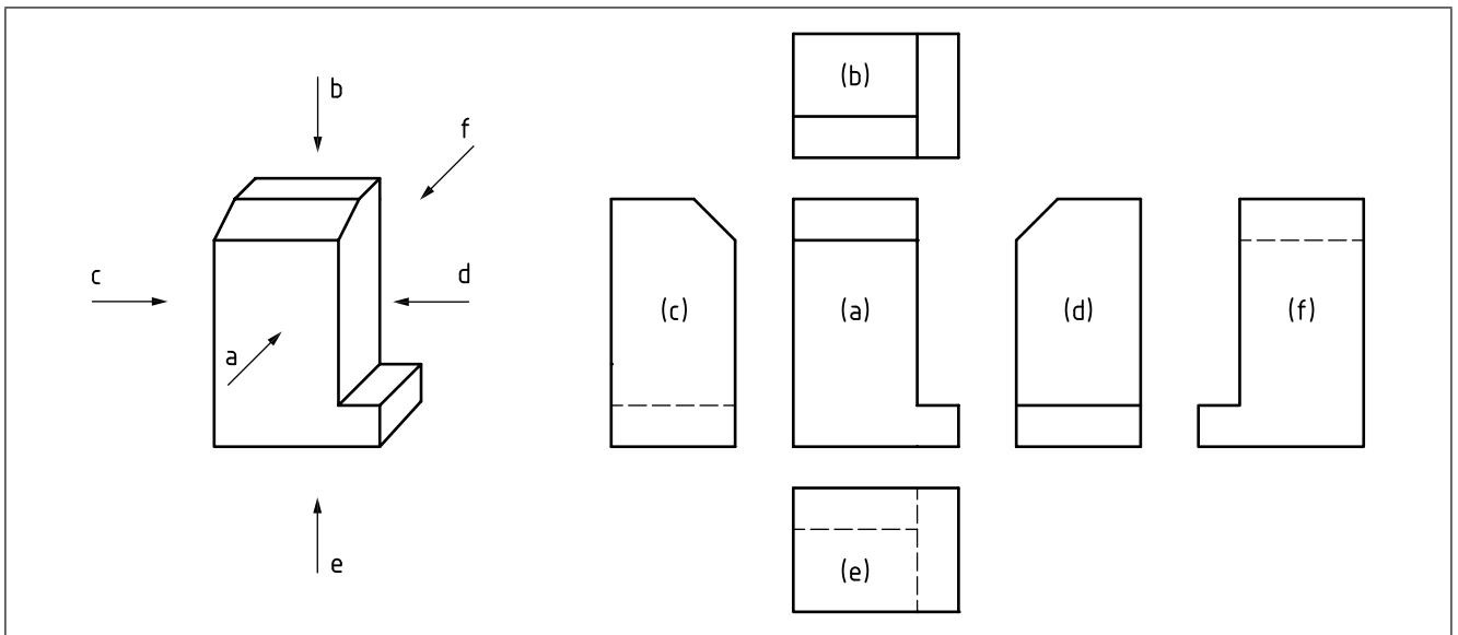
Figure 12 Third angle projection method
