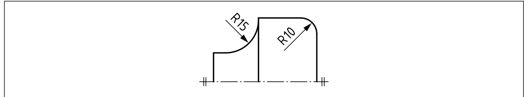
Figure 33 Indications of special dimensions: Radius
