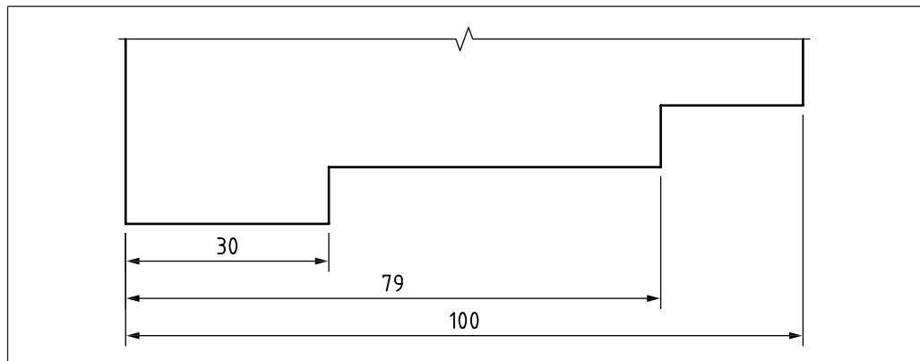
Figure 61 Example of parallel dimensioning
