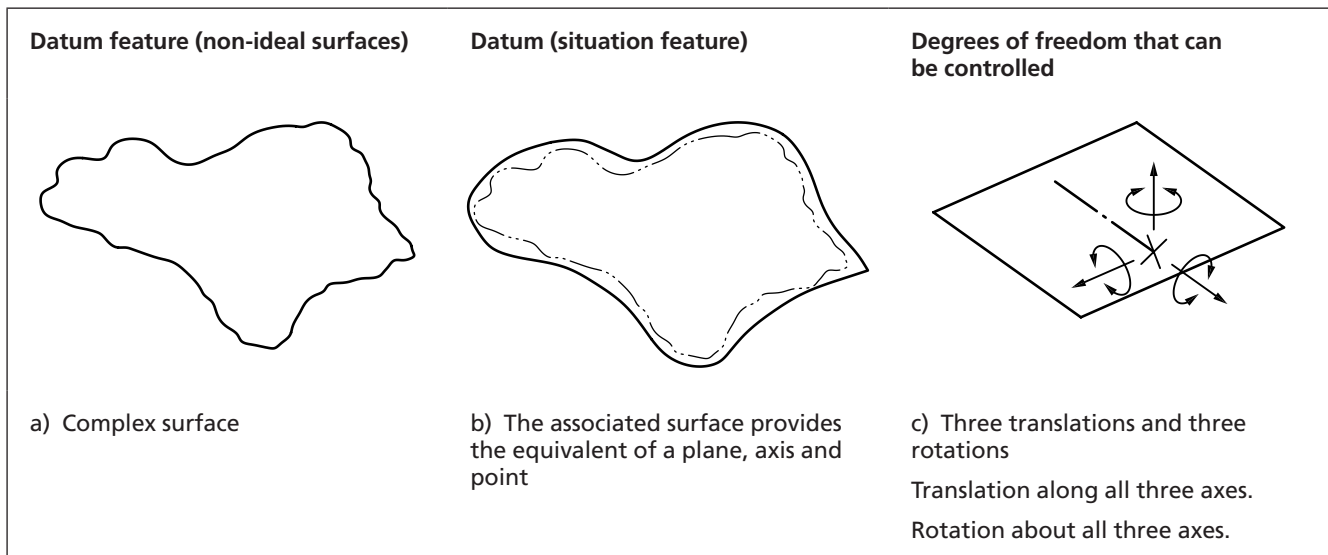
Figure 93 Datum feature consisting of a non-ideal complex surface
