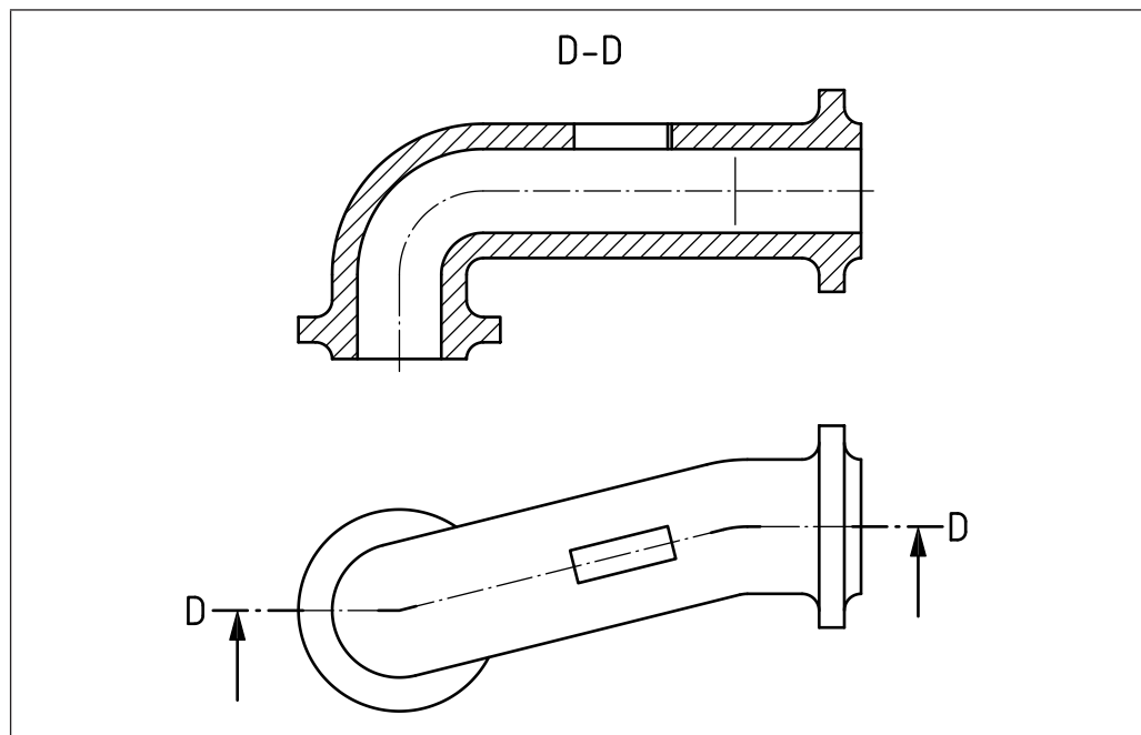
Figure 17 Section view in three contiguous planes showing true shape of inclined surface
