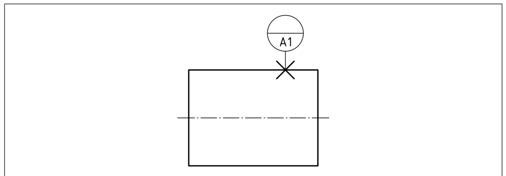
Figure 106 Indicator for single datum target point
