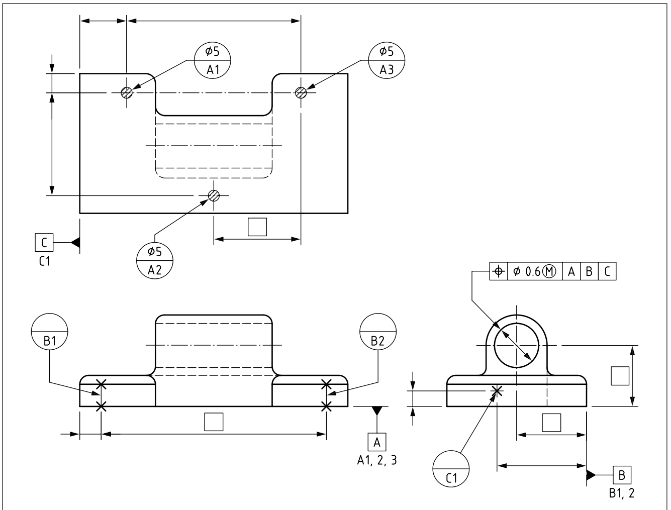
Figure 114 Application of datum targets
