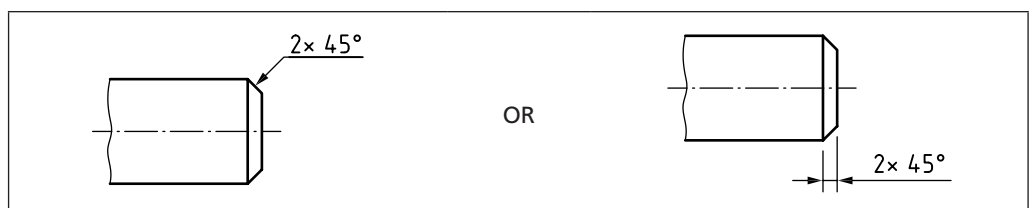
Figure 46 Dimension of external chamfer equal to 45°
