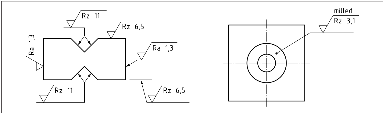
Figure 151 Attachment of surface texture requirement to workpiece
