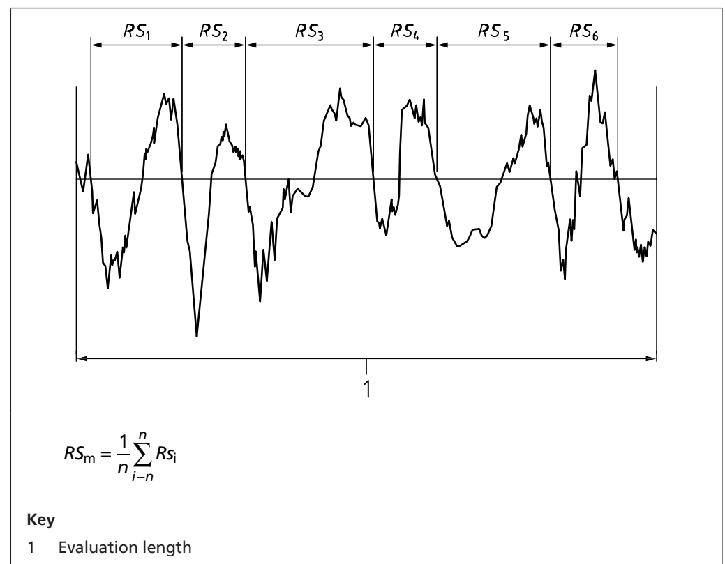
Figure 148 Derivation of mean width of profile element ( RS_m )
