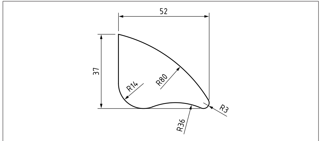
Figure 57 Example of curved feature defined by radii
