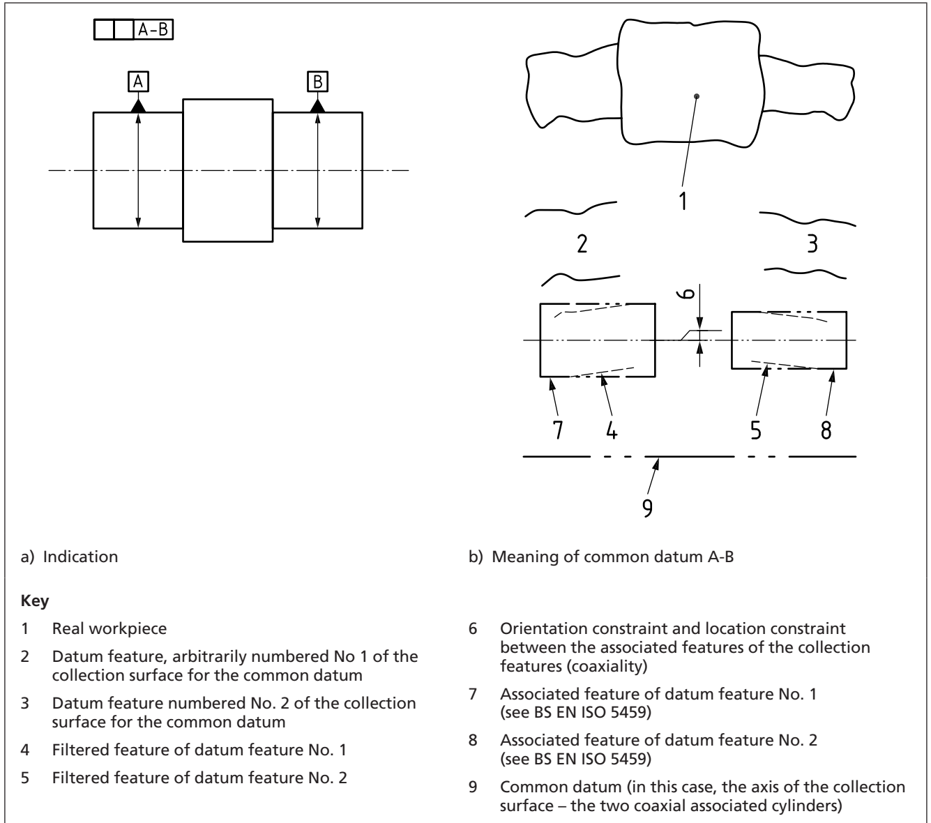
Figure 101 Association for a common datum based on two coaxial cylinders
