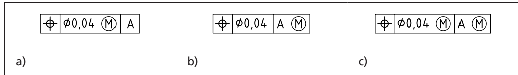
Figure 140 Indication of the maximum material requirement
