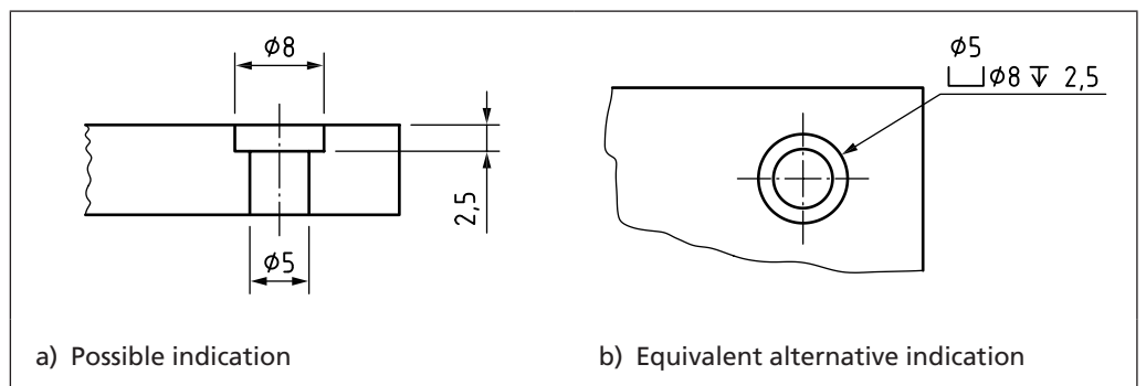
Figure 38 Diameter and depth of counterbore
