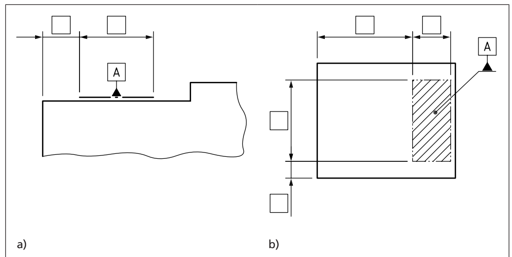
Figure 112 Simplification of drawing indication when there is only one datum target area
