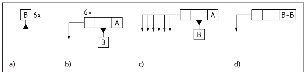
Figure 116 Examples of complementary indication
