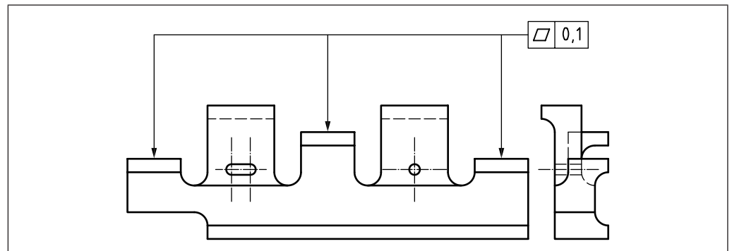
Figure 130 Tolerance zones applied to separate features
