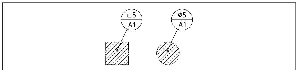
Figure 109 Indicator for single datum target area
