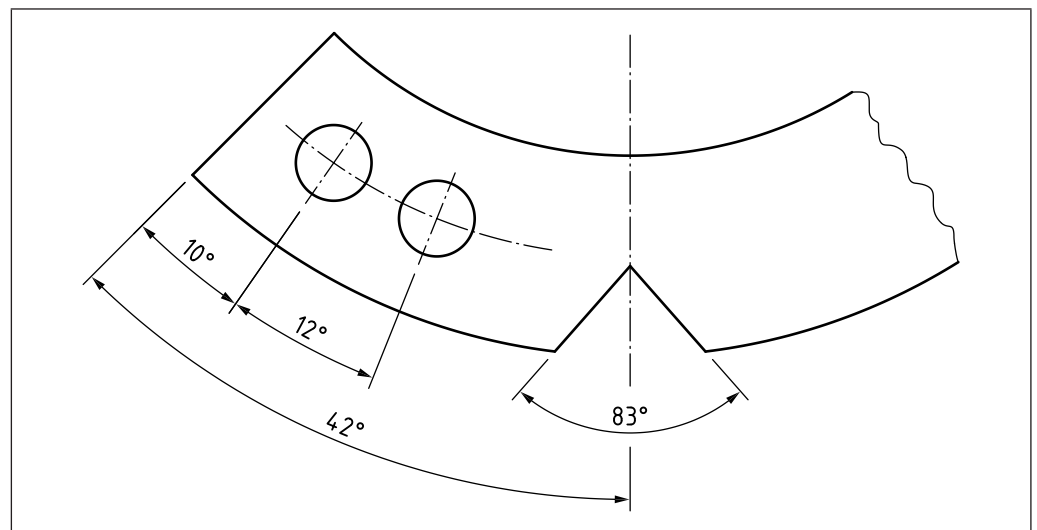
Figure 28 Extension lines of angular dimensions
