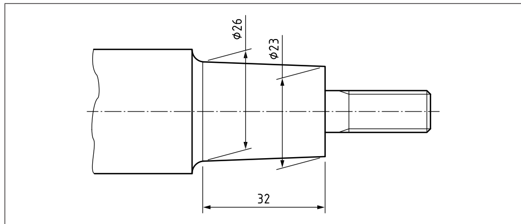
Figure 25 Oblique extension lines
