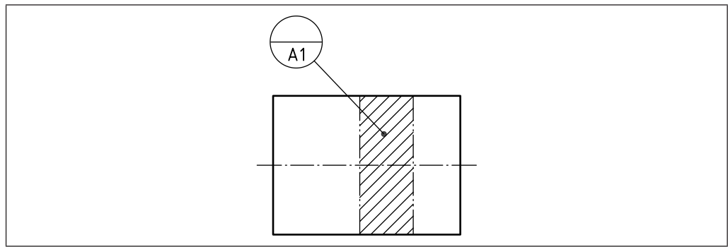
Figure 108 Indicator for single datum target surface
