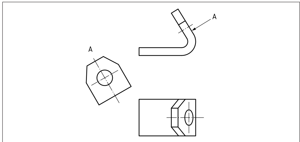
Figure 14 Auxiliary view showing true shape of inclined surface
