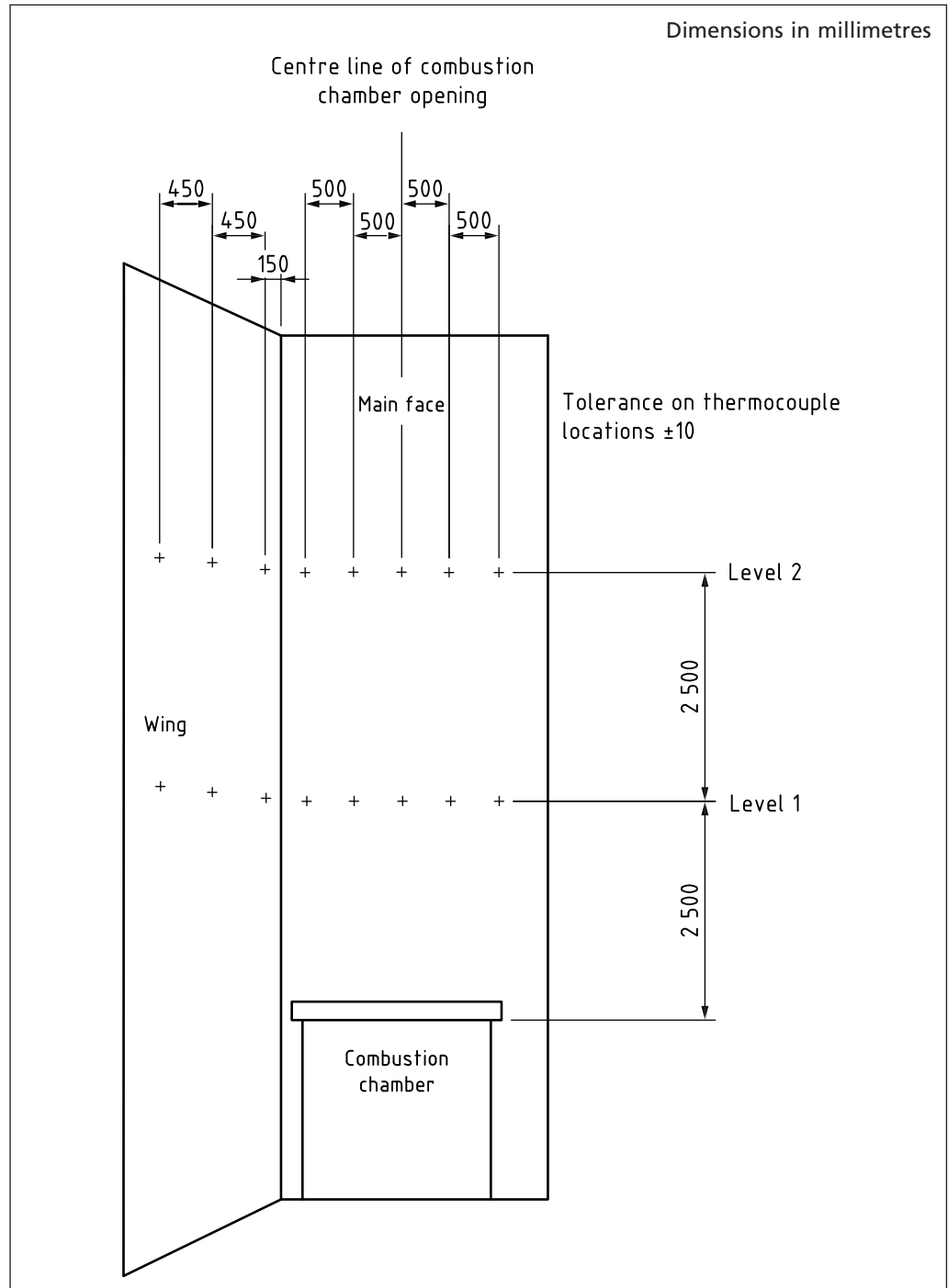
Figure 2 Location of thermocouples for a cladding test
