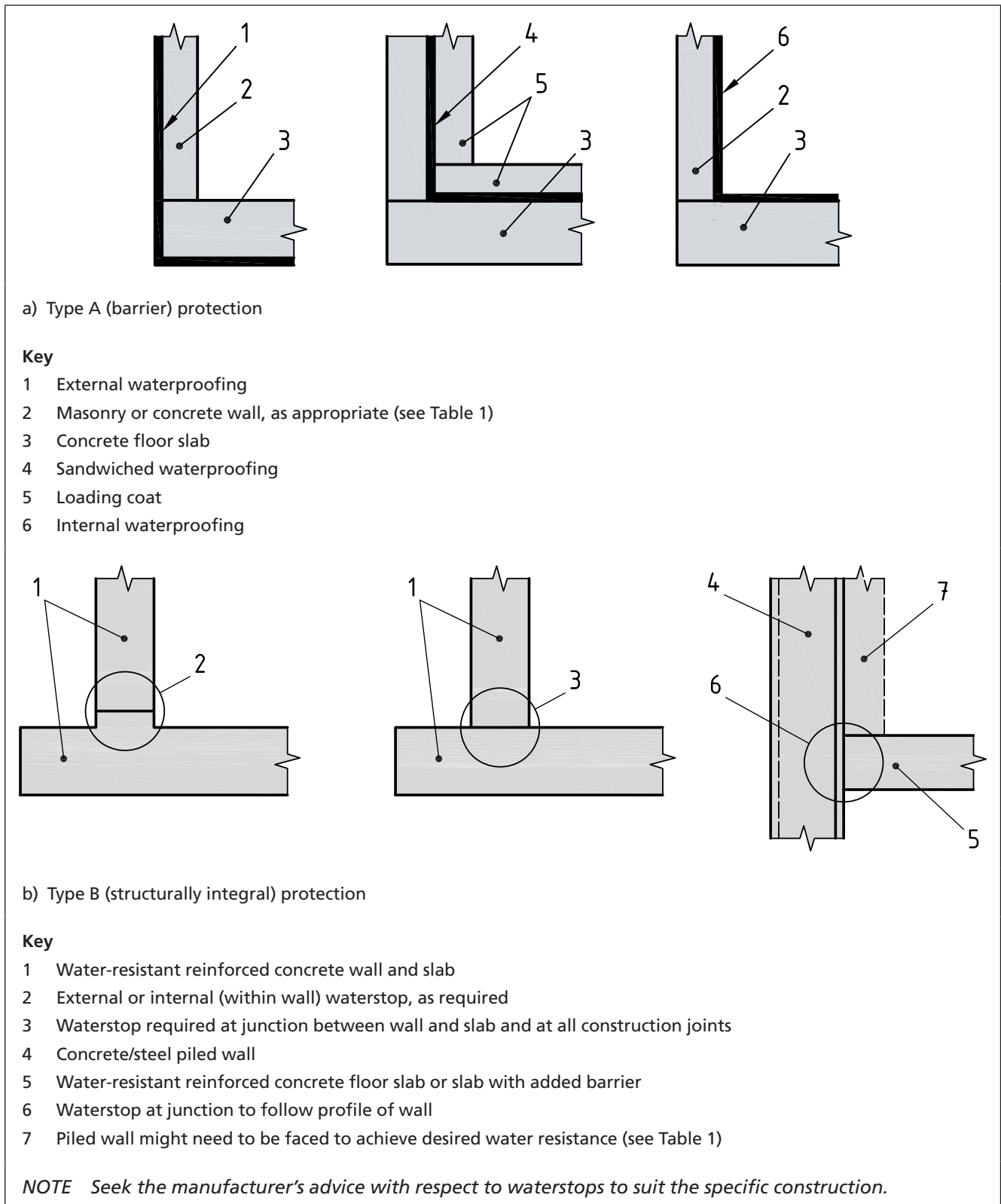
Figure 2 Schematic illustrations of Type A, Type B and Type C waterproofing protection
