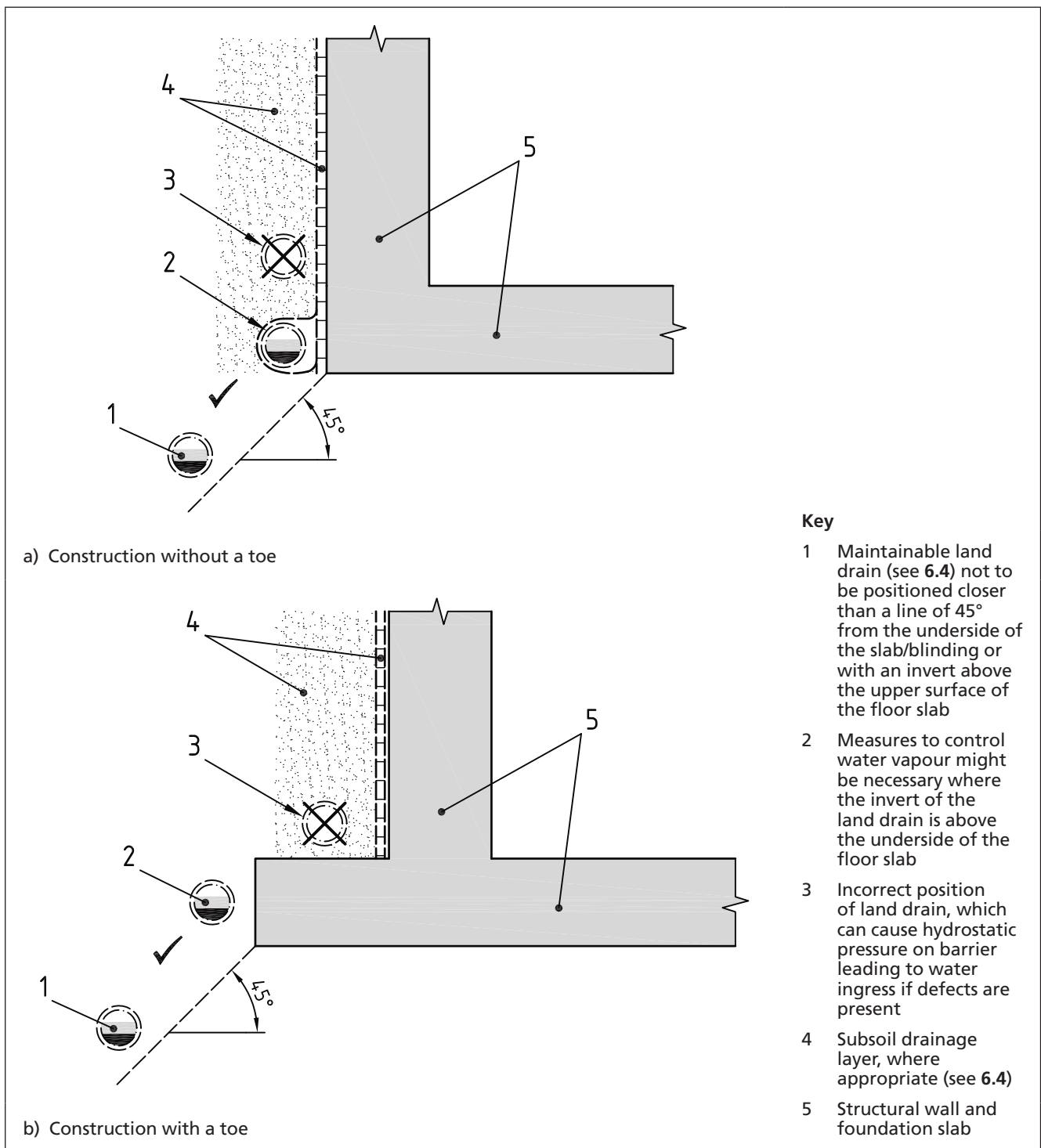
Figure 3 Sub-surface drainage positioning
