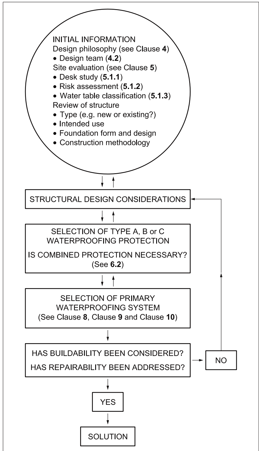
Figure 1 Design flowchart
