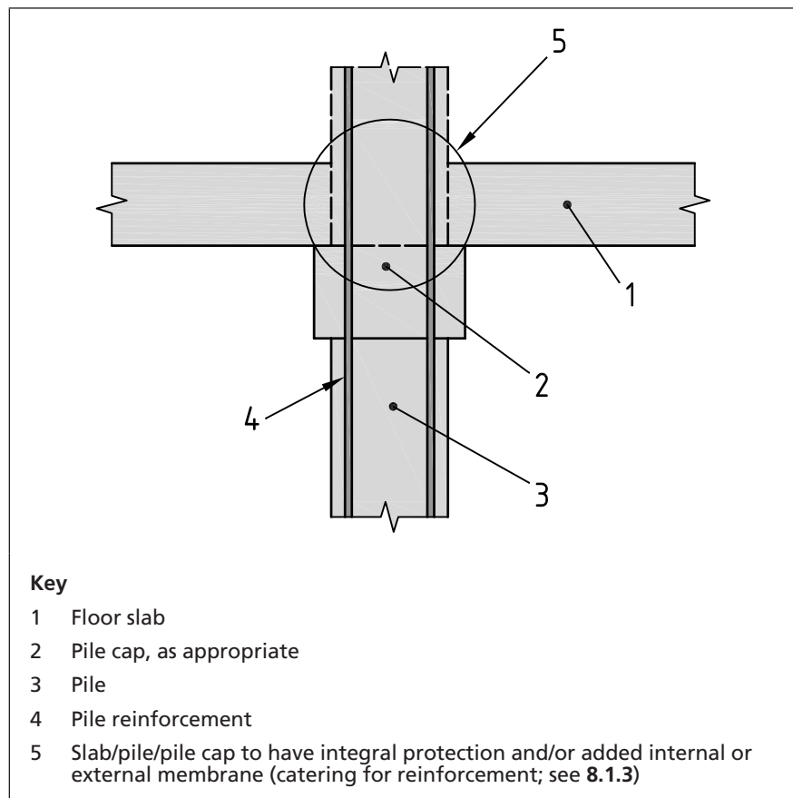
Figure 5 Pile to floor slab junction
