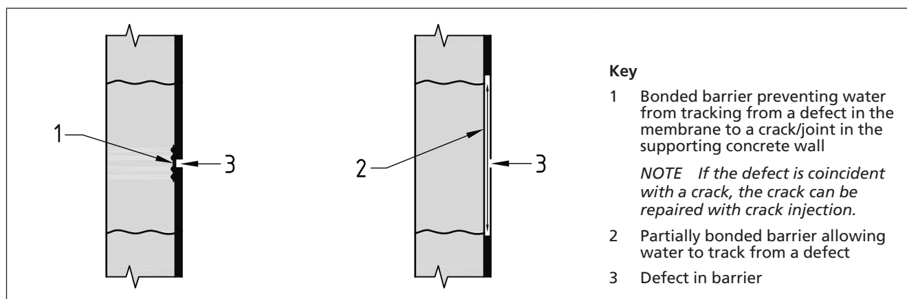
Figure 6 Effect of bonded or partially bonded barriers
