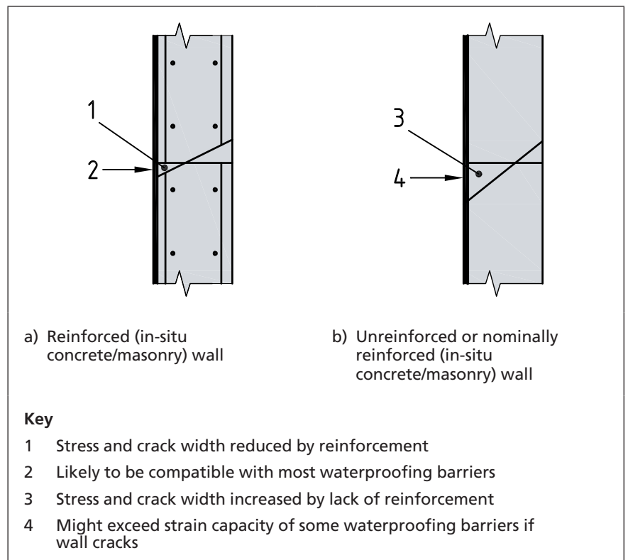
Figure 4 Effect of structure on applied waterproofing barrier
