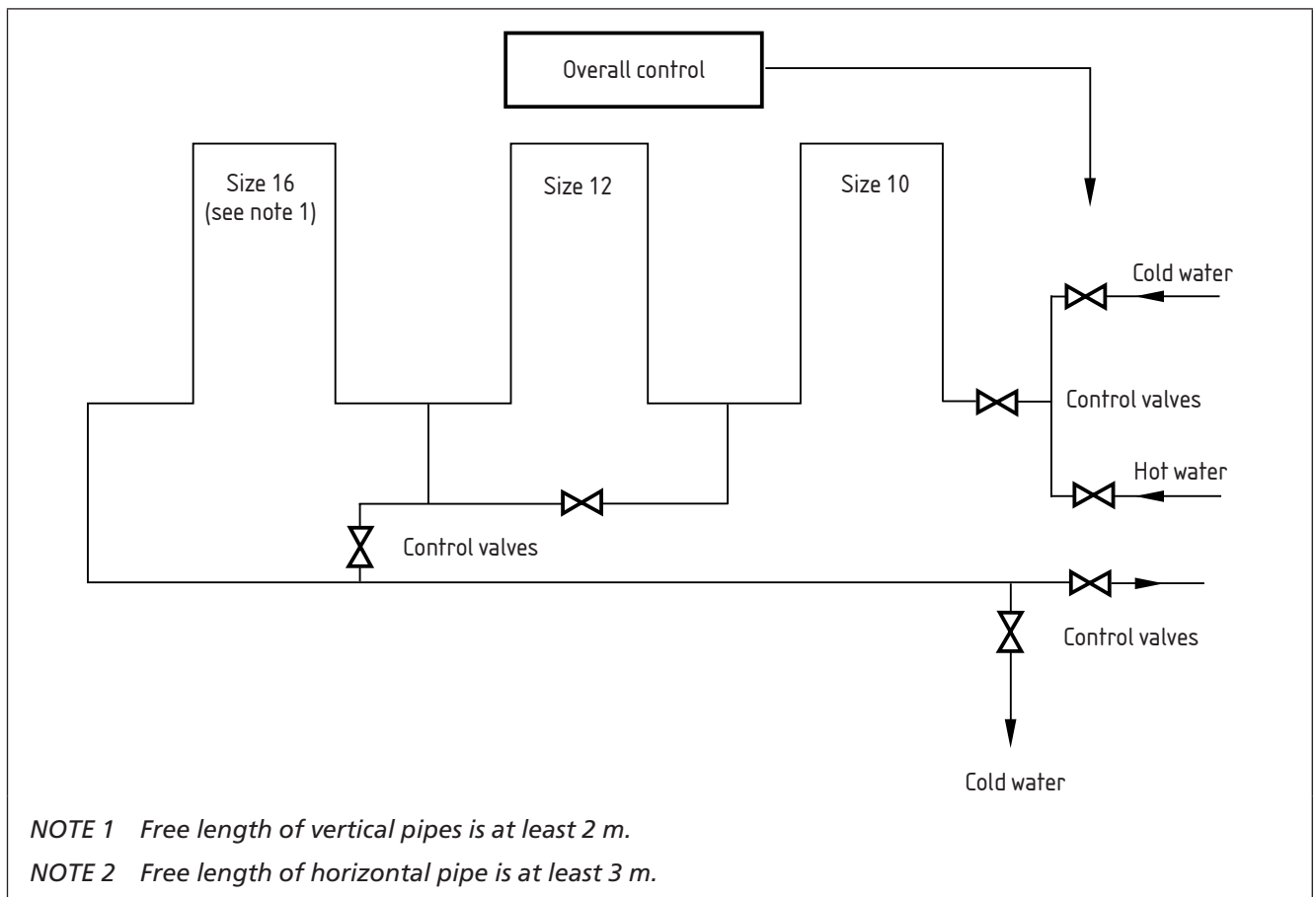
Figure C.1 Test assembly for systems based on rigid pipes
