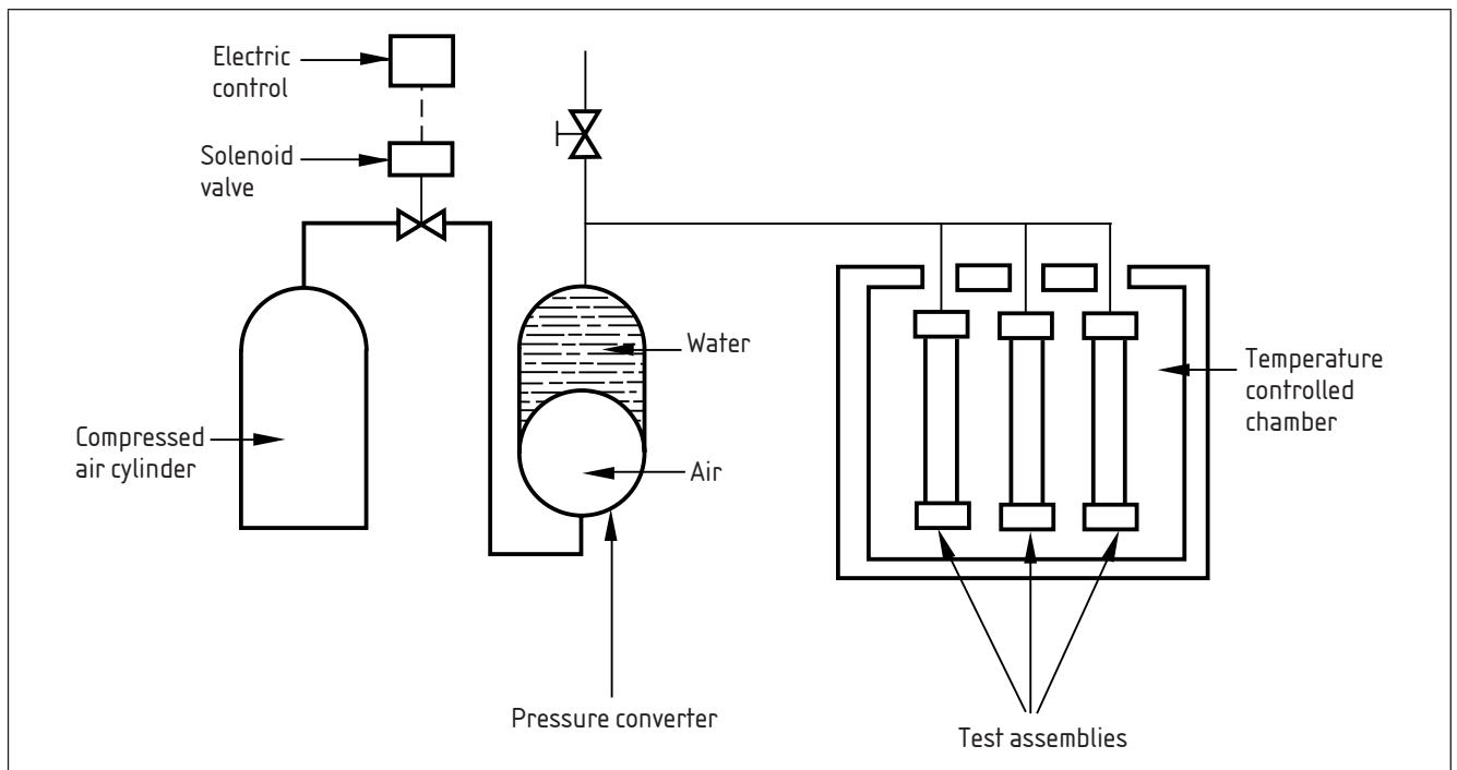
Figure D.1 Diagram of typical equipment arrangement for cyclic pressure shock test
