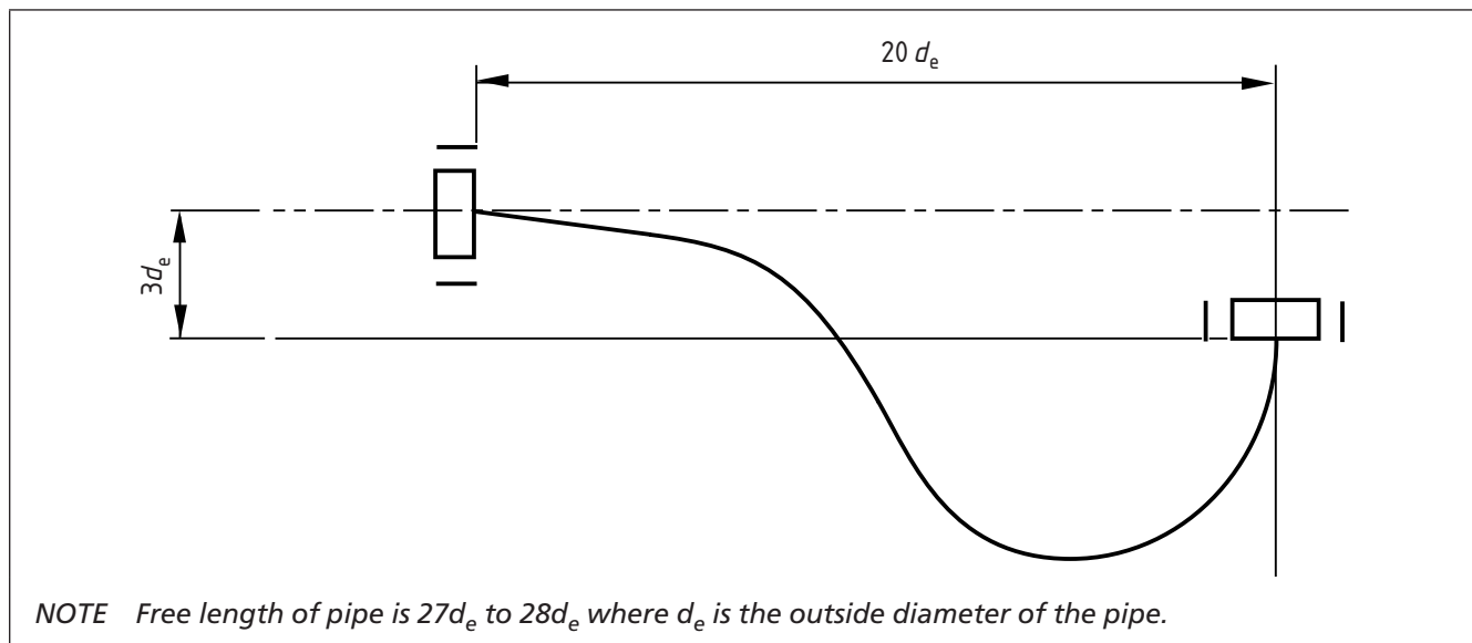
Figure C.3 Configuration of bent flexible pipes for thermal cycle testing
