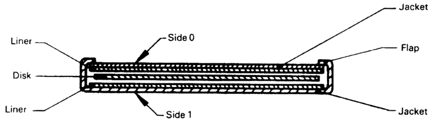
Figure 2 — Section A-A
