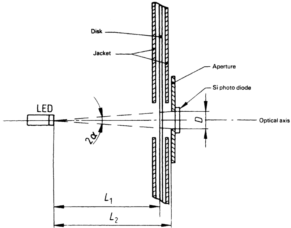
Figure 12 — Measuring device
