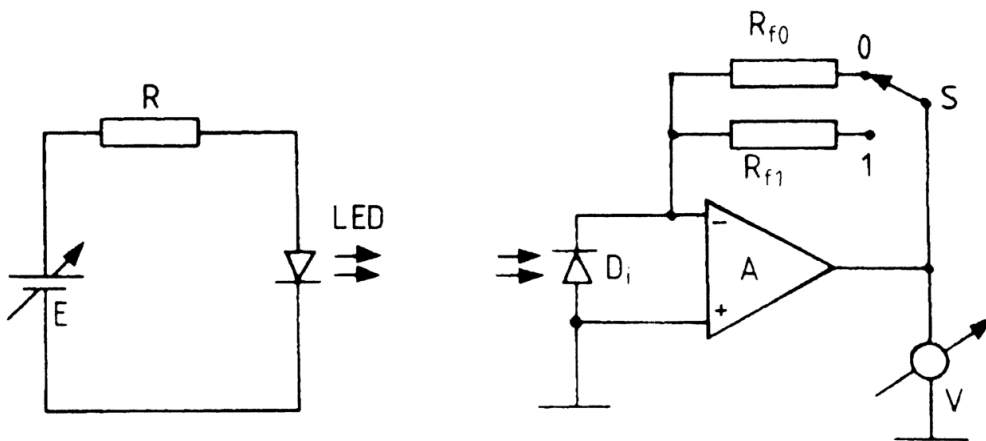
Figure 13 — Electronic circuitry
