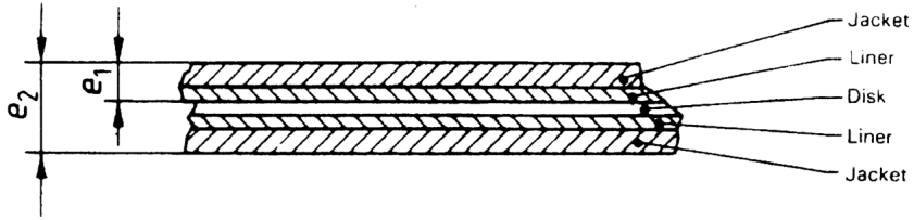
Figure 5 — Cartridge thickness
