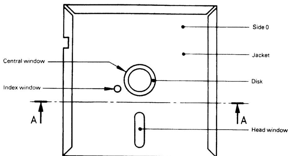
Figure 1 — Flexible disk cartridge
