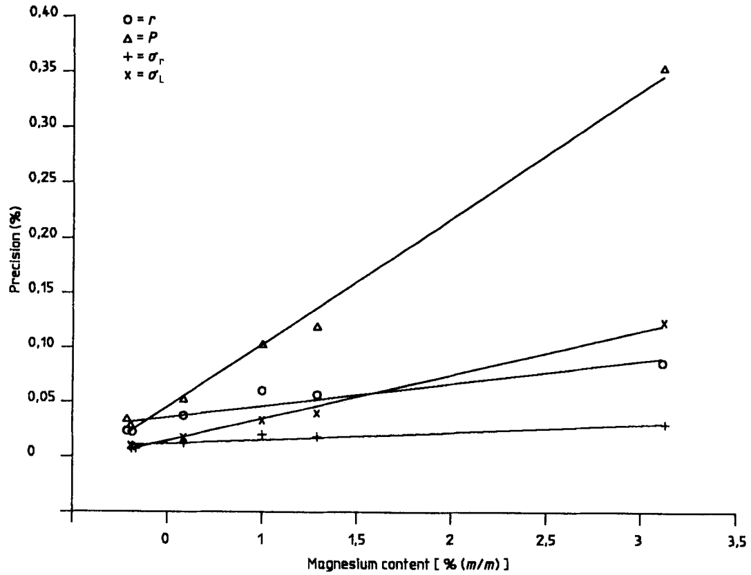
Figure C.1 — Least-squares fit of precision against X for magnesium
