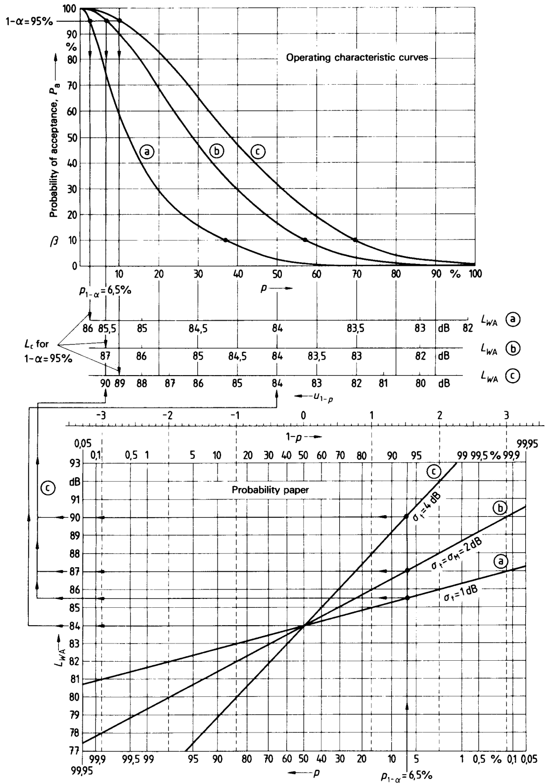
Figure 3 — Change of the operating characteristic curve for \sigma_t \neq \sigma_M
