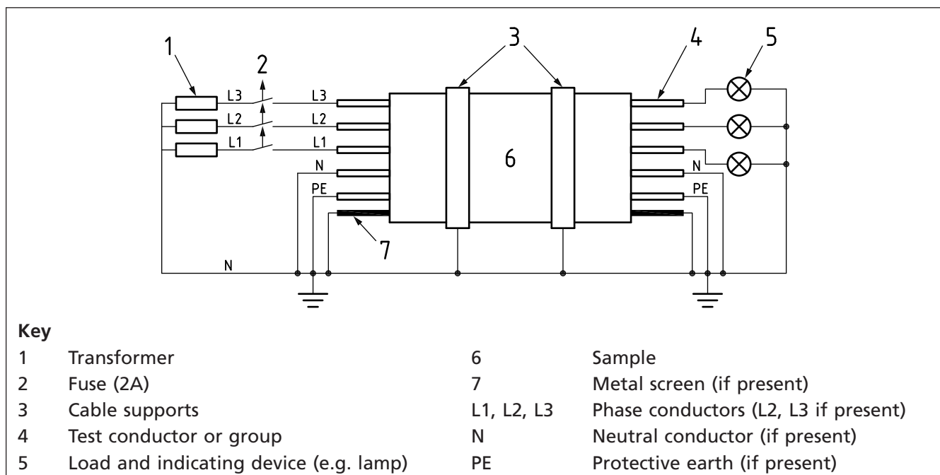
Figure 2 Circuit diagram
