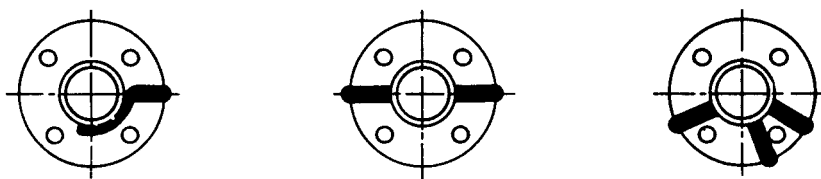
Figure 5 — Routing at flanges to avoid leaks and mechanical damage
