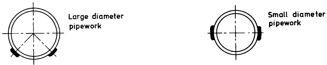
Figure 3 — Double run of heating tape straight traced on pipework without fittings
