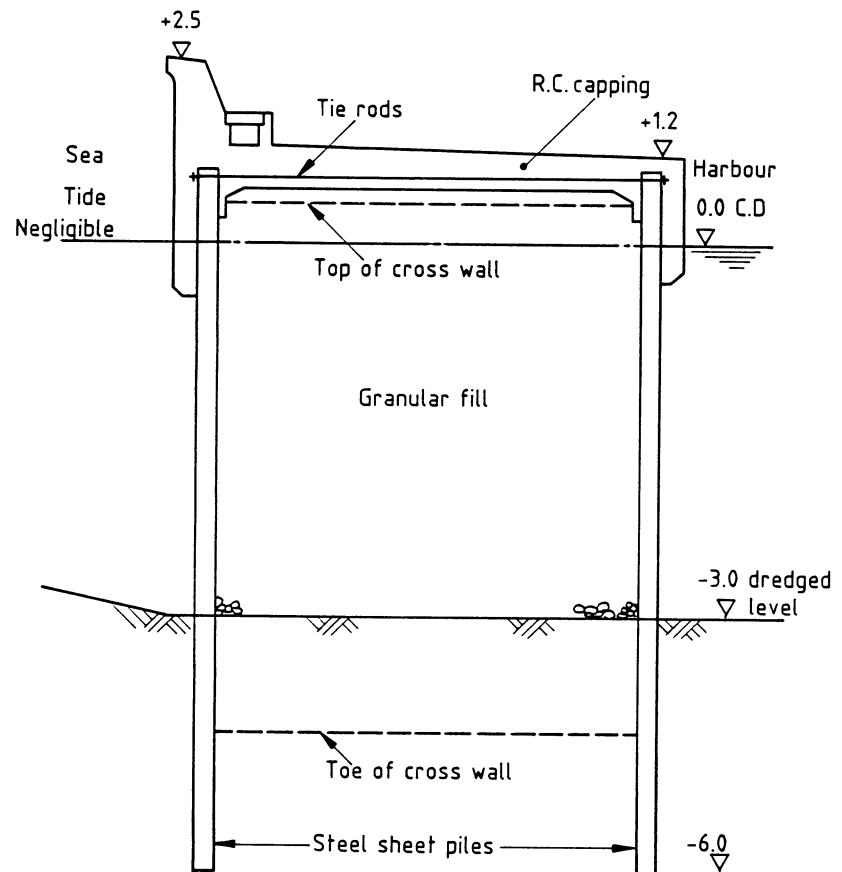
Figure 22 — Double-wall sheet piled structure
